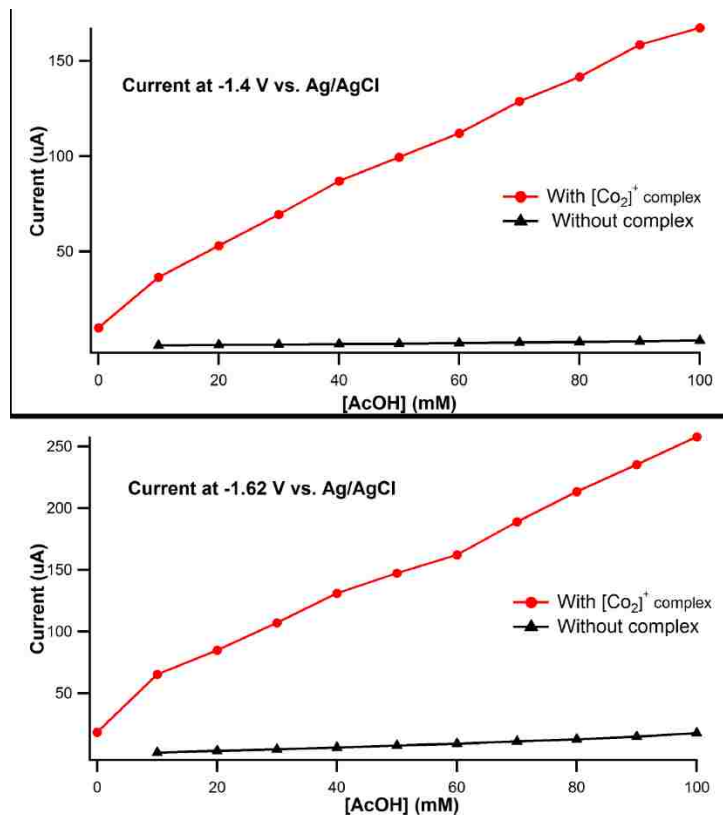
Figure 7.6 Red dots: CV current at -1.4 V (top) and -1.62 V (bottom) as a function of [AcOH] for solutions of [\text{Co}_2(\text{L}^{\text{N}3\text{O}2})(\text{bpy})_2]\text{ClO}_4 ( 15 ) (2.0 mM) in \text{CH}_3\text{CN} . Black triangles: The corresponding data measured under identical conditions but in the absence of complex 15 . All results were obtained using an amalgamated gold working electrode in \text{CH}_3\text{CN} solutions with 0.1 M (\text{NBu}_4)\text{PF}_6 as the supporting electrolyte.
