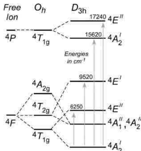
Figure 4.5 Energy level diagram indicating the ligand-field states for a high-spin d7 ion in three coordination environments: free ion, octahedral (O h ), and trigonal–bipyramidal (D 3h ). The experimentally-determined transition energies for the Co II ion in NiCo OAc are provided in wavenumbers (cm -1 ). Partially adapted from reference 162 .
