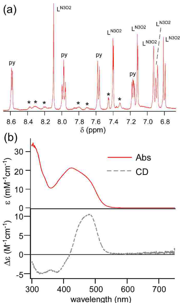
Figure 5.8 Top : Aromatic region of the ^1\text{H} NMR spectrum of complex 17 in \text{MeCN-}d_3 . The peaks are assigned to either the pyridyl (py) moiety of S - i\text{PrOxPy} or the \text{L}^{\text{N}3\text{O}2} ligand based on splitting patterns and comparison to data collected for \text{H}_3\text{L}^{\text{N}3\text{O}2} and 14 . Each of the 10 assigned features integrates to two H-atoms. The ill-defined peaks marked with asterisks arise from the minor diastereomeric product. Bottom : Absorption and CD spectra of 17 collected at room temperature in MeCN.
