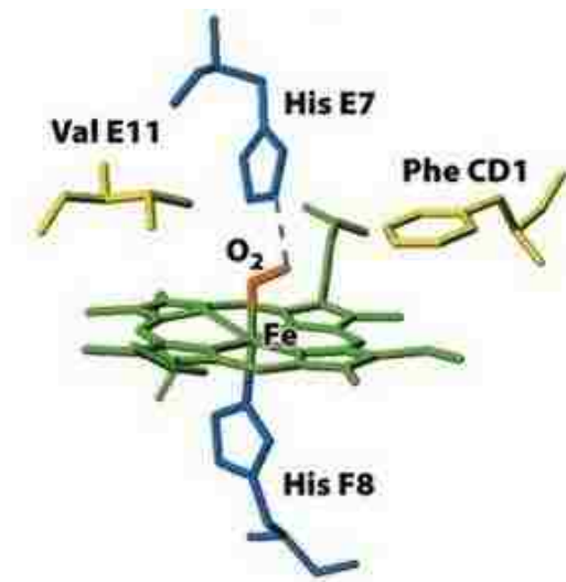
Figure 1.2 Active site structure of oxy-myoglobin. 16
