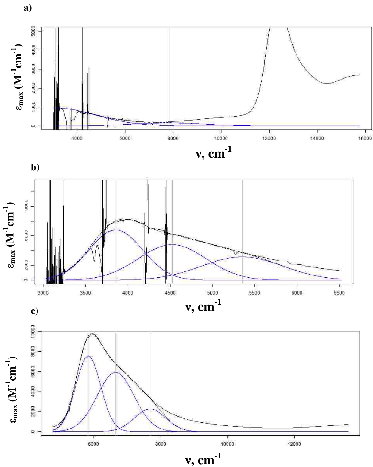
Figure 3.11. IVCT band shape fitting: a) [1](\text{BF}_3)_2 , b) [2](\text{PF}_6)(\text{BF}_4) , c) [3](\text{PF}_6)(\text{BF}_4) .
