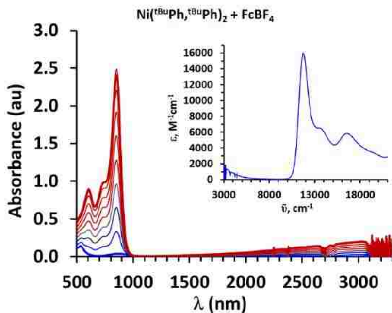
Figure 2.26. Vis-NIR spectra from incremental addition of \text{FcBF}_4 to solution of \text{Ni}(\text{tBuPh}, \text{tBuPh})_2 in \text{CH}_2\text{Cl}_2 . Inset: Spectra of \text{Ni}(\text{tBuPh}, \text{tBuPh})_2(\text{BF}_4) in wavenumber units.
