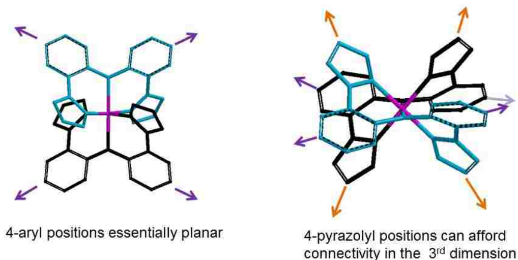
Figure 5.5. View of a model \text{Ni}(\text{X},\text{Y})_2 complex showing relative disposition of para-aryl and 4-pyrazolyl groups.
