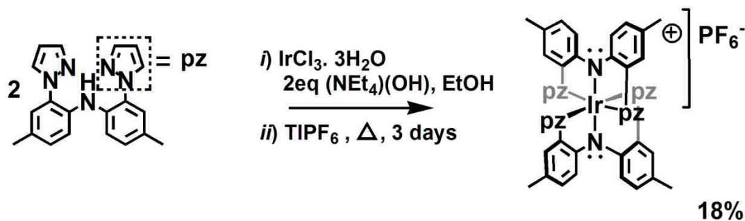
Scheme 3.3. Preparation of \text{Ir}(\text{Me},\text{Me})_2\text{PF}_6 , [\mathbf{3}](\text{PF}_6) complex.
