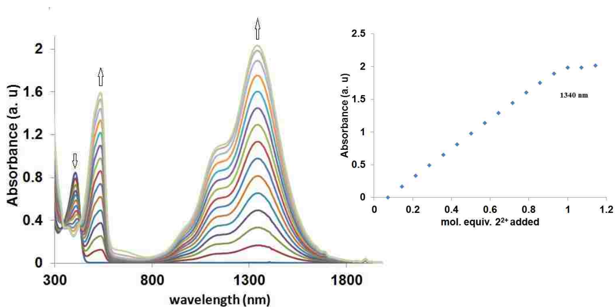
Figure 4.12. Spectrophotometric titration of 2 with 2 2+ in CH 2 Cl 2 . Inset: Absorbance vs mol. equi. of 2 2+ added at 1340 nm.
