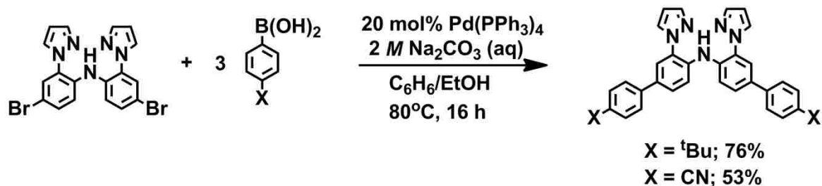
Scheme 2.4. Preparation of \text{H}(\text{tBuPh}, \text{tBuPh}) and \text{H}(\text{CNPh}, \text{CNPh}) by Suzuki reactions.
