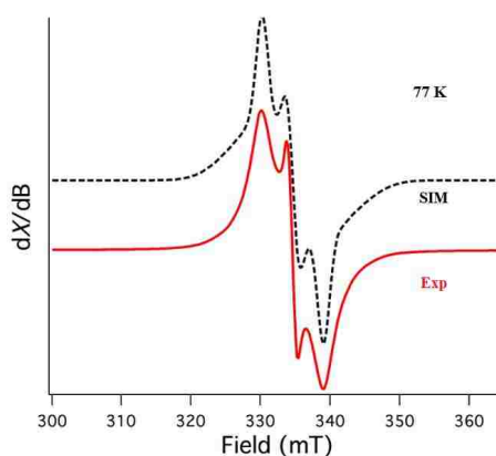
Figure 3.13. X-band (9.39 GHz) EPR spectrum of [ 1 ](BF 4 ) 2 in CH 2 Cl 2 at 77 K.
