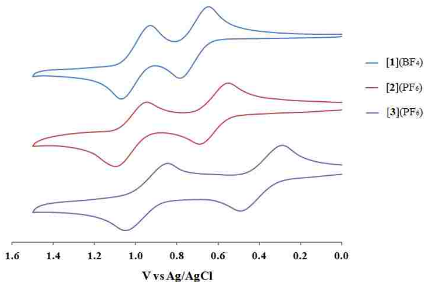
Figure 3.3. Overlay of cyclic voltammograms (CVs) of dichloromethane solutions of each metal complexes, [1] (BF 4 ), [2] (PF 6 ), and [3] (PF 6 ) at a scan rate of 100 mV/s. [N(Bu) 4 ](PF 6 ) was used as the supporting electrolyte.
