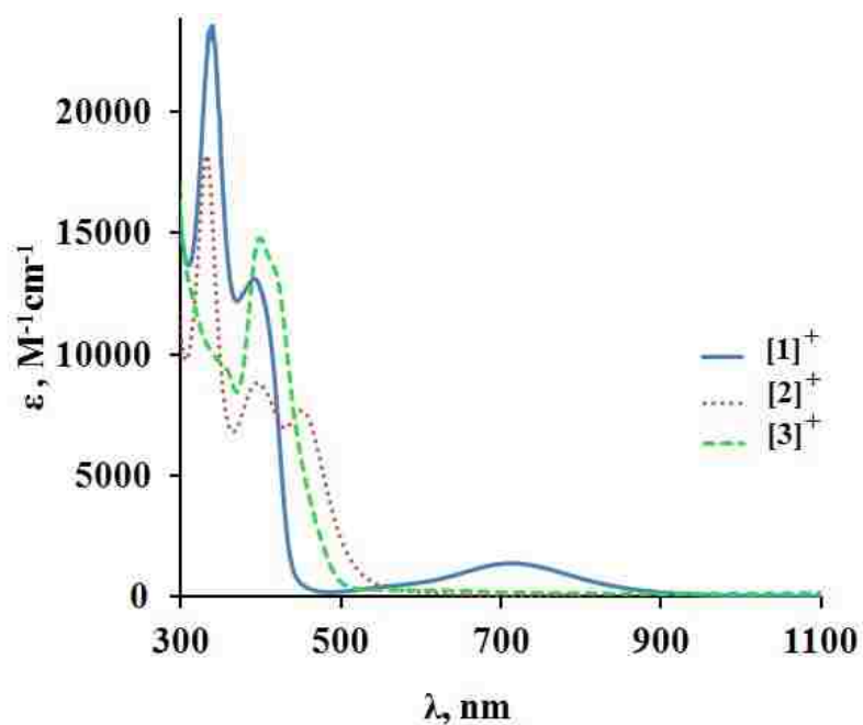
Figure 3.5. UV-vis-near IR spectrum of [1](BF_4) (blue), [2](PF_6) (red-dotted), and, [3](PF_6) (green-dashed) in CH_2Cl_2 .
