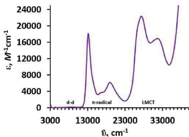
Figure 2.22. Visible/NIR spectrum of [\text{Ni}(\text{Me},\text{Me})_2](\text{BF}_4)_2 \cdot 0.5\text{CH}_2\text{Cl}_2 in \text{CH}_2\text{Cl}_2 .
