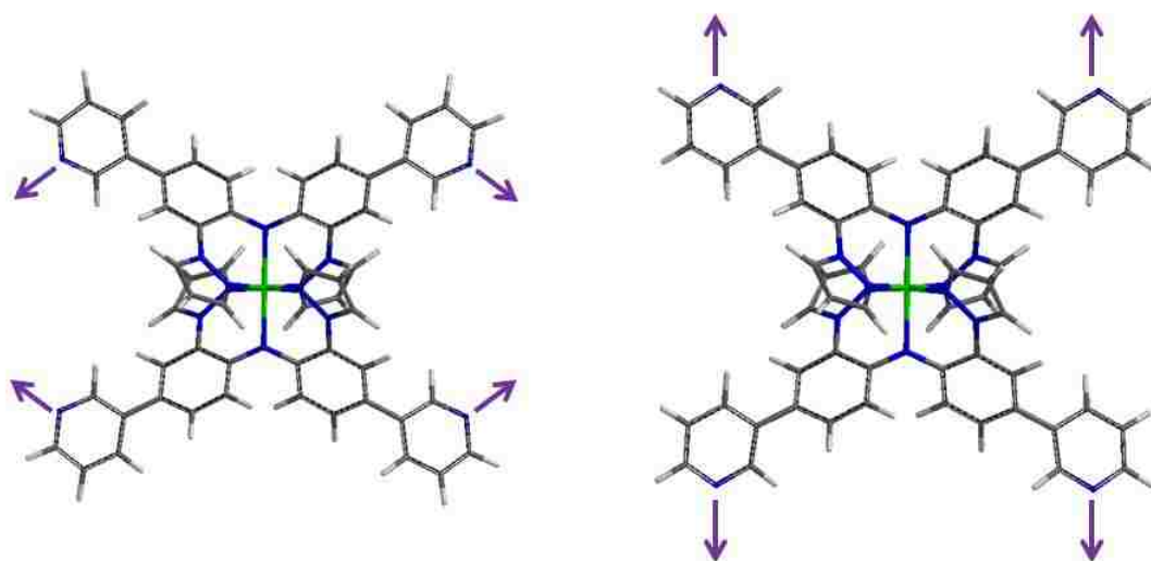
Figure 5.6. Two possible conformers of \text{Ni}(3\text{py},3\text{py})_2 illustrating potential connectivity patterns.
