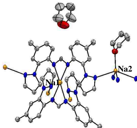
Figure 6.6. Asymmetric unit of the structure of 1 .
