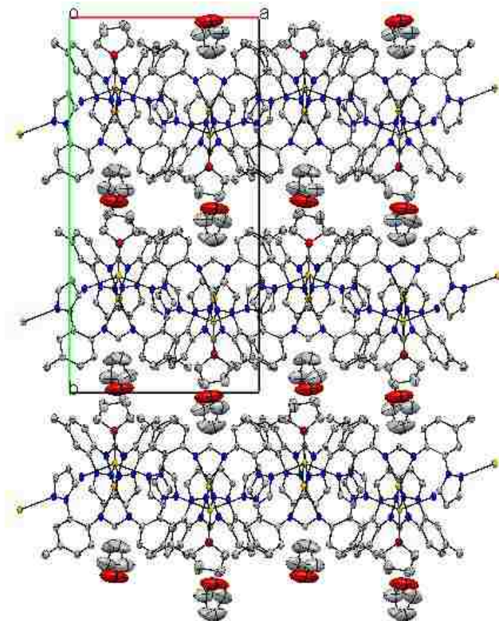
Figure 6.7. Crystal packing of 1 .
