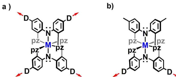
Figure 5.1. Metal containing building blocks with divergent lewis donors.
