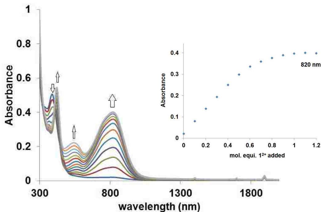
Figure 4.11. Spectrophotometric titration of 1 with 1 2+ in CH 2 Cl 2 . Inset: Absorbance vs mol. equi. of 1 2+ added at 820 nm.
