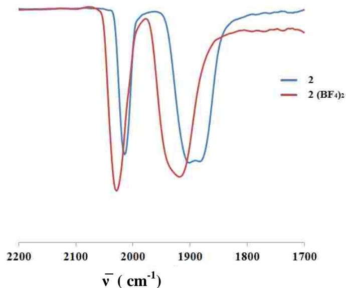
Figure 4.6. IR spectra of 2 and 2·(BF 4 ) 2 .
