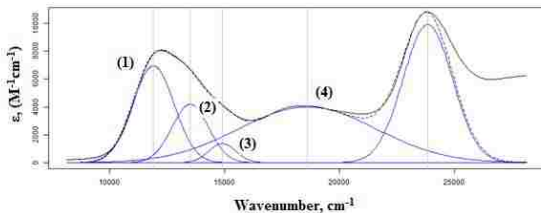
Figure 4.15. Deconvolution of IVCT band of 1 (BF 4 ). Parameters for curve fitting: ( \lambda_{\max} (cm -1 ), \Delta\nu_{1/2} (cm -1 ), \epsilon (M -1 cm -1 ): Curve 1 (11900, 900, 6938), Curve 2(13570, 882, 4180), Curve 3(15000, 600, 1000), Curve 4(18542, 2839, 3970).
