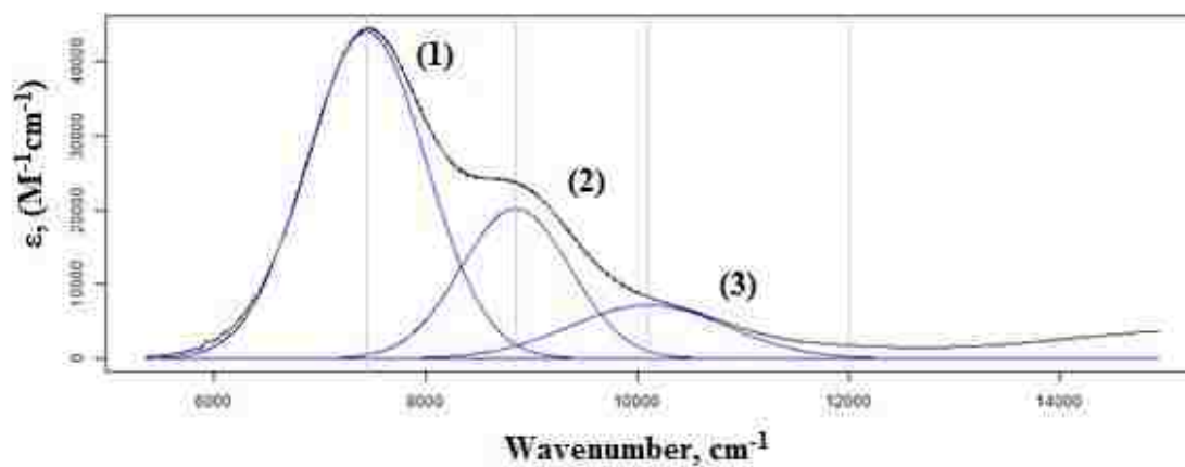
Figure 4.16. Deconvolution of IVCT band of 2 (BF 4 ). Parameters for curve fitting: ( \lambda_{\max} (cm -1 ), \Delta\nu_{1/2} (cm -1 ), \epsilon (M -1 cm -1 ): Curve 1 (7442, 563, 43904), Curve 2( 8901, 560, 20735), Curve 3 (10290, 917, 5269).
