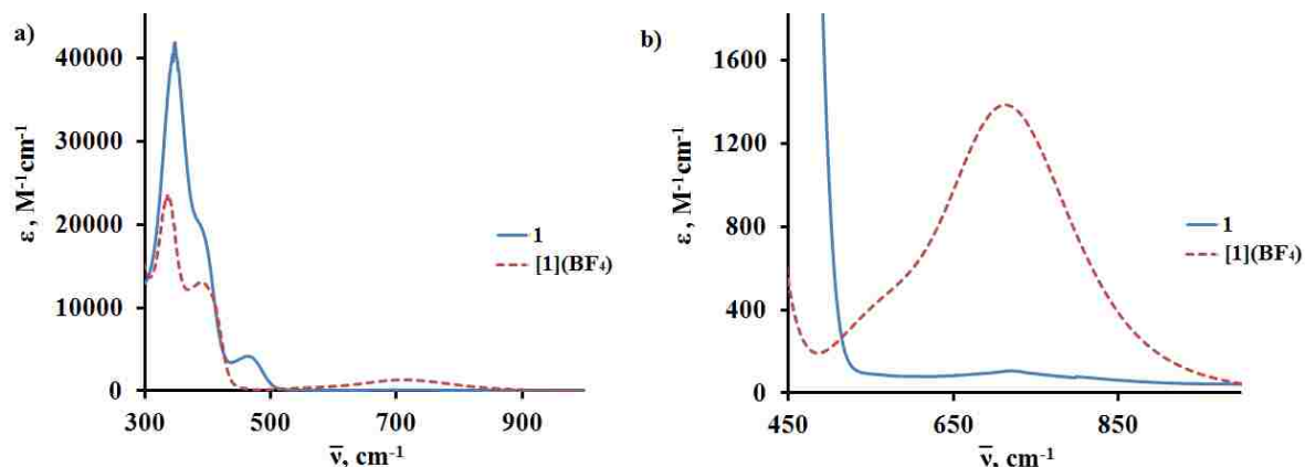
Figure 3.4. a) UV-Visible spectra of 1 and [\mathbf{1}](\text{BF}_4) in \text{CH}_2\text{Cl}_2 . b) Visible region of 1 and [\mathbf{1}](\text{BF}_4) in \text{CH}_2\text{Cl}_2 .
