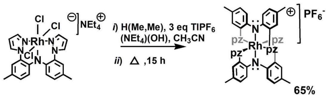
Scheme 3.2. Preparation of \text{Rh}(\text{Me},\text{Me})_2\text{PF}_6 , [\text{2}](\text{PF}_6) complex.
