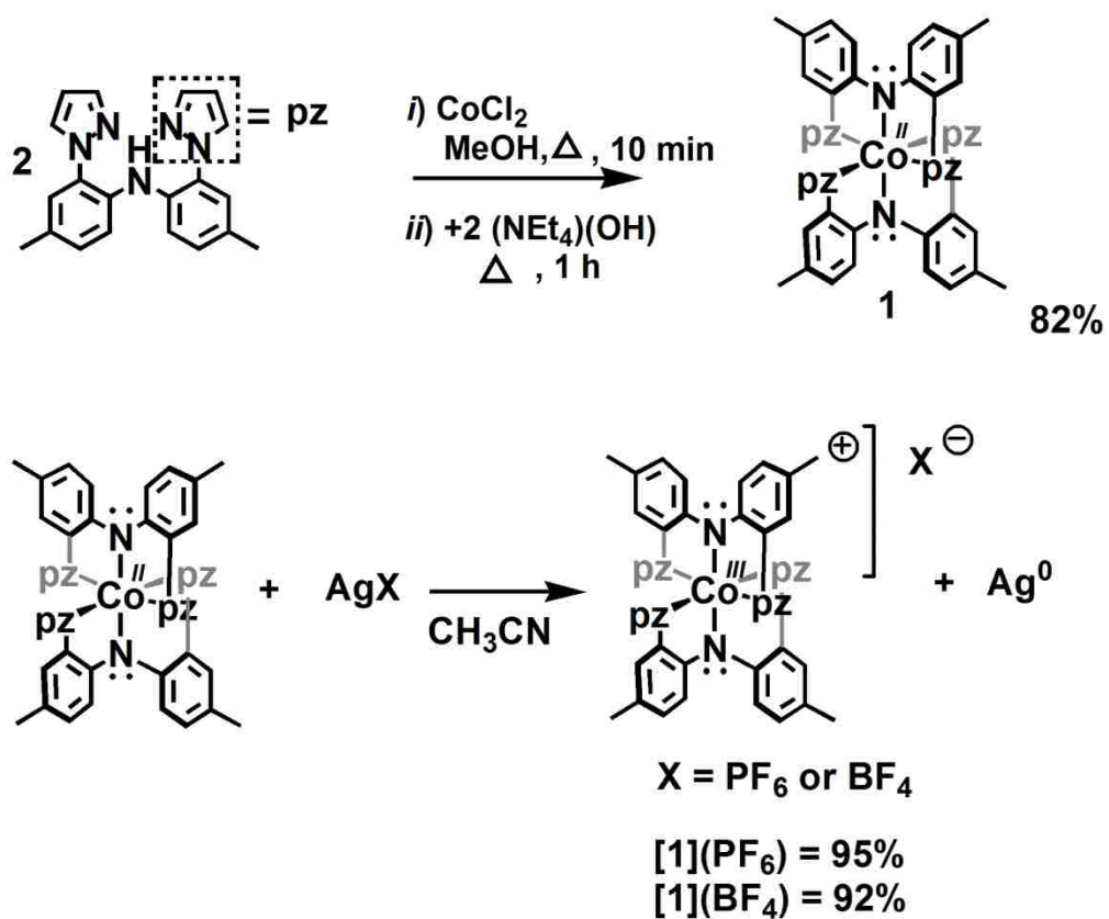
Scheme 3.1. Preparation of [\text{Co}(\text{Me},\text{Me})_2]\text{X} , [\text{1}]\text{X} complexes. ( \text{X} = \text{null or } \text{PF}_6 \text{ and } \text{BF}_4 ).
