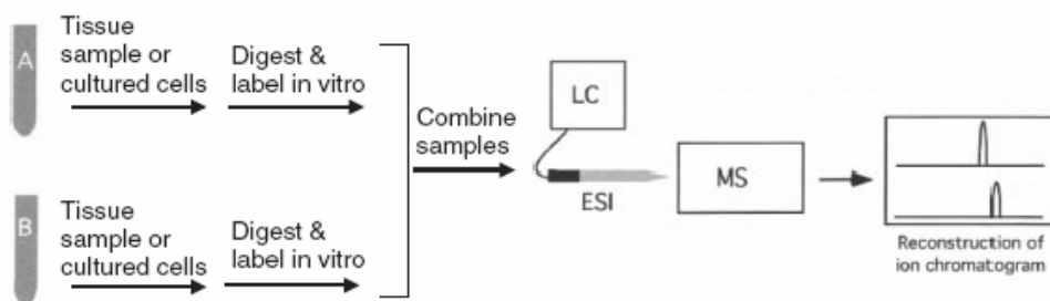
Figure 12: Mass Spectrometry Analysis of differential protein expression using in-vitro isotope tagging. 24
