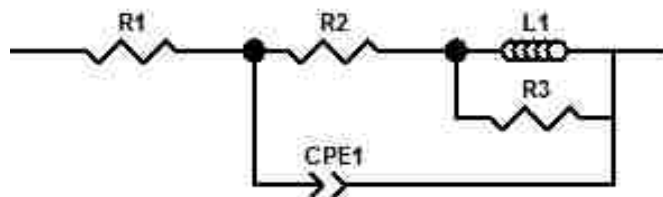
Figure 6-6 Equivalent circuit model for mild steel
