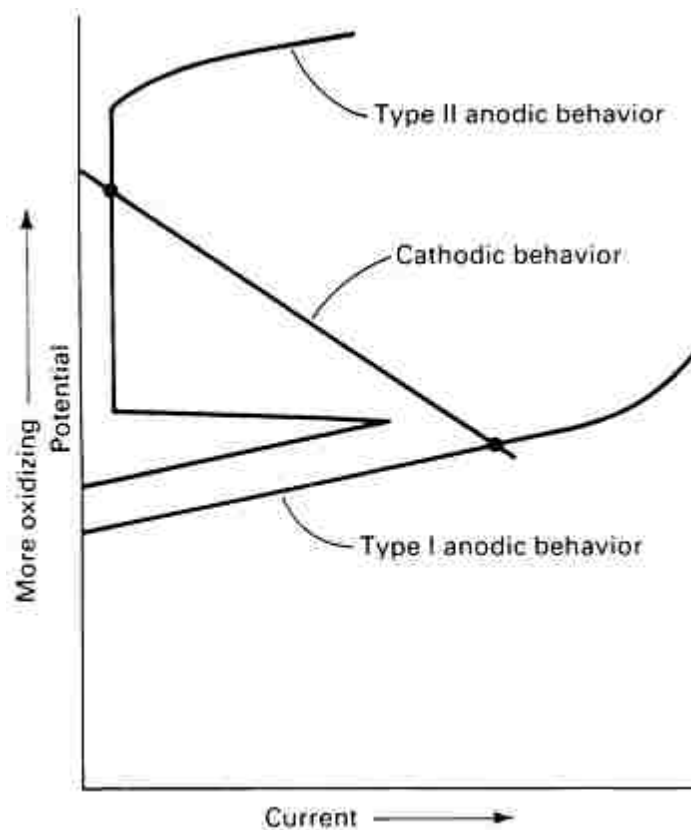
Figure 2-1 Different anodic behaviours of metals [14].
