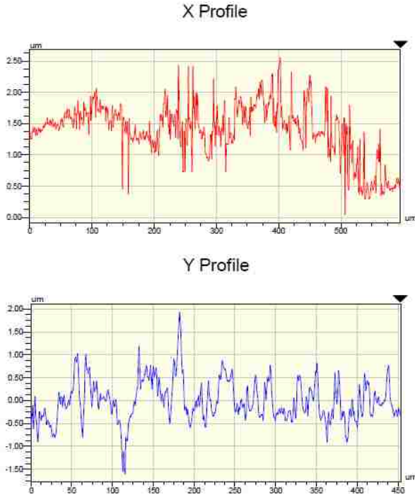
Figure 5-22 X-profile and Y-profile of sample G120 before corrosion
