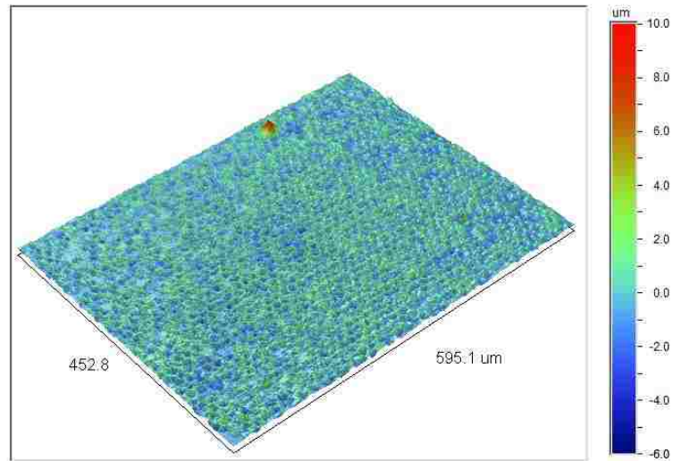
Figure 4-16 Sample D3.5L14 3D roughness after corrosion
