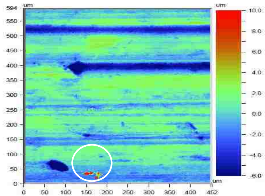
Figure 5-15 Sample G120 2D roughness after corrosion
