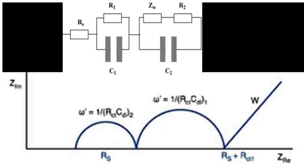
Figure 2-5 Experimental impedance spectra and the equivalent circuit for mild steel in dilute H_2SO_4 [34]
