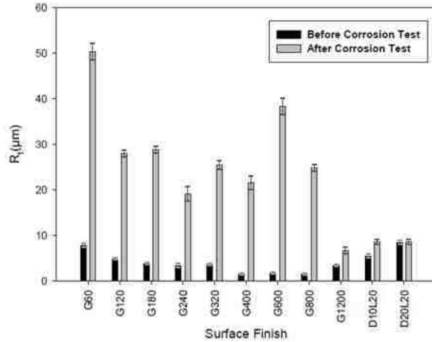
Figure 5-34 R_1 values for nickel before and after corrosion testing.
