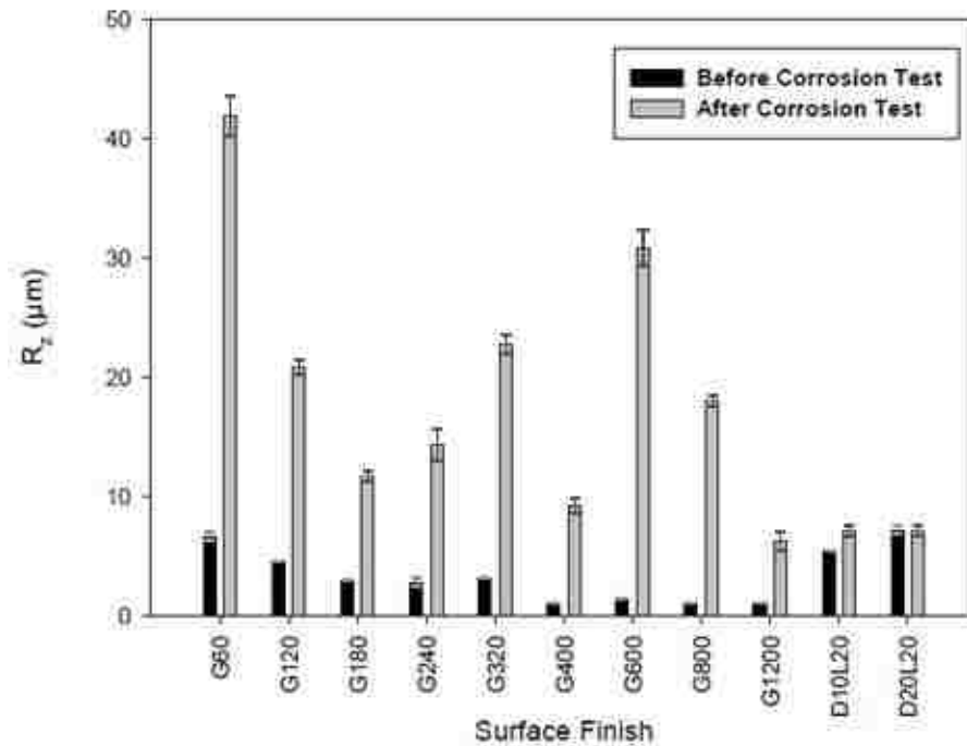
Figure 5-35 R_2 values for nickel before and after corrosion testing.
