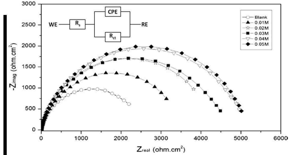
Figure 2-13 Experimental impedance spectra and the equivalent circuit for nickel in dilute H_2SO_4 [43]
