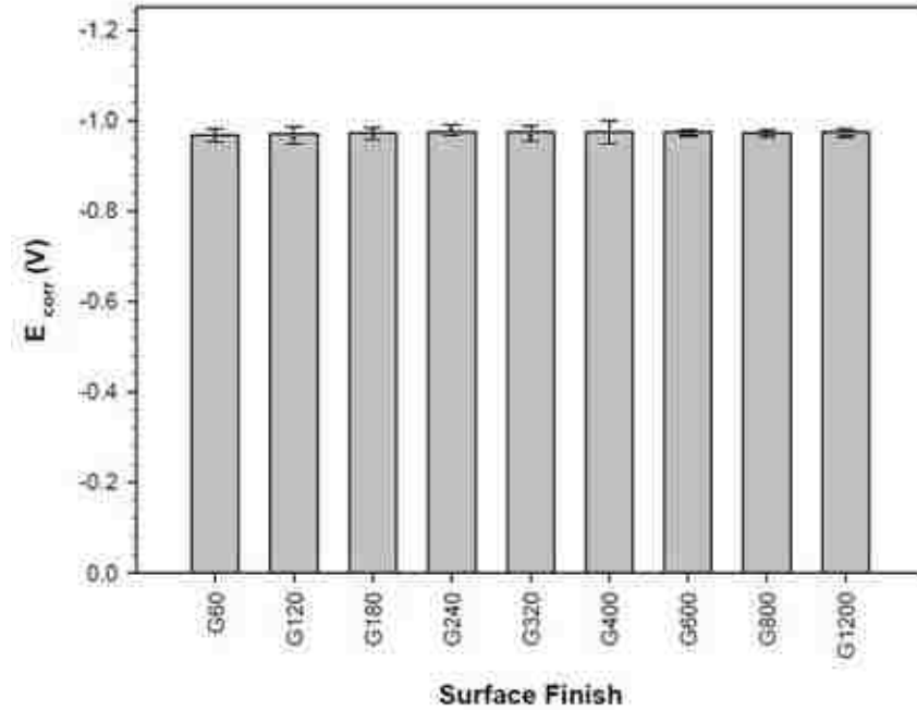
Figure 6-3 Dependence of E_{corr} on surface finish of mild steel
