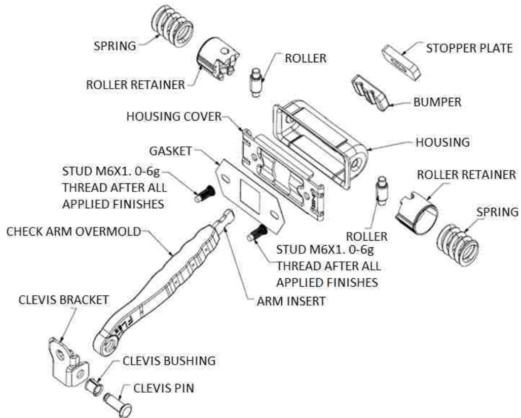
Figure 1-6: Exploded view of the door check system.
