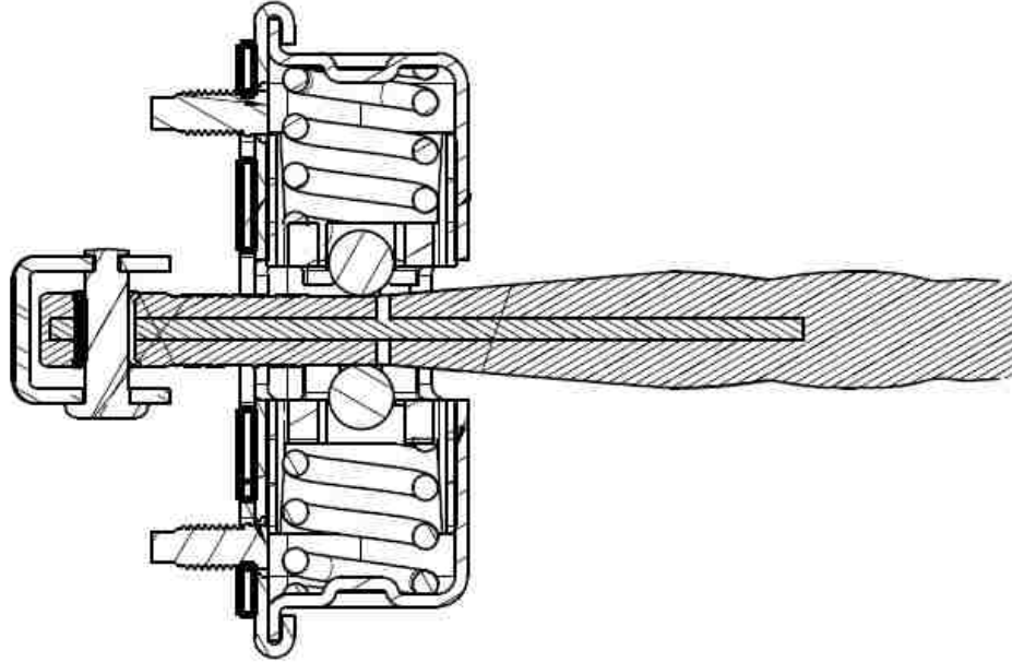
Figure 1-7: Check arm section. In the picture it is possible to see the two springs and the two roller bearings that allow the motion of the door along the check arm.
