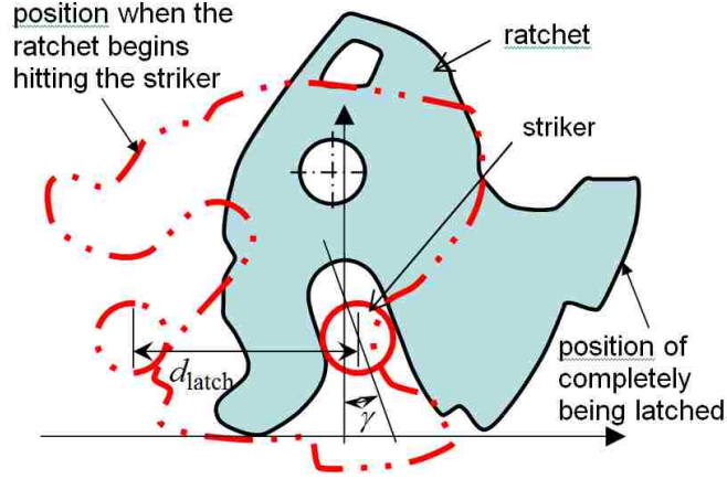
Figure 3-2: A schematic diagram for a latching system [24].
