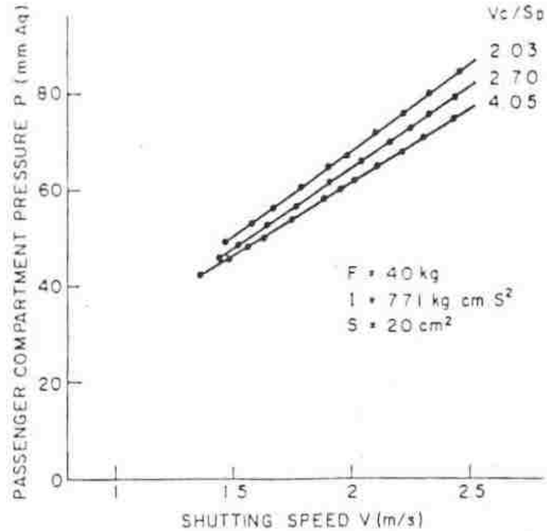
Figure 2-7: Passenger compartment pressure compared to door shutting speed [19].
