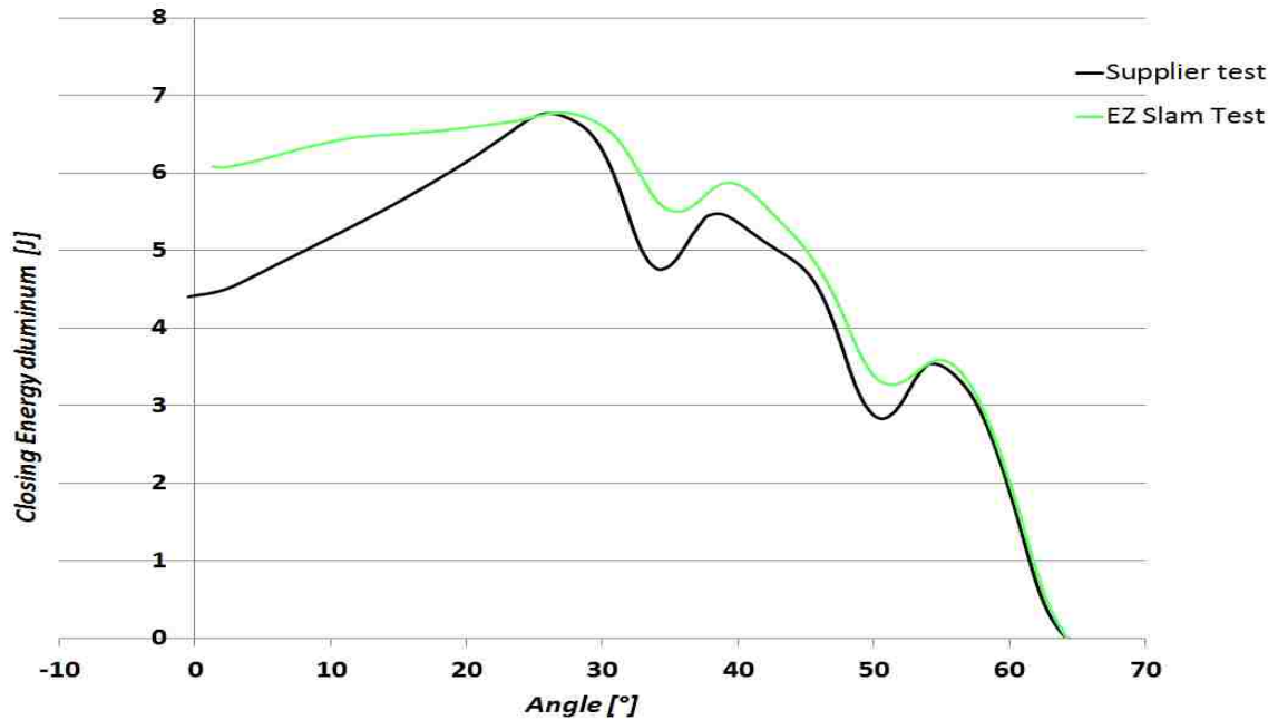
Figure 5-23: Closing energy comparison between the Supplier's tester measurements on the aluminum door setup and the EZ Slam measurement on the aluminum door.
