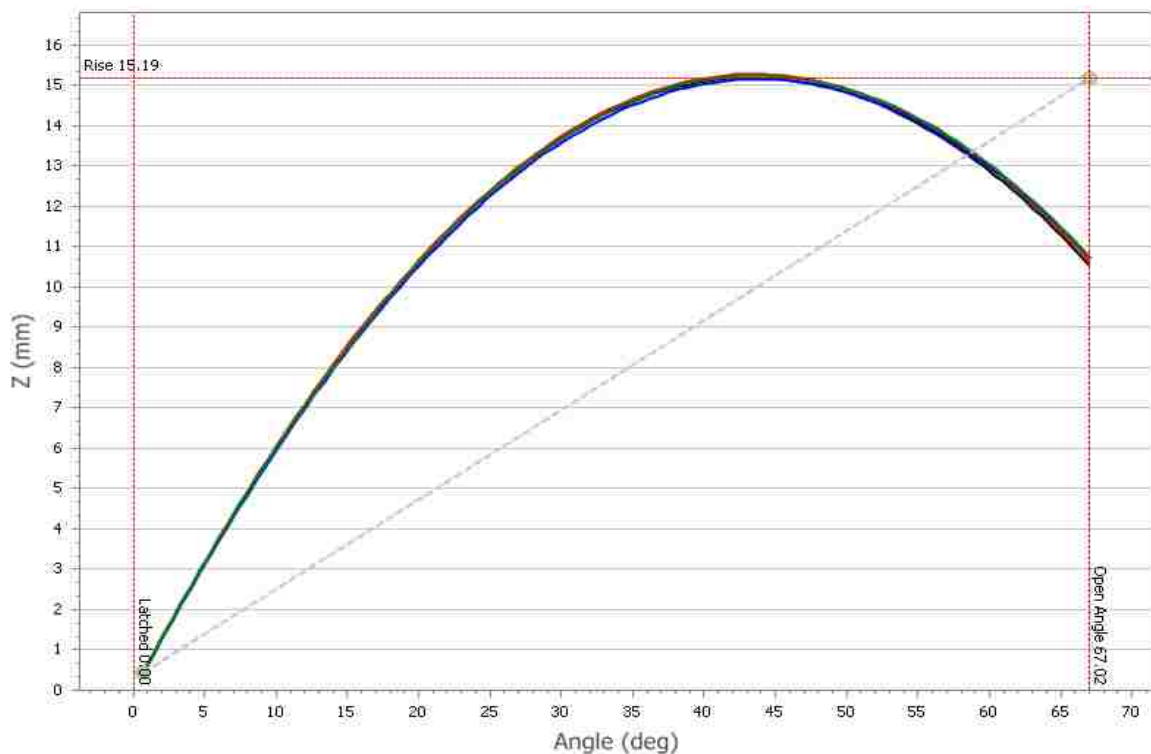
Figure 5-36: Door rise of the aluminum door during the closing event.
