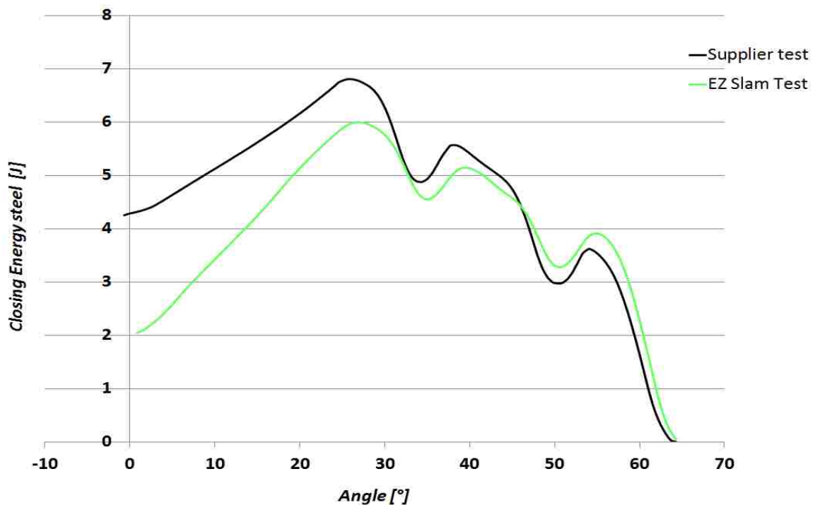
Figure 5-22: Closing energies comparison between the Supplier's tester measurements on the steel door setup and the EZ Slam measurement on the steel door.
