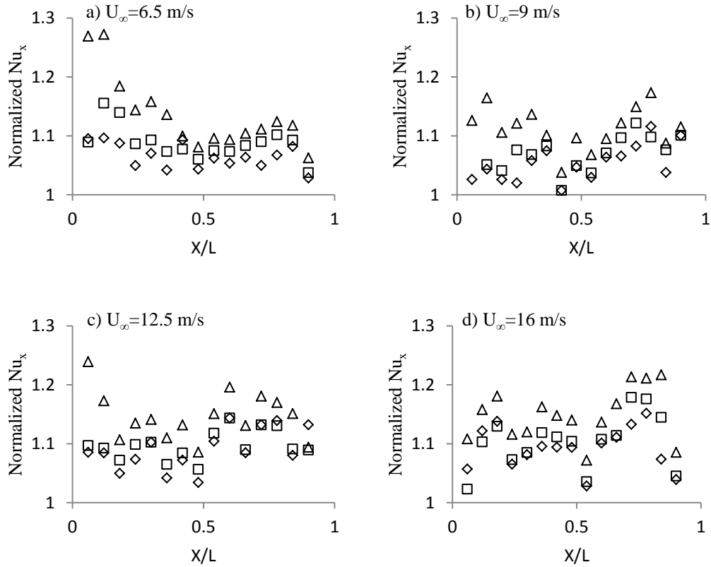
Figure 4.8: Normalized Nusselt number along the centerline of the plate ( \diamond , W=5 mm; \square , W=10 mm; \Delta , W=20 mm)
