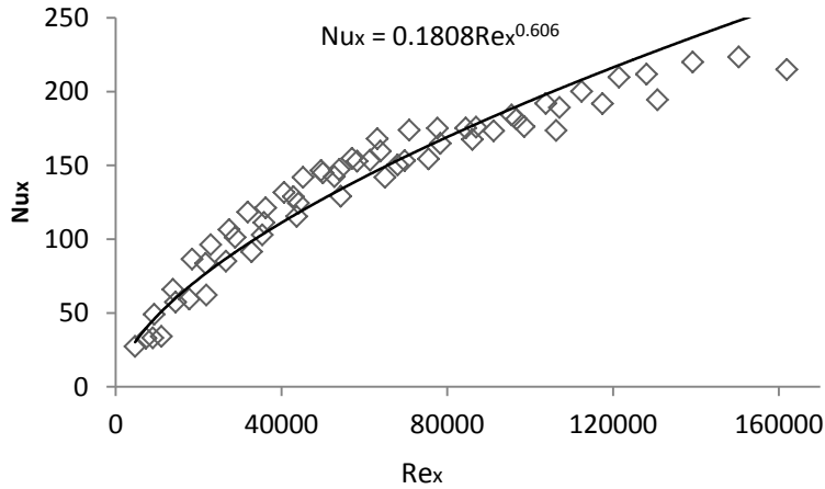
Figure 2.20: Overall local Nusselt number versus local Reynolds number with a turbulence generator (fin).
