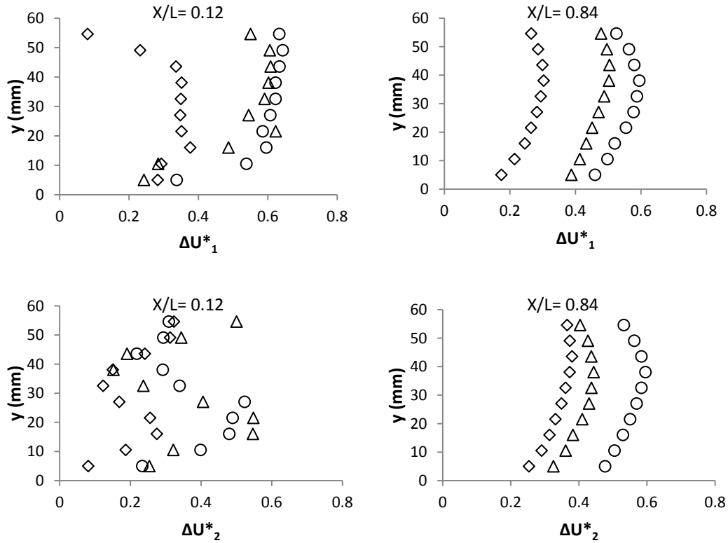
Figure 3.17: Local dimensionless velocity difference ( (\frac{u}{U_\infty})_{without\ fin} - (\frac{u}{U_\infty})_{with\ fin} ). ( \diamond , U_\infty = 7.3 m/s; \Delta , U_\infty = 13.5 m/s; \circ , U_\infty = 20.9 m/s).
