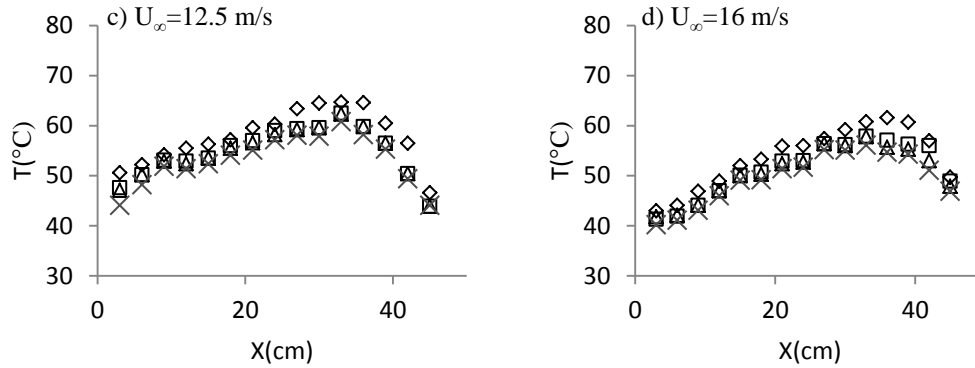
Figure 4.5: Variation of surface temperature along the centerline of the plate ( \diamond , W=0 ; \square , W=5 mm; \Delta , W=10 mm; \times , W=20 mm)
