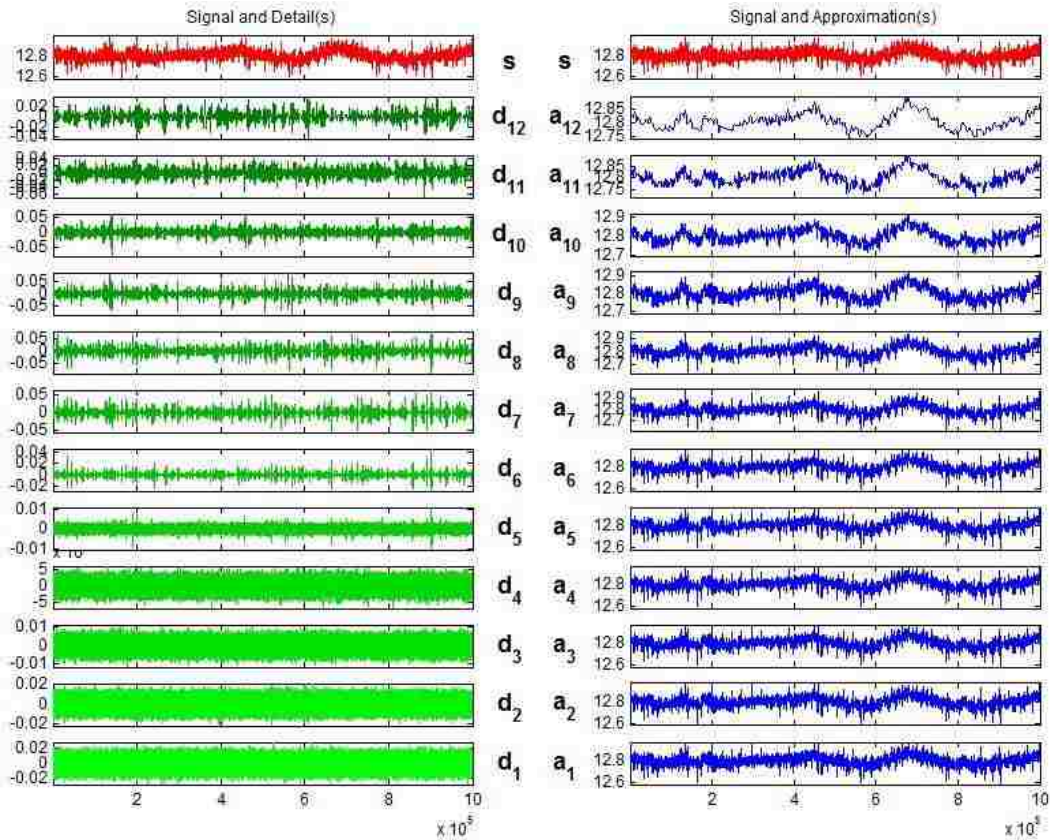
Figure A.4. Detail and approximation signal in each level
