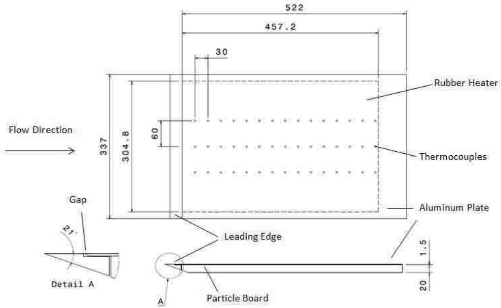
Figure 3.2: Configuration of the flat plate (dimensions are in mm).
