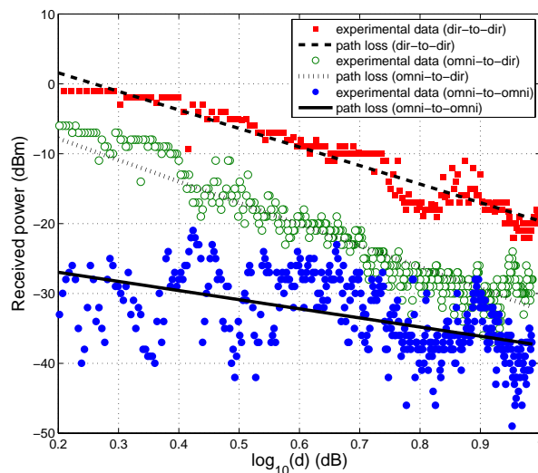
Figure 2.13: Impact of antenna angle in reducing small-scale fading. It can be seen that using an adaptive antenna with a small beamwidth can reduce the amount of multipath fading considerably and also increase the overall received signal power.
