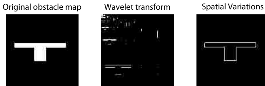
Figure 4.1: A T-shaped obstacle map with the obstacle areas denoted in white, where 100% of the energy is in 7.52% of the space samples (left), its transformed representation in wavelet domain, where 100% of energy is in less than 1.82% of the coefficients (center), and its spatial variations (right).
