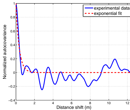
Figure 2.11: Exponential match for the normalized autocovariance of the log of shadowing variations. It can be seen that exponential provides a good match.
