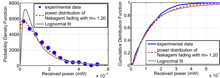
Figure 2.8: Comparison of Nakagami and lognormal for the distribution of small-scale fading – (left) pdf and (right) cdf.
