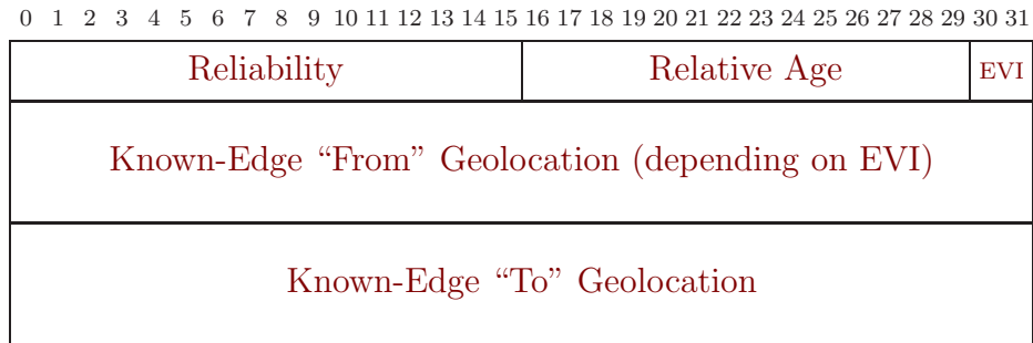
Known-Edge Block Diagram
