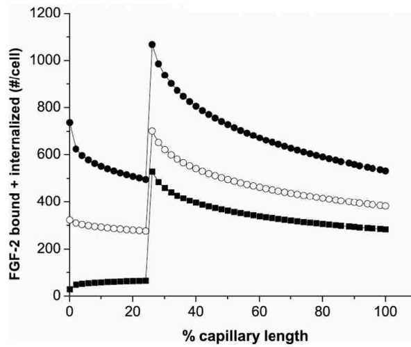
Figure 4.12: Simulations predict both FGFR and HSPG contribute to retention through FGF-2-mediated coupling. In these simulations, HSPG ( 2.5 \times 10^5 \# / cell ) were expressed on the cell-lined fibers along the entire chamber while FGFR ( 1 \times 10^4 \# / cell ) were expressed only in the cells found in the final 75% of the hollow fiber. FGF-2 (1ng) was added at time 0 (30% loss in the reservoir) at 0.65 (●), 1.3 (○), and 2.6 (■) mL/min pulsatile flow (1.3, 2.6, and 5.2 mm/sec respectively). Cell-bound+internalized FGF-2 after 5 min of simulation time is shown.
