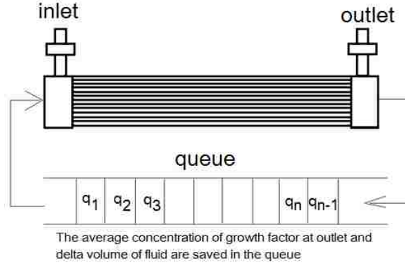
Figure 5.14: The diagram of a multi-pass simulation design. The average concentration of the growth factor at outlet is saved in a FIFO queue along with the delta volume of fluid in each time step. Once the original growth factor at inlet is depleted, switching to the queue, forming a simulation loop, but without mixing the growth factor in the queue.
