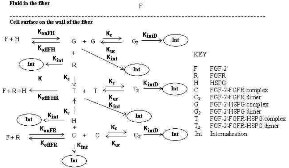
Figure 3.4: The diagram of binding kinetic pathway.
