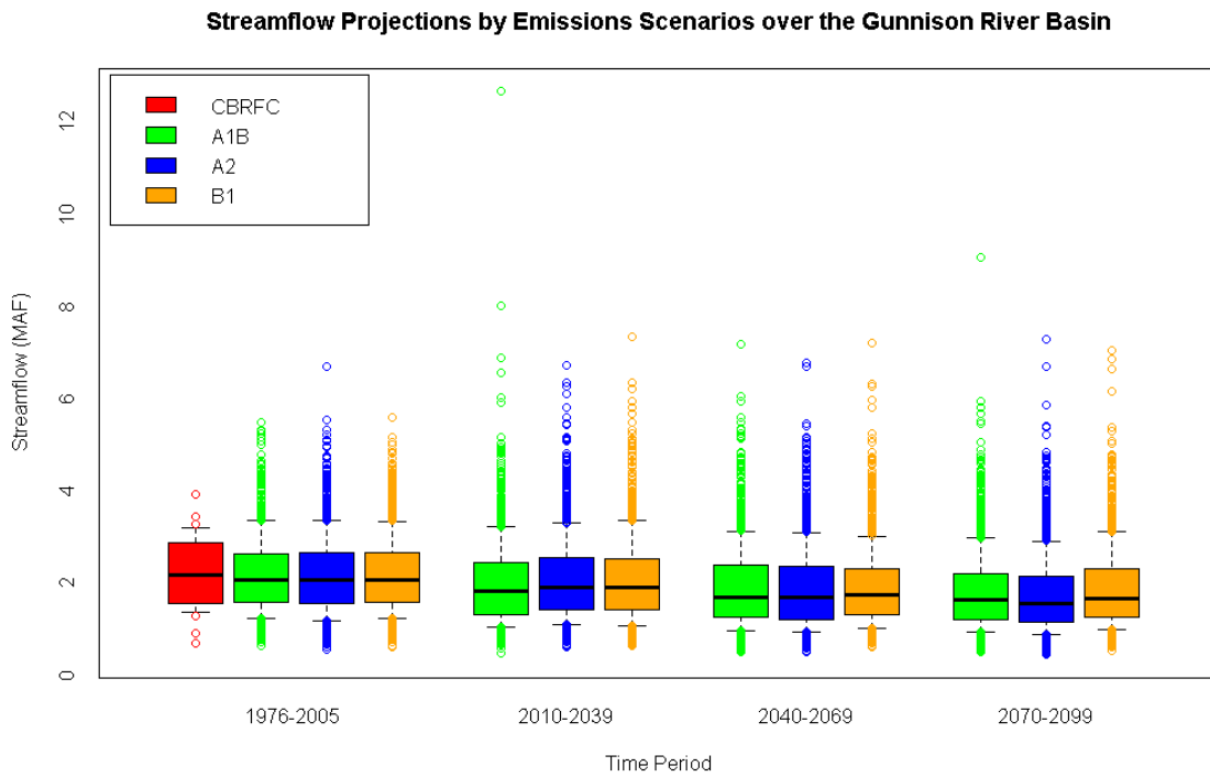
Figure 37: Streamflow Projections over the Gunnison River Basin separated by emissions scenarios.
