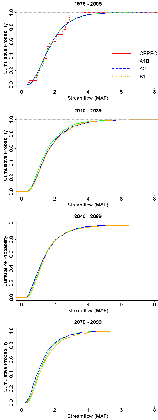
Figure 47: Plots of CDFs of projected streamflow over the San Juan River Basin.
