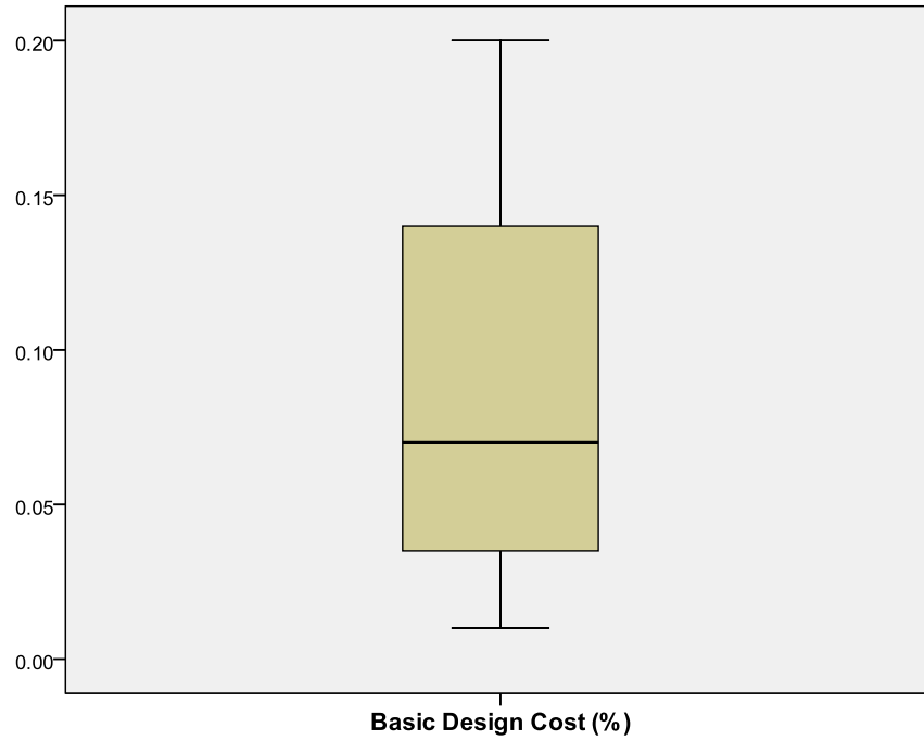
Figure 28. Box plot of basic design cost (%) of CCDPW flood control projects
