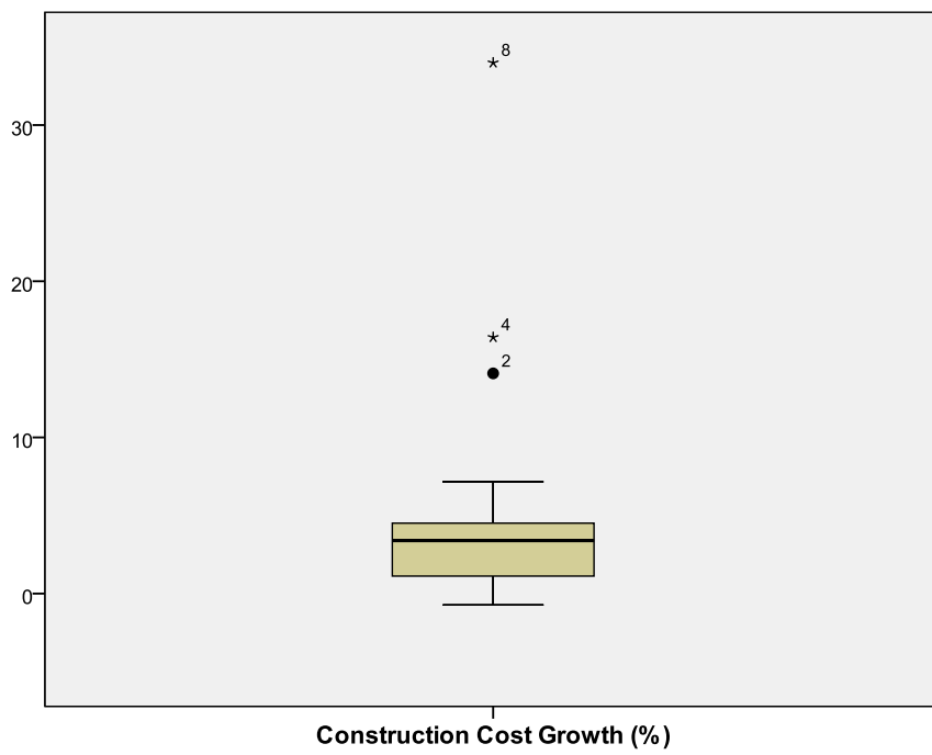
Figure C- 22. Box plot for construction cost growth (%) of TXDOT road projects
