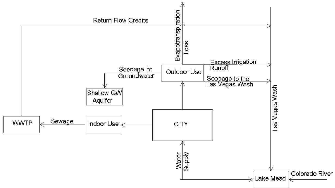
Figure 2.4. A portion of the water balance model showing a city system
