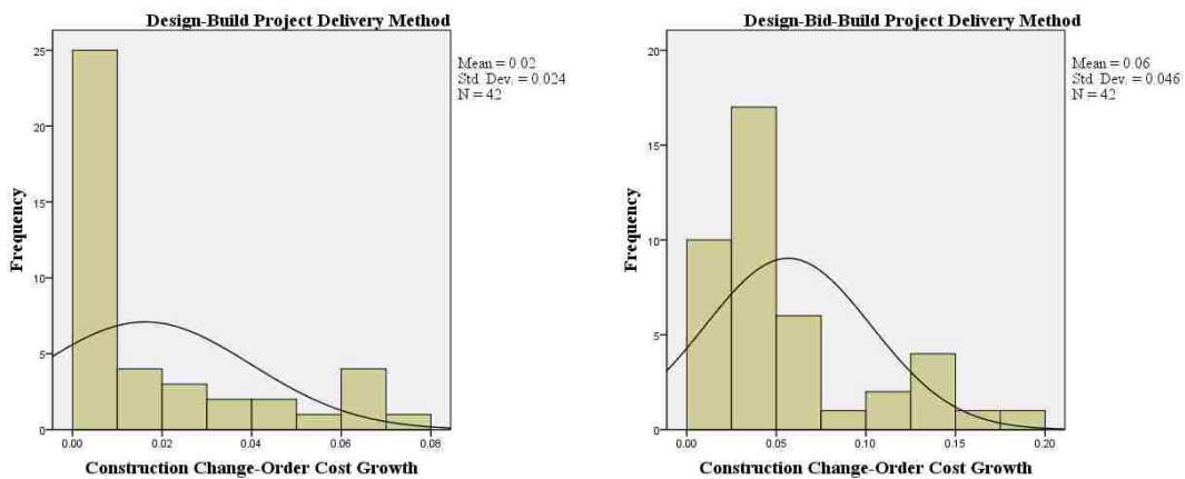
Figure 20. Histogram of Construction Change-Order Cost Growth.
