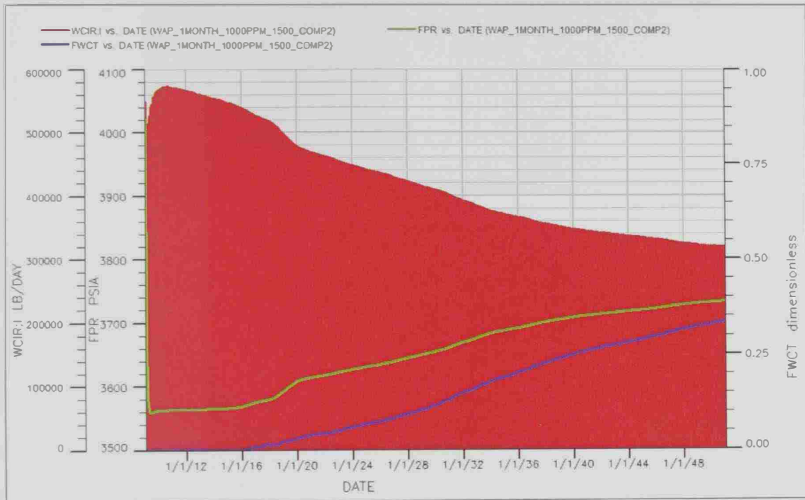
Figure 5.34: WAP injection at 1500 STB/D (1000 ppm, COMP2, 1 month) reservoir performance
