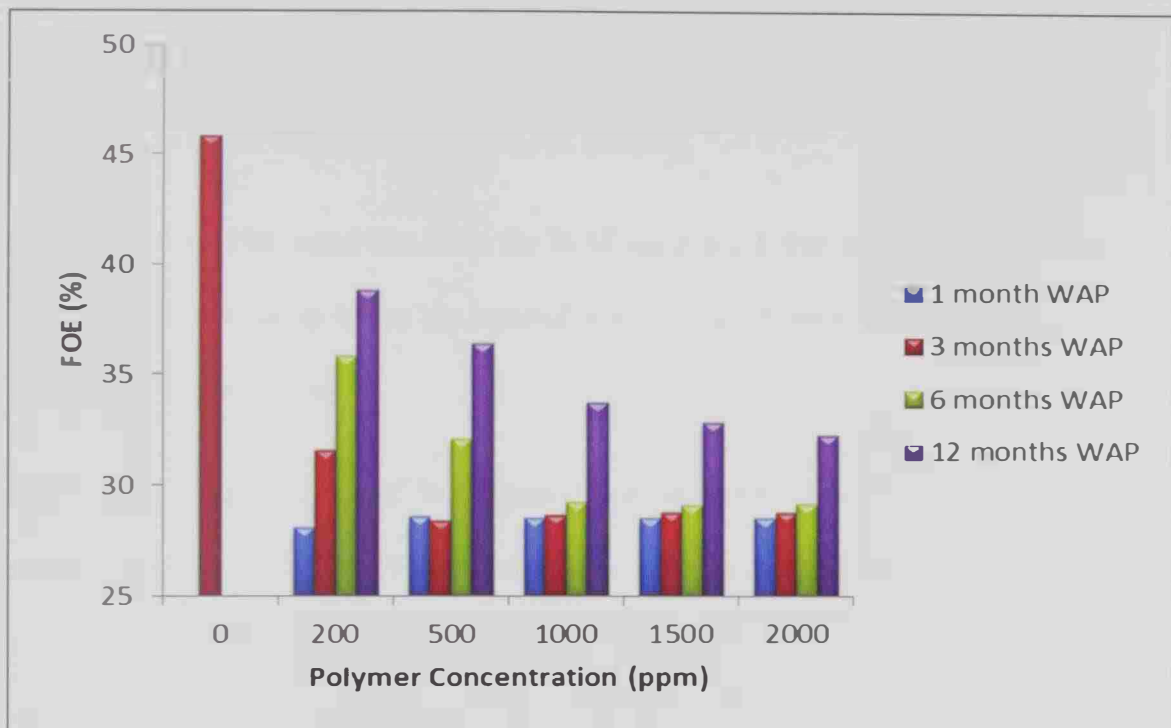
Figure 5.51: FOE vs. polymer concentration using COMP3 (WAP injection)
