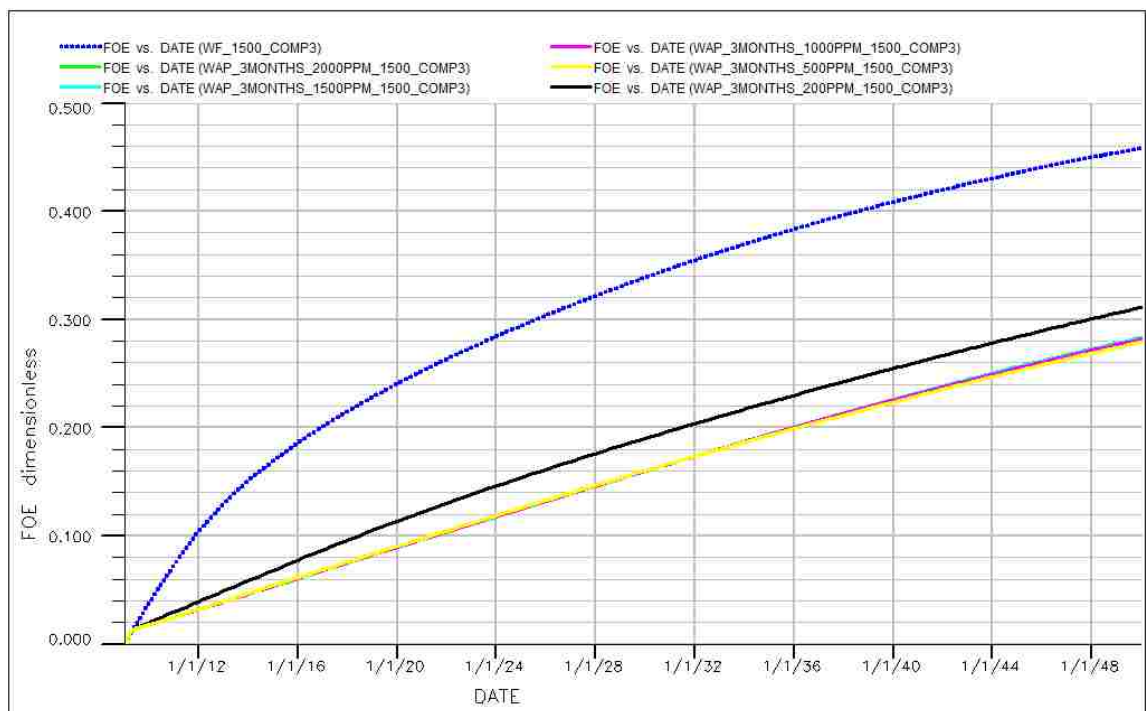
Figure 5.48: Oil recovery for 3 months WAP injection using COMP3
