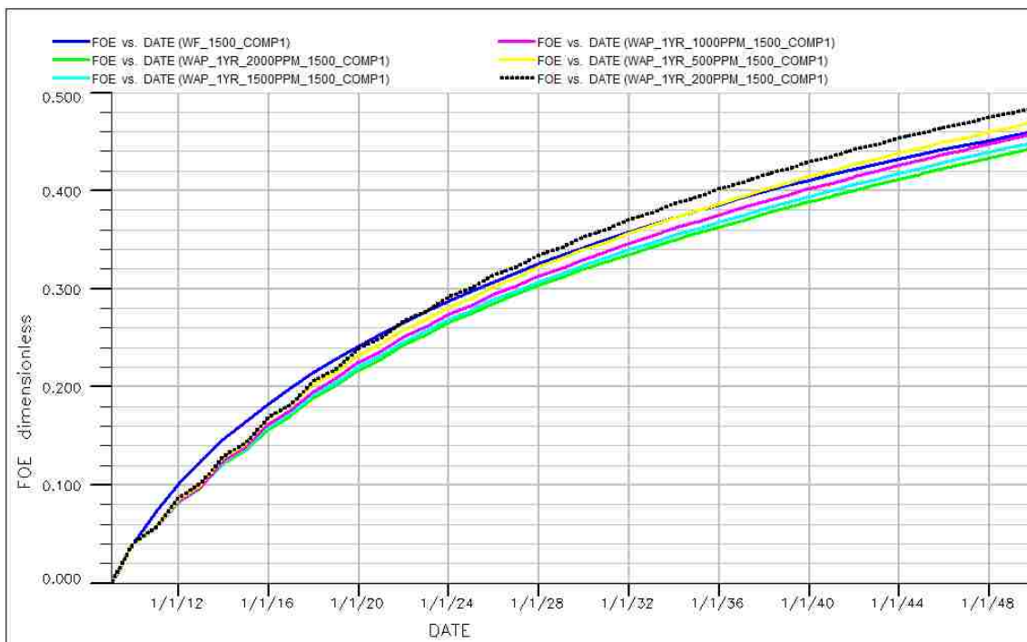
Figure 5.32: Oil recovery for 1 year WAP injection using COMP1
