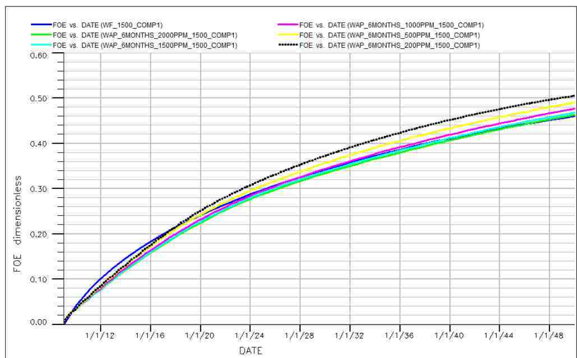
Figure 5.31: Oil recovery for 6 months WAP injection using COMP1
