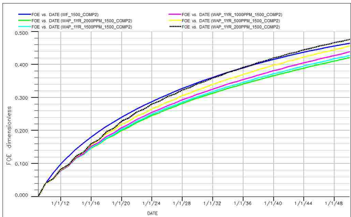
Figure 5.41: Oil recovery for 1 year WAP injection using COMP2
