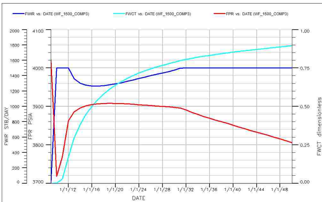
Figure 5.12: Waterflooding injection at 1500 STB/D (COMP3) reservoir performance
