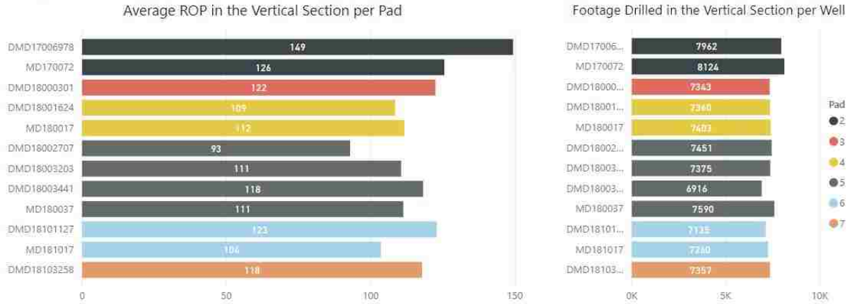
Figure 3.3. Visualization of the Average ROP in the Vertical Section
