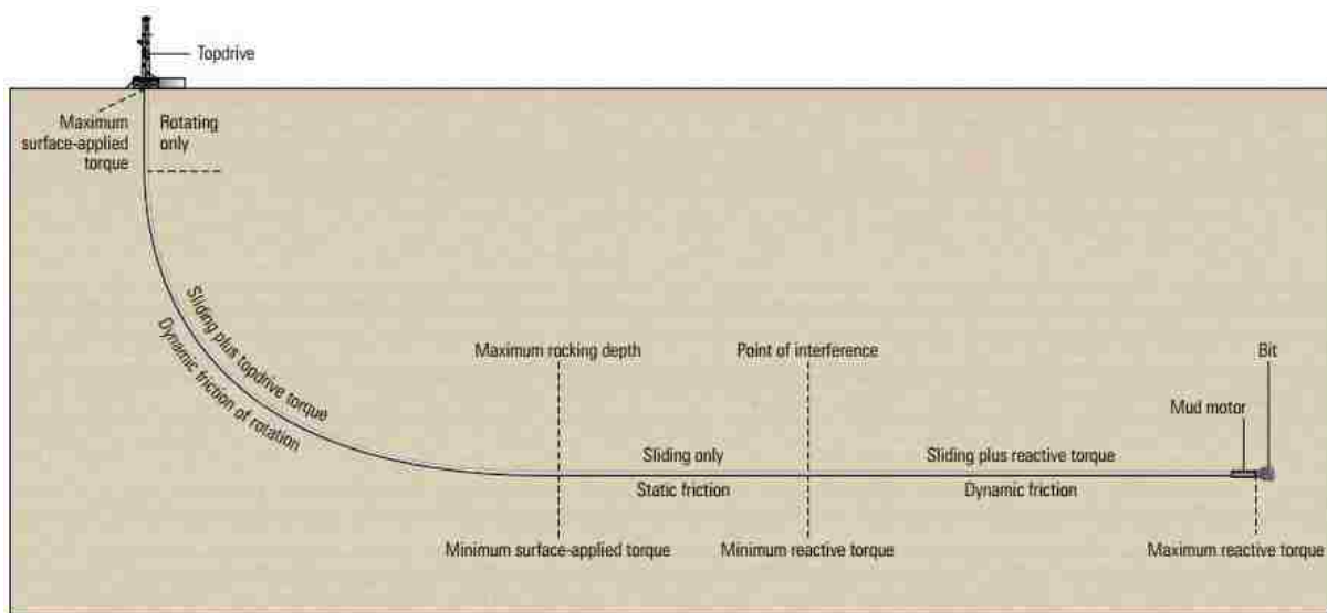
Figure 2.9. Representation of the Different Zones of the Drill String During Rocking, From [Duplantis, 2016]
