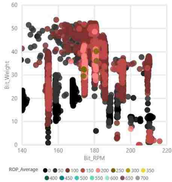
Figure 3.16. Heat Map of WOB vs Bit RPM for the Second Half of Depth Intervals
