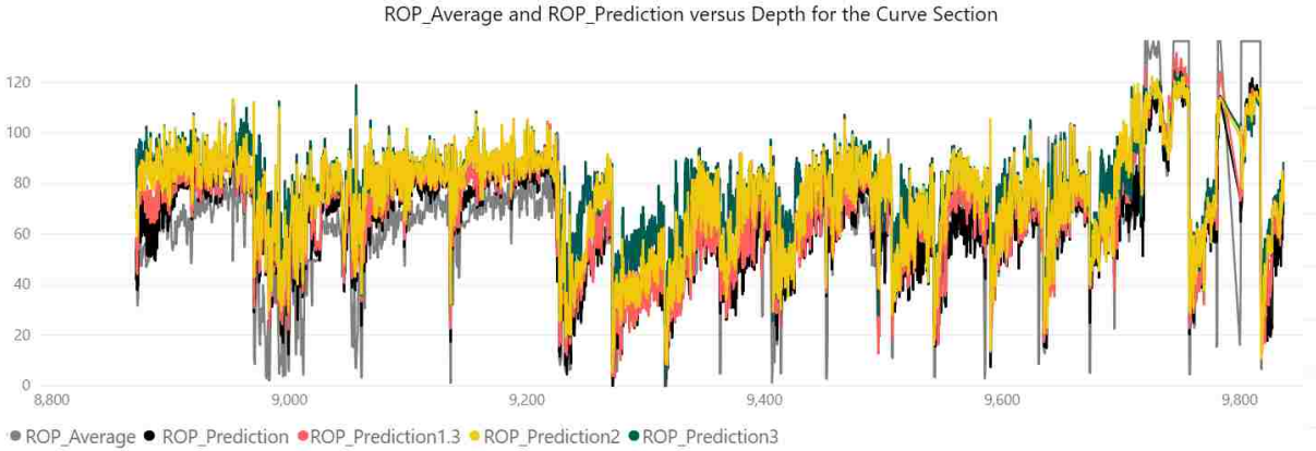
Figure 4.10. Resulting ROP Prediction for ROP of 1.3, 2 and 3 Times Higher
