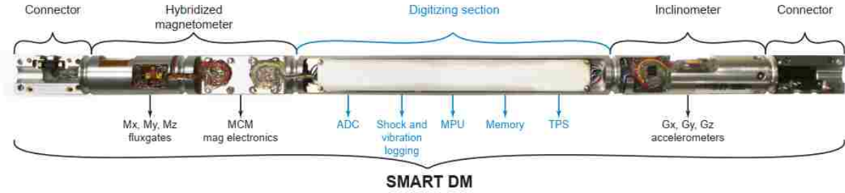
Figure 1.8. Typical MWD Assembly, From JAE Smart DM 2016 Catalog
