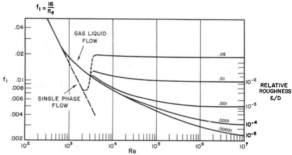
Figure 2.8. Dimensionless f_1 factor as a function of Re and relative roughness \epsilon/D [11].
