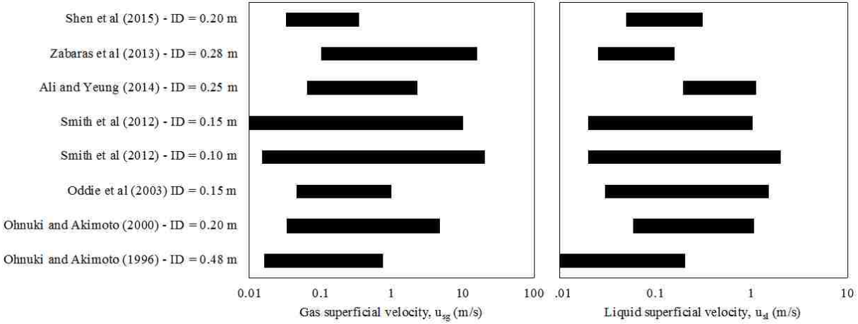
Figure 3.2. Literature review on works with characterized flow regimes for vertical upward two-phase flows in large diameter pipes.
