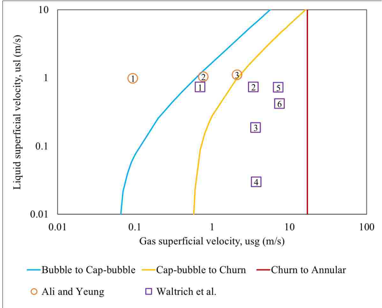
Figure 4.3. Data points evaluated with CFD on Waltrich et al. [9] work plotted on newly proposed flow regime map.
