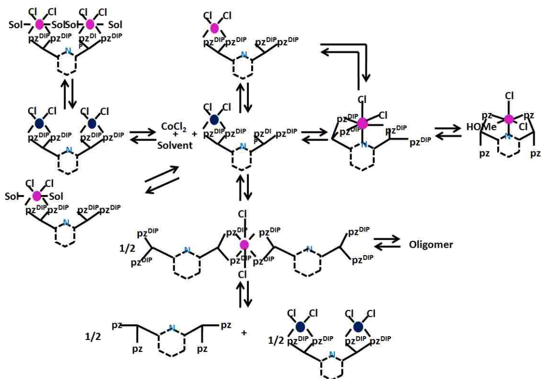
Figure 3.21. Alternative equilibrium process occurring in methanol.
