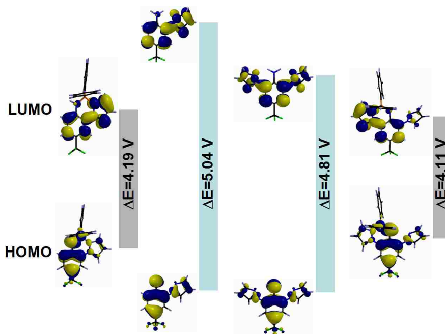
Figure 6.7. HOMO (bottom) and LUMO (top) for (from left to right): Ph 2 B(pzAn CF 3 ) H(pzAn CF 3 ), H(pz 2 An CF 3 ), Ph 2 B(pz 2 An CF 3 ) from density functional calculations (B3LYP/6-31G*). Vertical scale represents relative energy. Gas phase HOMO-LUMO gap energy ( \Delta E ) from calculations is given for ligands (blue) and BORAZANs
