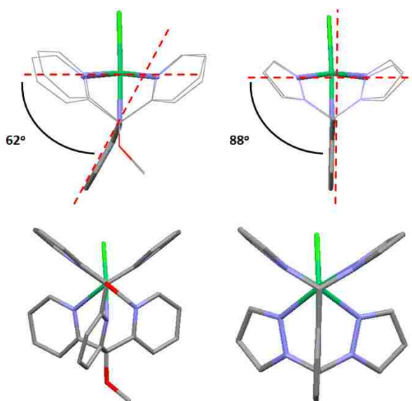
Figure 2.5. Comparison of the structures of related [NiCl(L)]^+ cations ( L = PY5 , left; L = pz_4lut , right). H atoms are omitted. Top: views orthogonal to the axial pyridyl. Bottom: Views down C – O ( PY5 ) or C – H ( pz_4lut ) bonds.
