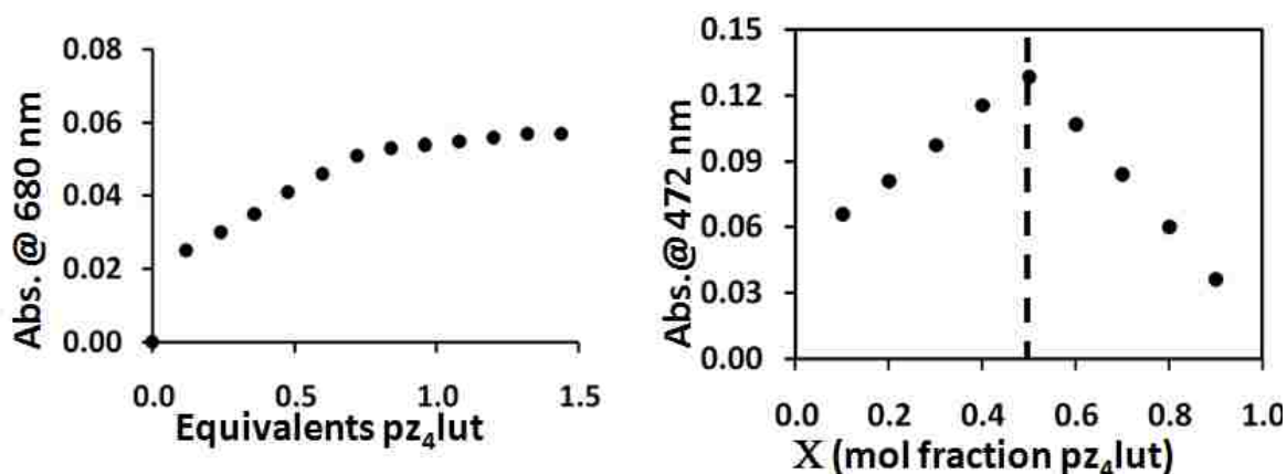
Figure 3.11. Titration of pz* 4 lut (in MeOH) into a methanol solution of CoCl 2 (left) and Job's plot in MeOH of pz* 4 lut.
