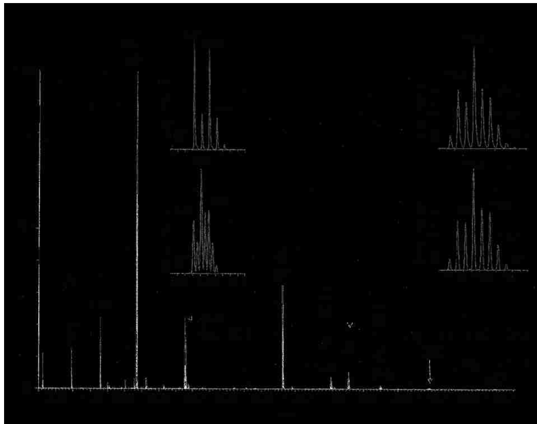
Figure 1.7. ESI(+) mass spectrum of [\text{Ag}(\text{pz}^4\text{lut})][\text{BF}_4] , 2 in \text{CH}_3\text{CN} .
