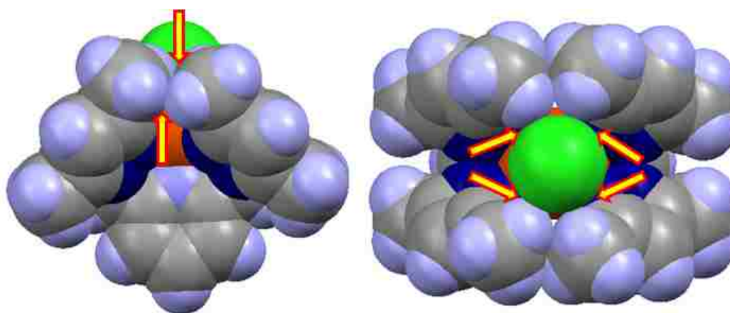
Figure 4.4. Space-filling model of 3a \cdot 2\text{MeOH} highlighting the steric interactions between methyls (left) and between methyls and chloride groups (right).
