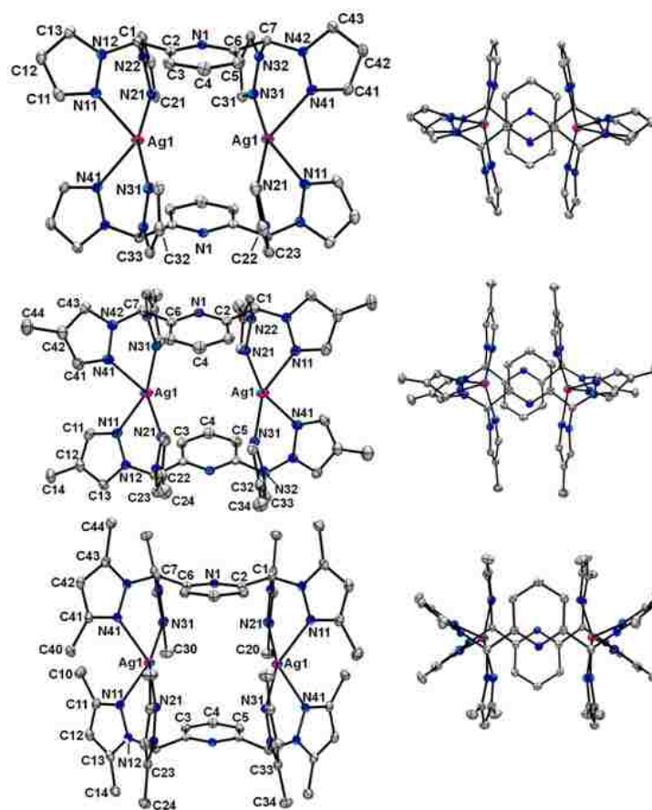
Figure 1.3. Views of the cyclic dications in [\text{Ag}(\text{pz}_4\text{lut})](\text{BF}_4) ( \mathbf{1} ), top; [\text{Ag}(\text{pz}^{\text{4'}}_4\text{lut})](\text{BF}_4)\cdot\text{CH}_3\text{CN} , \mathbf{2}\cdot\text{CH}_3\text{CN} , middle; and [\text{Ag}(\text{pz}^{\text{*4}}_4\text{lut})](\text{BF}_4)\cdot\text{CH}_3\text{CN} , \mathbf{3}\cdot\text{CH}_3\text{CN} , bottom; Left, perspective view; Right, view normal to pyridyl plane. Each with thermal ellipsoids shown at 50% probability and with hydrogens removed for clarity.
