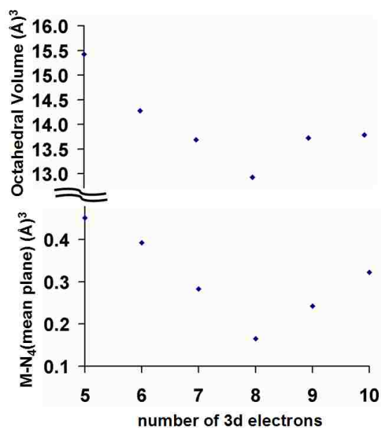
Figure 2.4. Plots of MN_5Cl octahedral volume (top) and deviation of M from equatorial N_4 plane (bottom) versus d-electron count of metal in [MCl(pz_4lut)]^+ complexes.
