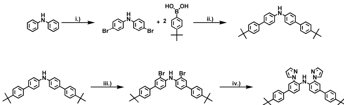
Scheme 7.1. Synthetic route to new ligand L 1 . i.) 2 NBS, 0 °C, DMF, 3 h. ii.) 5 mol % Pd(0), 2 M aq. K 2 CO 3 , toluene/MeOH, 80 °C, 20 h. iii.) 2 Br 2 , 1:1 MeOH/CH 2 Cl 2 , 0 °C, 1 h. iv.) 3.5 HPz, 3.5 K 2 CO 3 , 10 mol % CuI, 40 mol % DMED, xylenes, 3 d.
