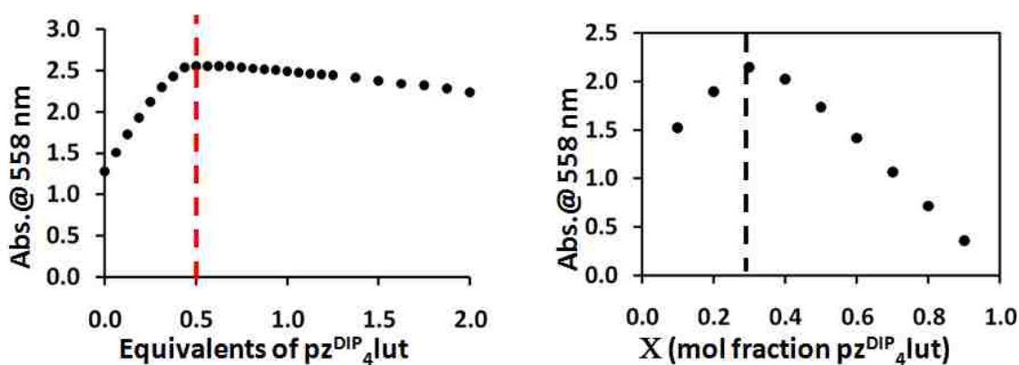
Figure 3.13. Titration of \text{pz}^{\text{DIP}}_4\text{lut} solution ( \text{CH}_2\text{Cl}_2 ) into a \text{CoCl}_2 solution ( \text{CH}_3\text{CN} , left). Job's plot of \text{pz}^{\text{DIP}}_4\text{lut} and \text{CoCl}_2 in acetonitrile and dichloromethane showing 1:2 stoichiometry.
