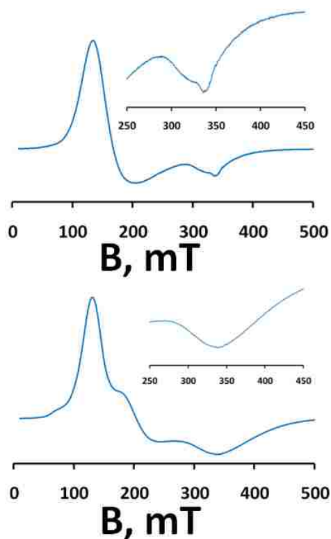
Figure 3.6b. EPR Spectra of of (\text{CoCl}_2)_2(\mu\text{-pz}^X_4\text{lut}) ; (X = 3,5-dimethyl, top, 6 ); (X = 3,5-DIP, Bottom, 7 ) as Frozen Glass Solutions in Acetonitrile:Toluene.
