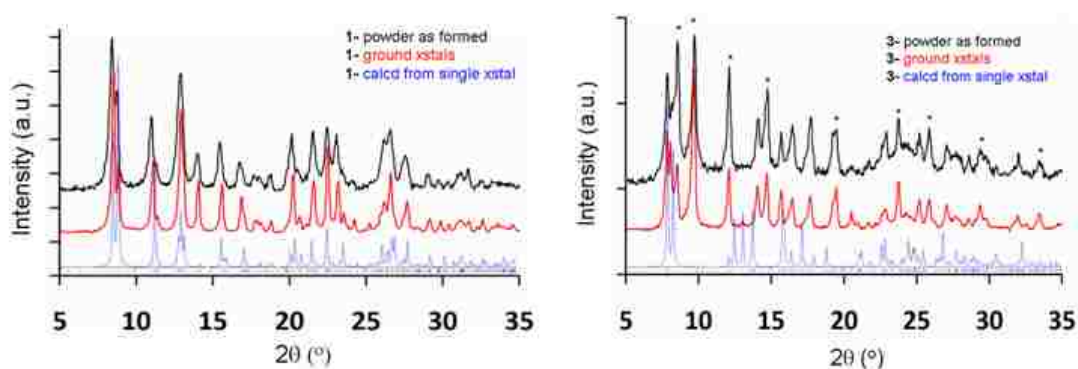
Figure 1.6. X-Ray Powder diffraction patterns of 1 (left) and 3 (right) obtained for initially obtained precipitate of preparative reactions in THF (top, black) and for bulk crystalline samples (middle, red) after drying and grinding. The calculated diffraction patterns based on single crystal diffraction experiments are also given (bottom, blue). For 3 , reflections demarcated with asterisks (*) are not found in the calculated pattern of the solvate 3 ·CH 3 CN.
