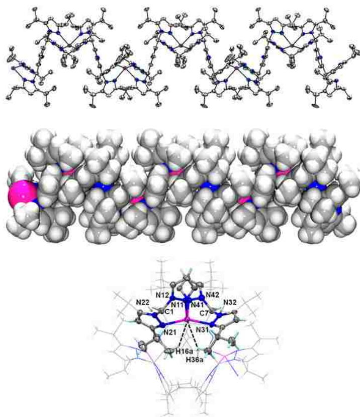
Figure 1.5. Views of the cation in [\text{Ag}(\text{pz}^{\text{DIP}}\text{4lut})](\text{OTf}) \cdot \text{CH}_3\text{CN} \cdot 0.5\text{Et}_2\text{O} ( 5 \cdot \text{CH}_3\text{CN} \cdot 0.5\text{Et}_2\text{O} ). Top: ORTEP drawing (thermal ellipsoids shown at 50% probability and with hydrogens removed for clarity) of a fragment of one polymeric chain that propagates along a -axis. Middle: Space-filling representation of same fragment. Bottom: A view approximately down the a -axis emphasizing the coordination environment about silver.
