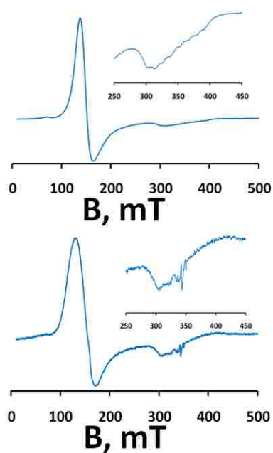
Figure 3.6a. EPR Spectra of of (\text{CoCl}_2)_2(\mu\text{-pz}^X_4\text{lut}) ; (X = H, top, 4 ); (X = 4-Me, 2nd, 5 ).
