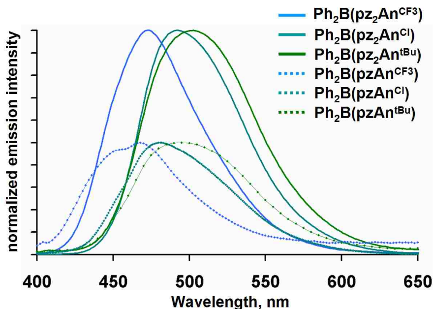
Figure 6.11. Overlay of normalized emission spectra of \text{Ph}_2\text{B}(\text{pz}_2\text{An}^X) (solid lines) and \text{Ph}_2\text{B}(\text{pzAn}^X) (dashed lines, arbitrarily set to half-intensity of dipyrazolyl derivatives) where ( X = \text{CF}_3 , blue; \text{Cl} , cyan; \text{tBu} , green).
