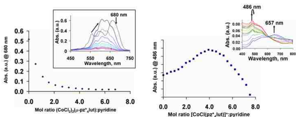
Figure 3.9. Titration of pyridine into solutions of (\text{CoCl}_2)_2(\mu\text{-pz}^*_4\text{lut}) in \text{CH}_3\text{CN} (left) and of [\text{CoCl}(\text{pz}^*_4\text{lut})][\text{Cl}] in \text{MeOH} (right).
