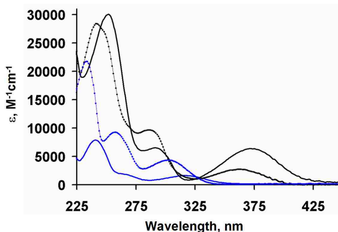
Figure 6.10. Overlay of electronic absorption spectrum of H(pzAn CF 3 ) (dotted blue line), H(pz 2 An CF 3 ) (solid blue line), Ph 2 B(pzAn CF 3 ) (dotted black line), and Ph 2 B(pz 2 An CF 3 ) (solid black line) in CH 2 Cl 2 .
