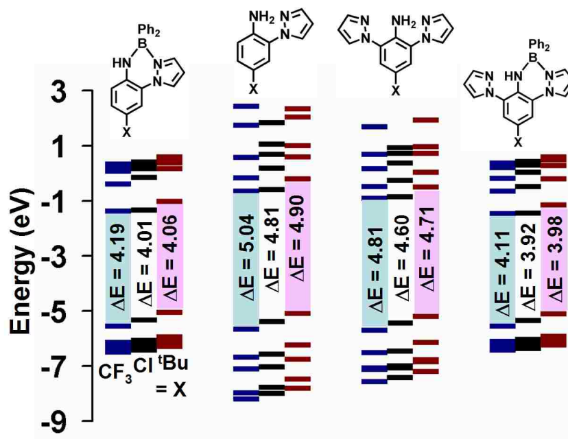
Figure 6.7. HOMO (bottom) and LUMO (top) for (from left to right): Ph 2 B(pzAn CF 3 ) H(pzAn CF 3 ), H(pz 2 An CF 3 ), Ph 2 B(pz 2 An CF 3 ) from density functional calculations (B3LYP/6-31G*). Vertical scale represents relative energy. Gas phase HOMO-LUMO gap energy ( \Delta E ) from calculations is given for ligands (blue) and BORAZANs
