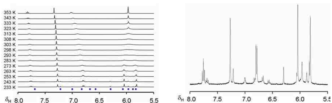
Figure 1.9. Left: The downfield region of the ^1\text{H} NMR spectrum of 3 in \text{CD}_3\text{CN} acquired at different temperatures emphasizing both a dynamic process and the equilibrium formation of a new species at low temperature (blue circles). Right: Magnified view of the 233 K spectrum.
