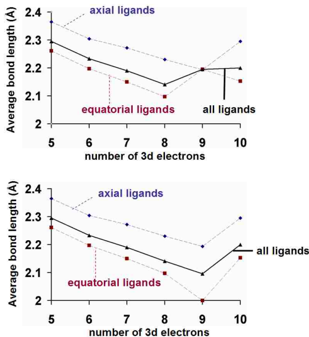
Figure 2.3. Plots of bond distances as a function of d-electron count of metal in [MCl(pz_4lut)]^+ . Average of all groups of MN_5Cl considered (top). Long Cu-N(pyrazoly) bond distances ignored (bottom).
