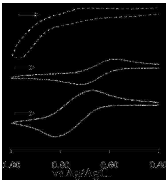
Figure 4.9. Cyclic voltammograms of 1 •CH 2 Cl 2 (bottom), 2 •MeOH•Et 2 O (middle) and 3a •2MeOH (top) in methanol (1 mM) with 0.1 mM [NBu 4 ][HSO 4 ]. Scan rate = 100 mvs.
