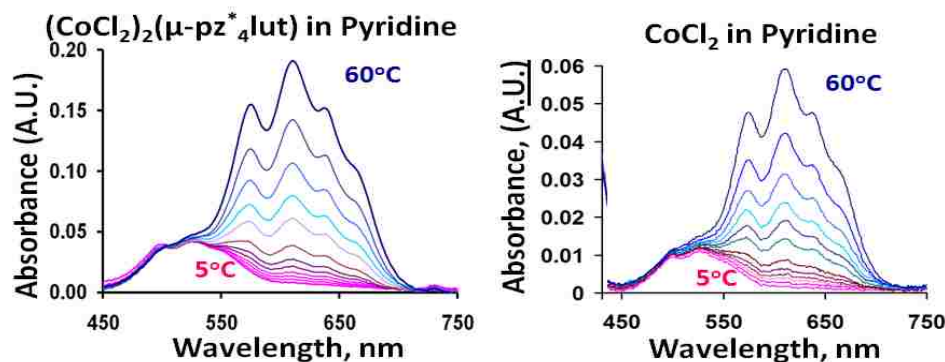
Figure 3.10. Variable temperature absorption spectra in pyridine of (CoCl 2 ) 2 (μ-pz* 4 lut) (left) and CoCl 2 (right).
