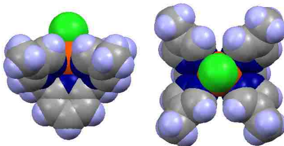
Figure 4.11. Spacefilling model of the cation of 2\bullet\text{MeOH}\cdot\text{Et}_2\text{O} showing the lack of steric interactions.
