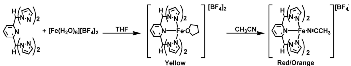
Scheme 5.1. Synthesis of [\text{Fe}(\text{THF})(\text{pz}_4\text{lut})][\text{BF}_4]_2 ( 1 ) and [\text{Fe}(\text{CH}_3\text{CN})(\text{pz}_4\text{lut})][\text{BF}_4]_2 ( 2 ).
