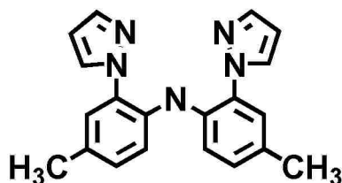
Figure 7.2. Recently reported NNN type pincer ligand by our group.
