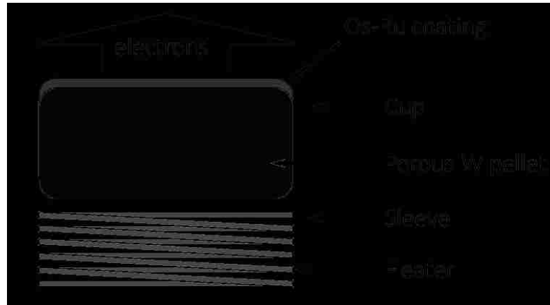
Figure 1.1 Schematic of the typical design of a thermionic dispenser cathode used by Semicon Associates. An Os-Ru thin film was coated on the porous W pellet on the heating element.
