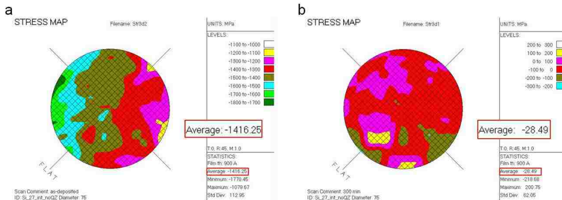
Figure 3.5 Stress maps of (a) as-deposited PdNi precursor alloy (90 nm thick) and (b) dealloyed np-Pd films generated by the wafer curvature system. The stress was 1.4 GPa (in compression) in the as-deposited film and decreased to 28 MPa (in compression) after the film dealloyed for 5 hrs.
