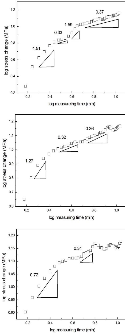
Figure 8.8 Log-log plots of stress change vs. measuring time of a 200 nm np-PdNi film during the hydridation segments of three consecutive cycles. Each curve exhibited 2-4 stages with different slopes. Slope of the 1 st stage (0.72-1.59) was higher than the followed stage(s). Slope of the 2 nd stage was with a narrow range (0.31-0.37).
