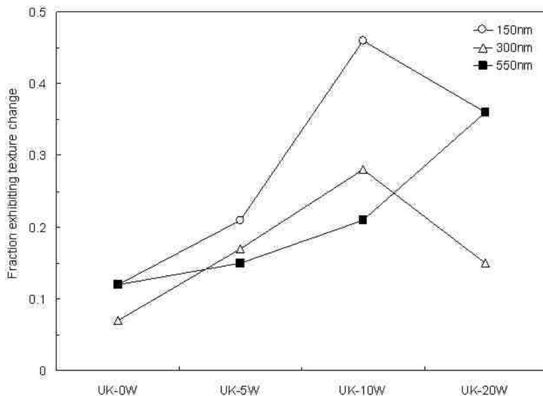
Figure 9.7 The plot shows the relationship between fraction exhibiting texture change during annealing and bias power of UK-150nm, UK-300nm, and UK-550nm films. With a given film thickness, fraction exhibiting texture change increased with the applied bias power increasing, except the UK-20W-150nm and UK-20W-300nm films. (Note: Fraction exhibiting texture change of Semicon films was 0.48, higher than all UK films.)
