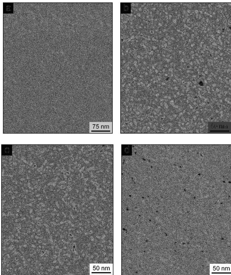
Figure 5.3 Microstructure of PdNi films dealloyed with surfactants and ultrasonic agitation for (a) 0 min (as-deposited), (b) 15 min, (c) 30 min and (d) 60 min. Grain size of the as-deposited PdNi film was \sim 20 nm. Nanoporosity was uniform and as small as 5 nm in size (for np-PdNi films dealloyed for 30-60 min).
