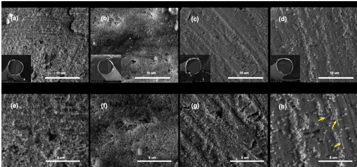
Figure 2.9 SEM images of lithium-ion deposition at 125 μm Ni micro-electrode at different concentration (a) and (e) 0.5 M, (b) and (f) 1.5 M, (c) and (g) 2 M, (d) and (h) 4 M LiClO 4 -PC by LSV, potential step from 1 V to -0.35 V vs. Li + /Li at 23 °C and scan rate is 20 mV s -1 .
