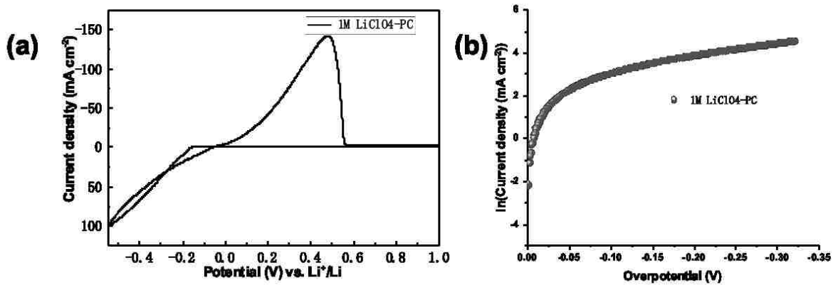
Figure 2.4 (a) Cyclic voltammety results for the 125um Ni micro-electrode. Scan rate is 100 mV s -1 from 1 V to -0.35 V at 23°C. (b) Tafel plot.
