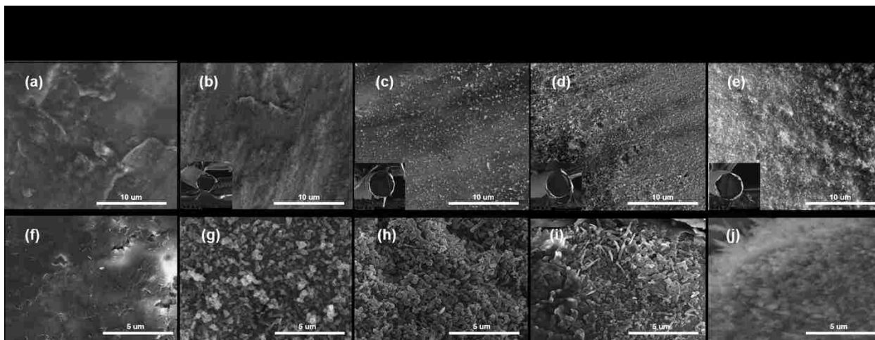
Figure 2.6 SEM images of lithium-ion deposition at 100 \mu\text{m} micro-electrode in (a) 1.2 M LiFSI-TEP-BTFE, (b) 1 M LiPF 6 -PC, (c) 1 M LiTFSI-PC, (d) 1 M LiFSI-PC, and (e) 1 M LiClO 4 -PC by LSV, potential step from 1 V to -0.35 V vs. Li + /Li at 23 °C and scan rate is 20 mV s -1 . (f)-(j) are the SEM images in the diffusion control state.
