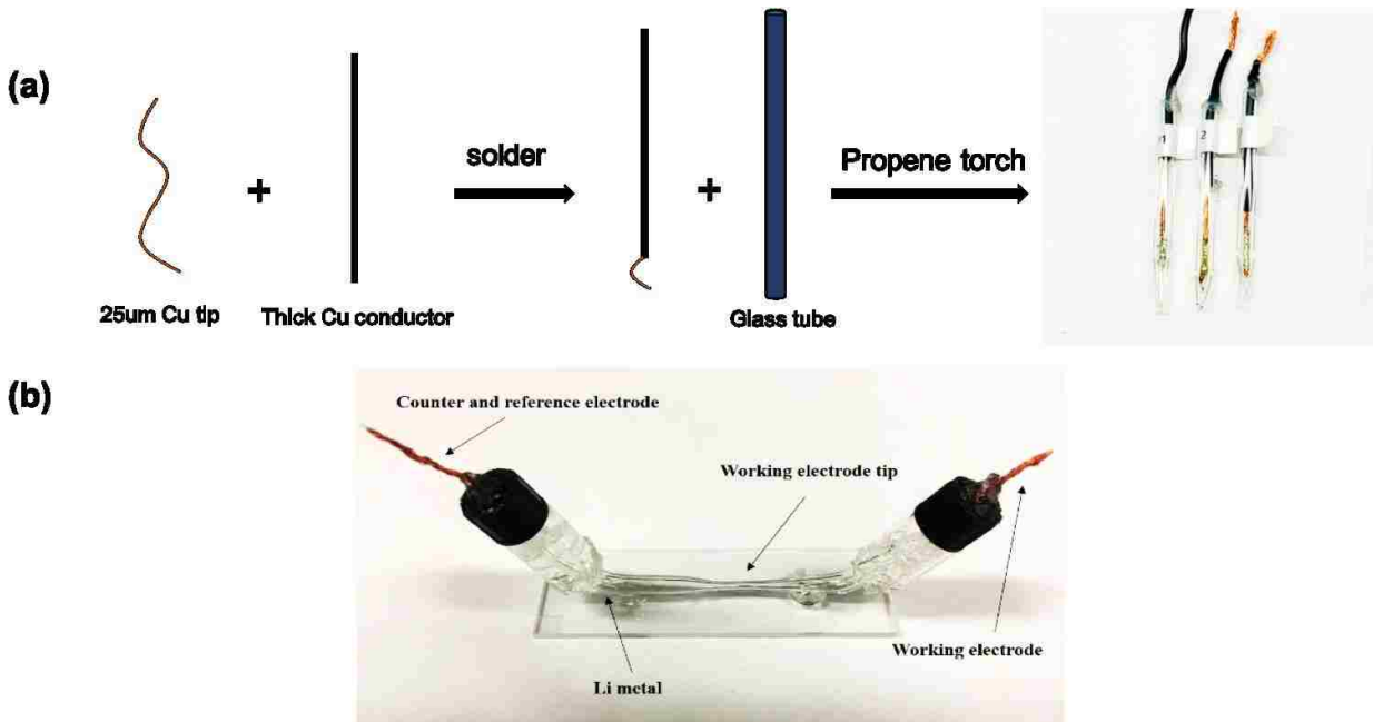
Figure 2.2 (a) Brief procedure of making 25 μm diameter micro-electrode, and (b) homemade reactor for 125 μm diameter micro-electrode to obtain SEI images.
