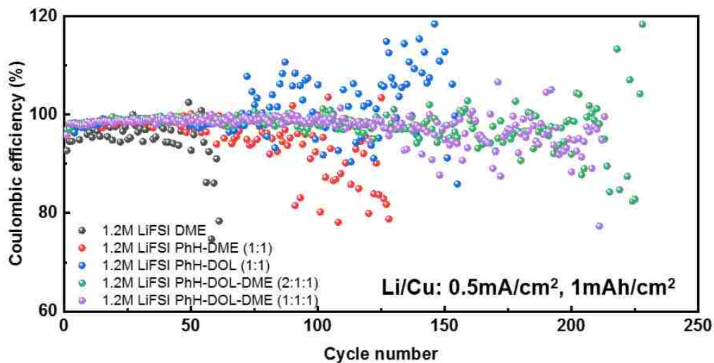
Figure 3.3 Coulombic efficiency of Li-Cu half cells used various electrolytes.
