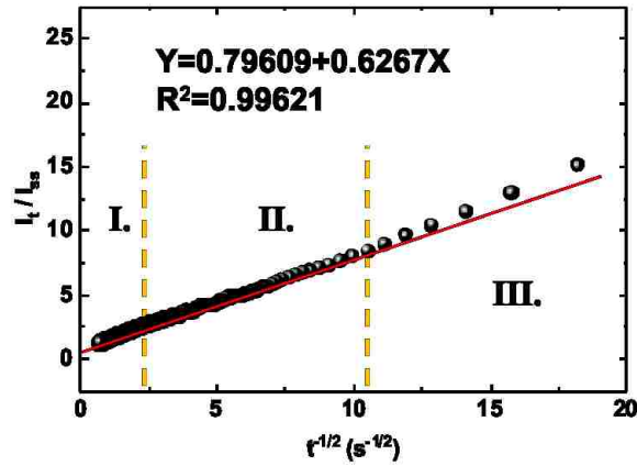
Figure 2.3 Chronoamperometry of lithium-ion deposition at 25 \mu m micro-electrode in 1 M \text{LiClO}_4\text{-PC} , 23°C, potential step from 1 V to -0.015 V vs. \text{Li}^+/\text{Li} .
