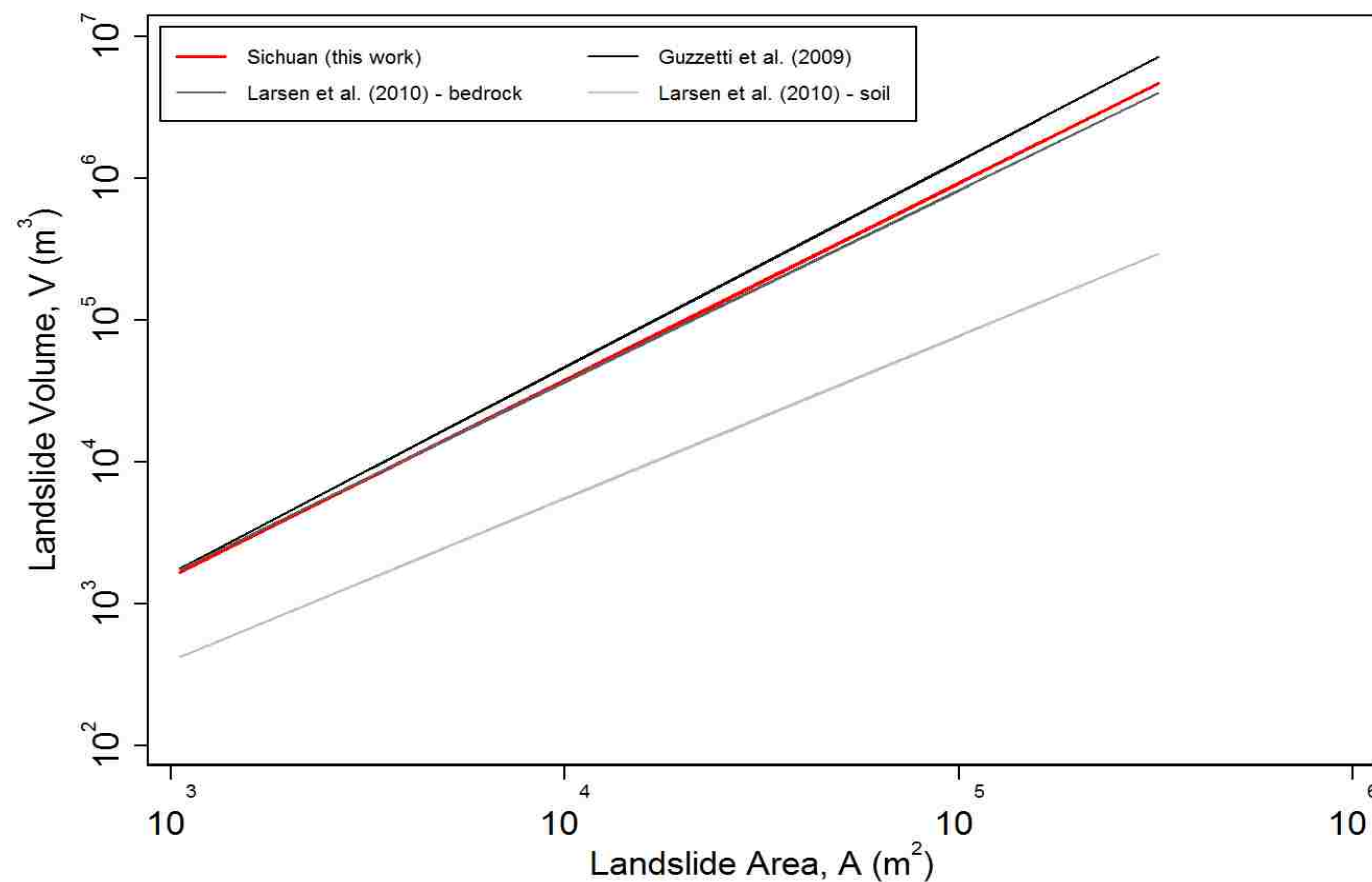
Figure 4.6: A log-log graph displaying 4 of the relationships shown in Figure 4.5 over a smaller data range, representative of the data collected in Sichuan (this work), i.e. 10^3 \text{ m}^2 \leq A \leq 10^{5.5} \text{ m}^2 . The red line represents the relationship developed for Sichuan in this work. For more detail on the data sources and the equations that describe the relationships see Table 4.1.
