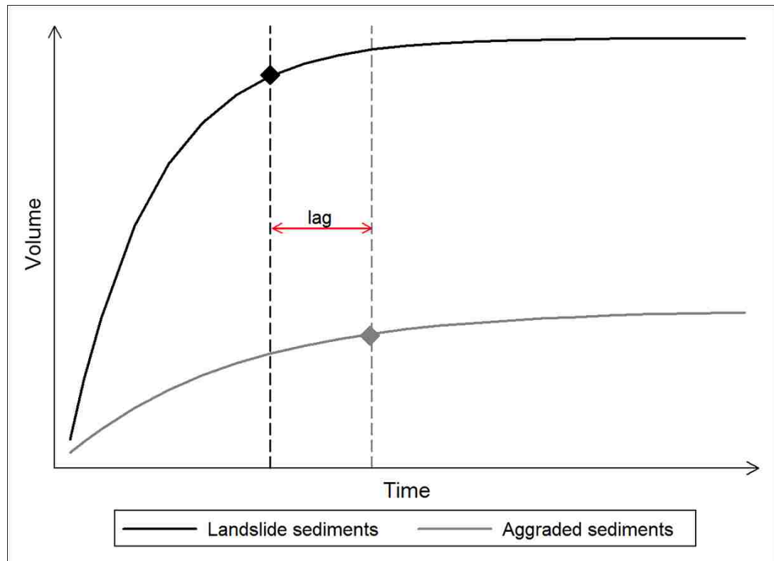
Figure 5.8: Conceptual model of the temporal changes in landslide sediment and aggraded sediment volumes post-earthquake for a typical catchment. The diamonds represent the point at which each volume is at 90% of its peak value: the lag time between these points is shown by the red arrow.
