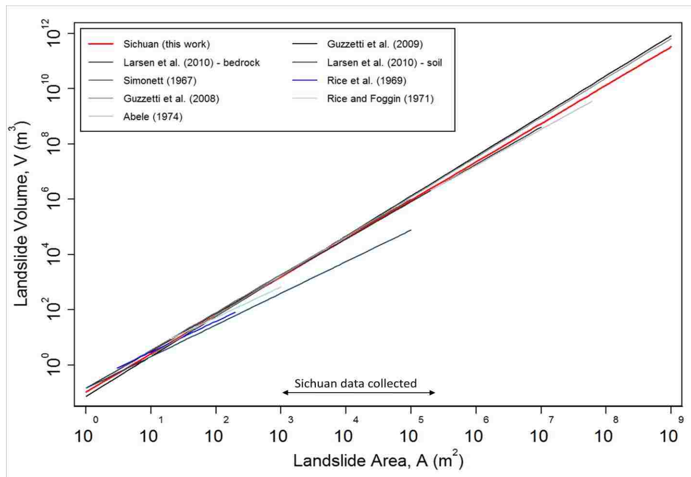
Figure 4.5: A log-log graph displaying relationships linking landslide area ( A , \text{m}^2 ) and landslide volume ( V , \text{m}^3 ) from various literature sources. The red line represents the relationship developed for Sichuan in this work. For more detail on the data sources and the equations that describe the relationships see Table 2.1 .
