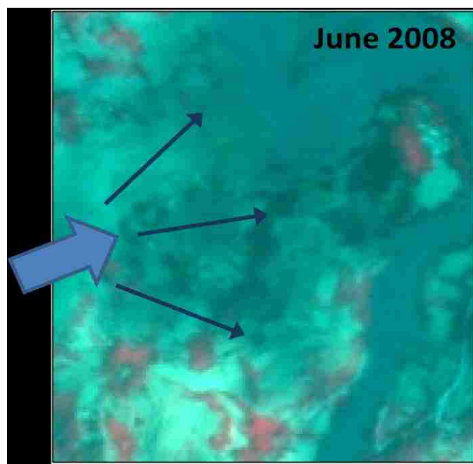
Figure 3.18: Removal of landslide deposit at Fenghuang as seen in the satellite imagery. Arrows on image S1 (left) indicate the direction of flow of material.
