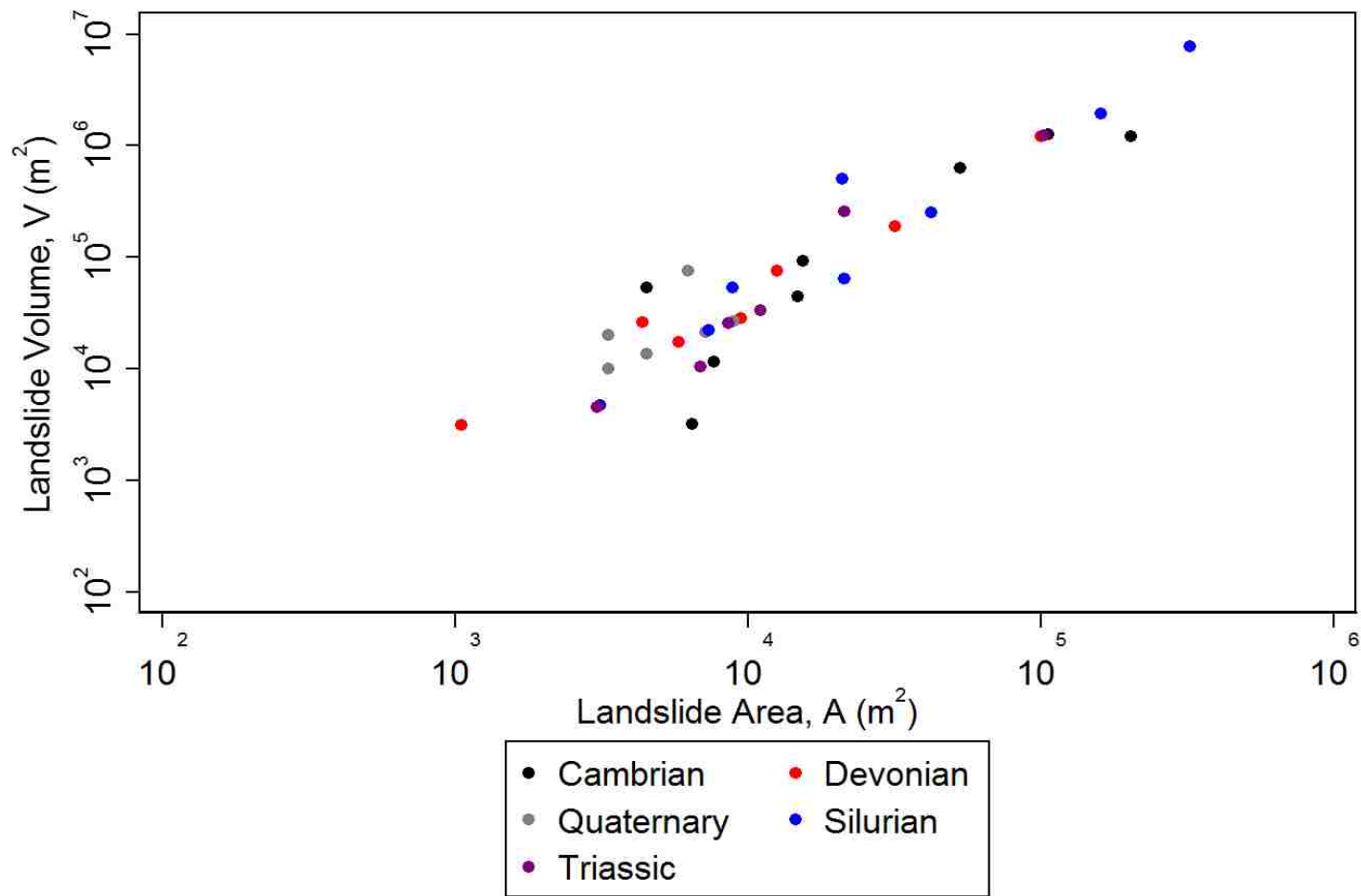
Figure 4.7: A log-log plot of the landslide area ( A, m^2 ) and calculated landslide volume ( V, m^3 ) of the 41 failures measured in-field: the failures have been identified according to geologic unit.
