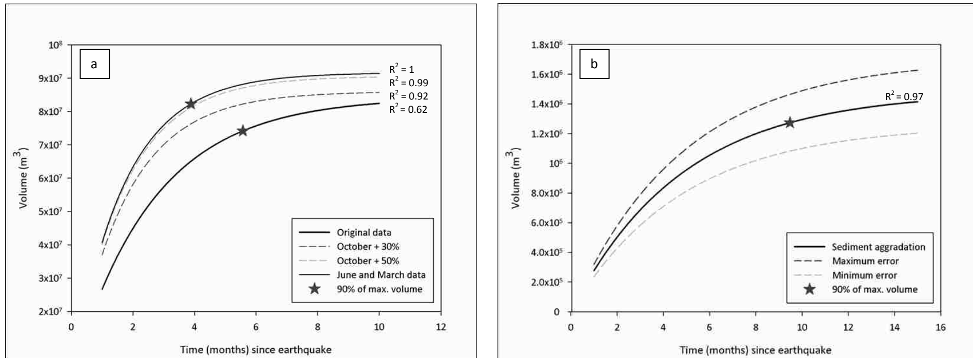
Figure 5.9: Cumulative landslide sediment volume (a) and aggraded sediment volume (b) data for the Beichuan catchment, fitted with a negative exponential decay:
