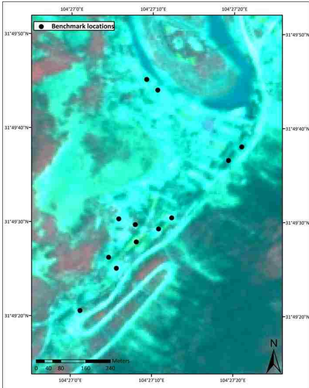
Figure 5.3: Location of the benchmarks used in photographic analysis of Beichuan town (background is the March 2009 SPOT 5 image).
