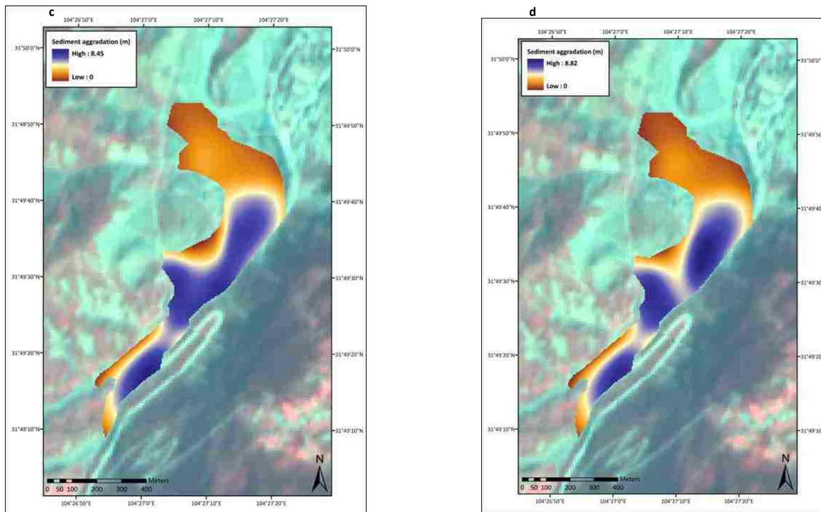
Figure 5.6: Surface models of sediment aggradation in Beichuan town: a – June 2008 (background: June 2008 SPOT 5 image); b – October 2008 (background: October 2008 SPOT 5 image); c – March 2009 (background: March 2009 SPOT 5 image); d – August 2009 (background: March 2009 SPOT 5 image).
