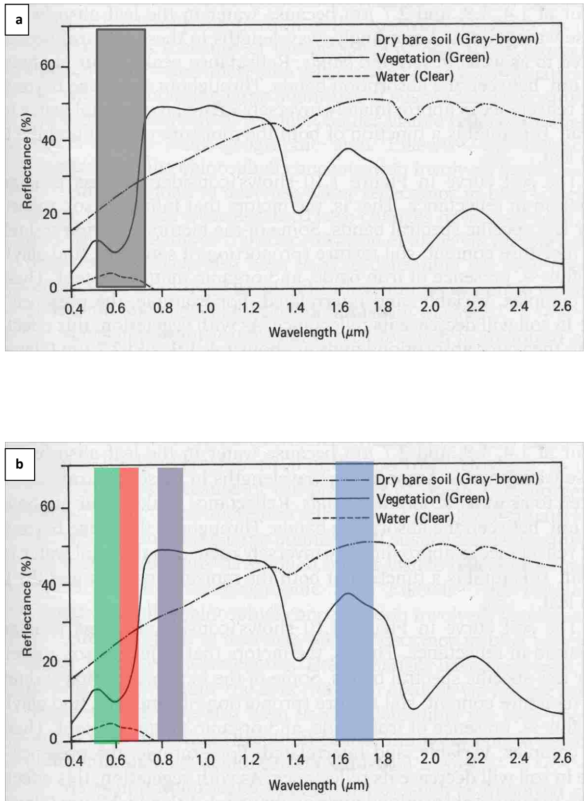
Figure 2.3: Typical spectral signatures of bare soil, vegetation and water (taken from Lillesand and Keefe, 2004). a: The SPOT 5 panchromatic band is shown in grey; b: The SPOT 5 multispectral bands are shown as follows: Green = Green; Red = Red; Purple = NIR; Blue = MIR.
