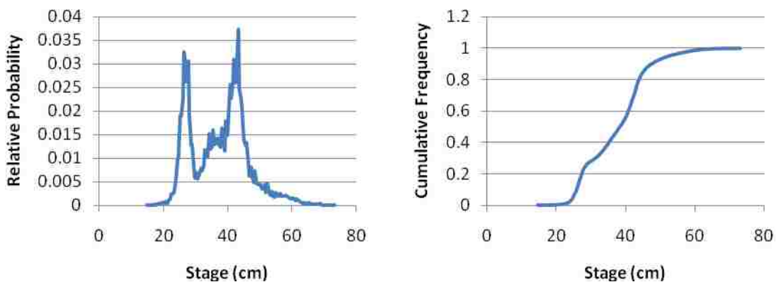
Figure 4.11: Relative probability and cumulative frequency of stage for the Winter and Spring period (November 2009 – May 2010).
