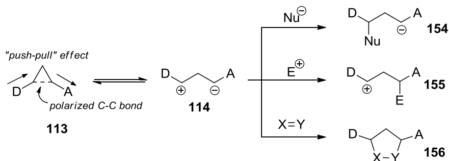
Figure 1.8. Reactions of activated vicinal DA cyclopropanes.
