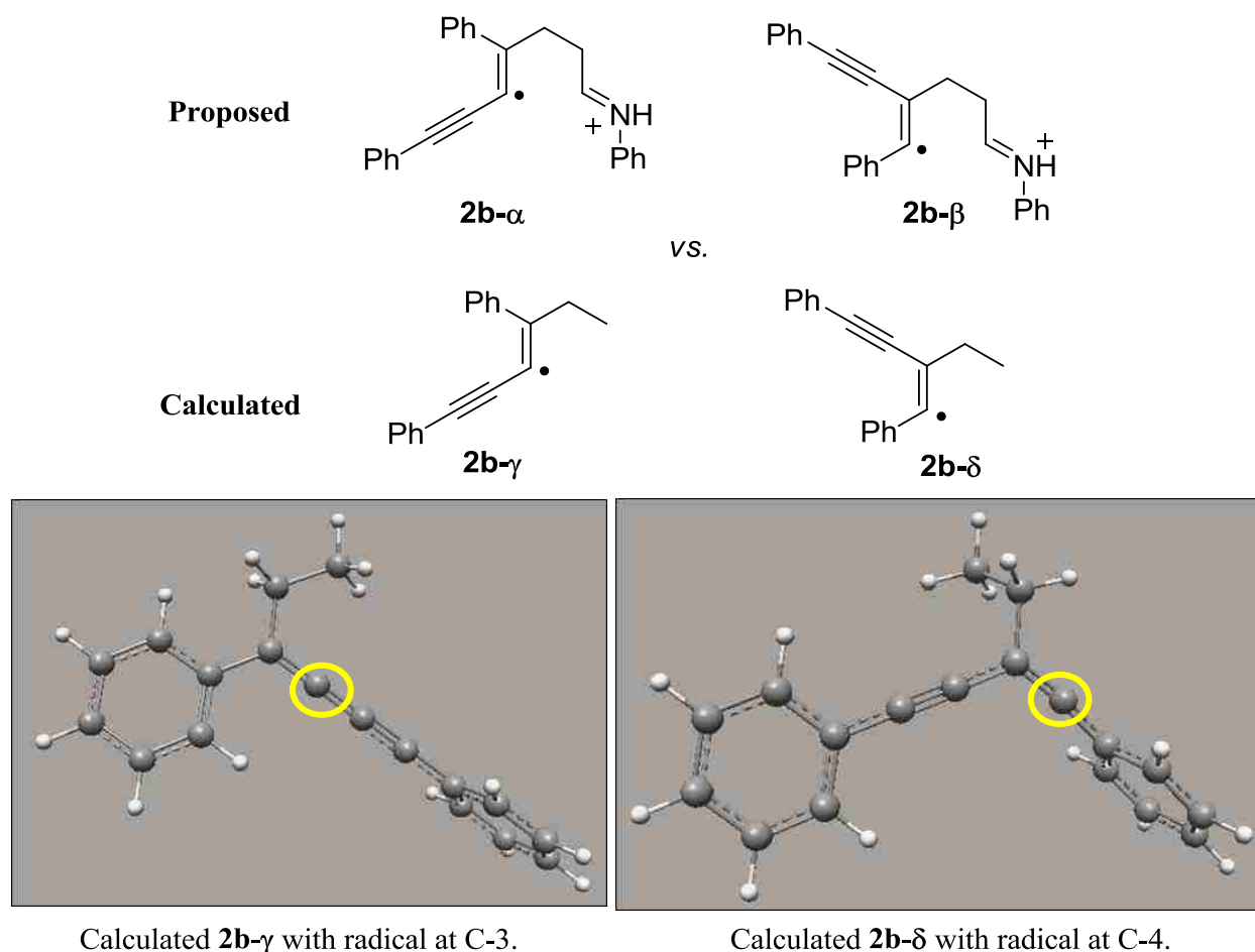
Figure 2.4. DFT calculations for the observed selectivity of diyne 2b .
