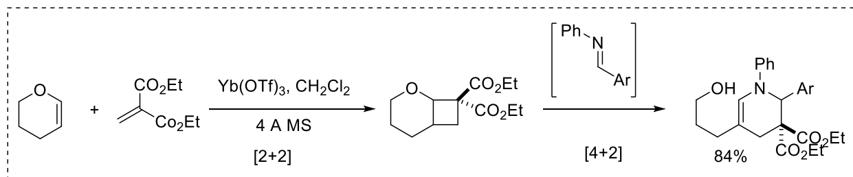
Scheme 1.22. Formal [2+2+2] Cycloaddition.
