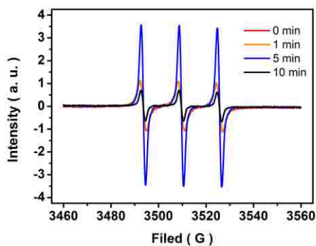
Figure 2.4.10c. Control experiment of addition of 1a
