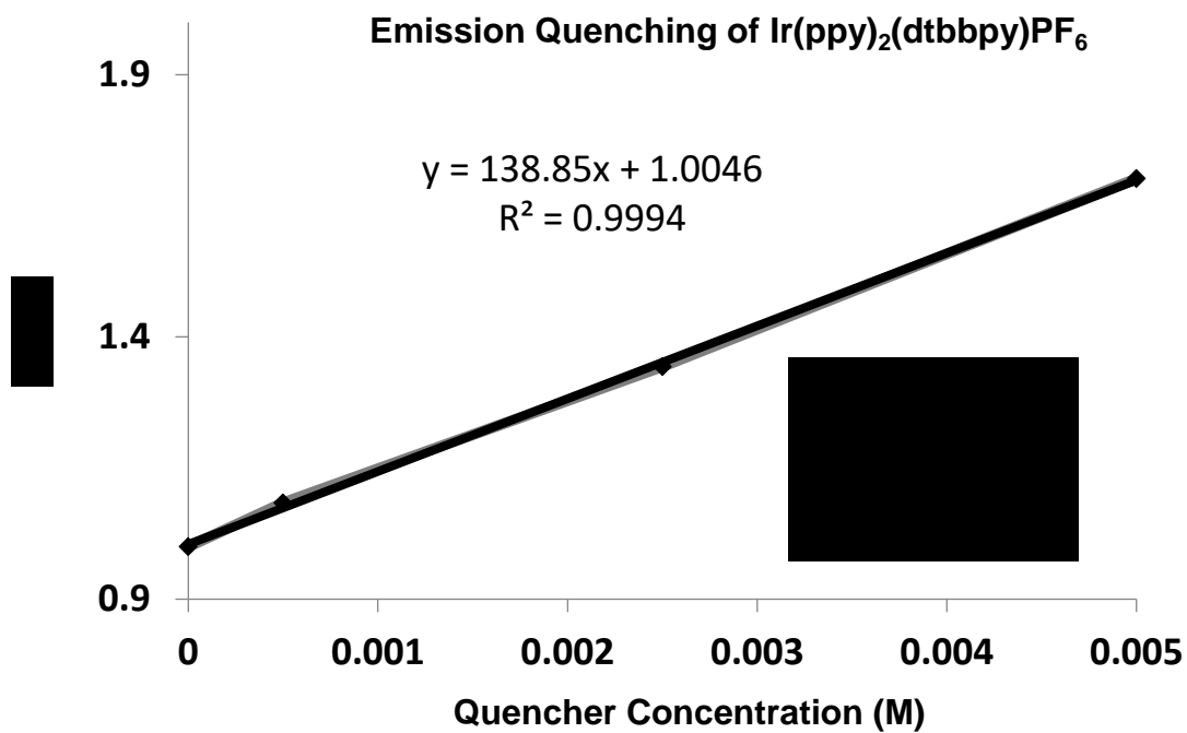
Chart 3.1a Using N -cyclobutylaniline to quench Ir(ppy) 2 (dtbbpy)PF 6 .
