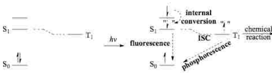
Figure 1.2. Different Pathways of Photoexcited Molecules.
