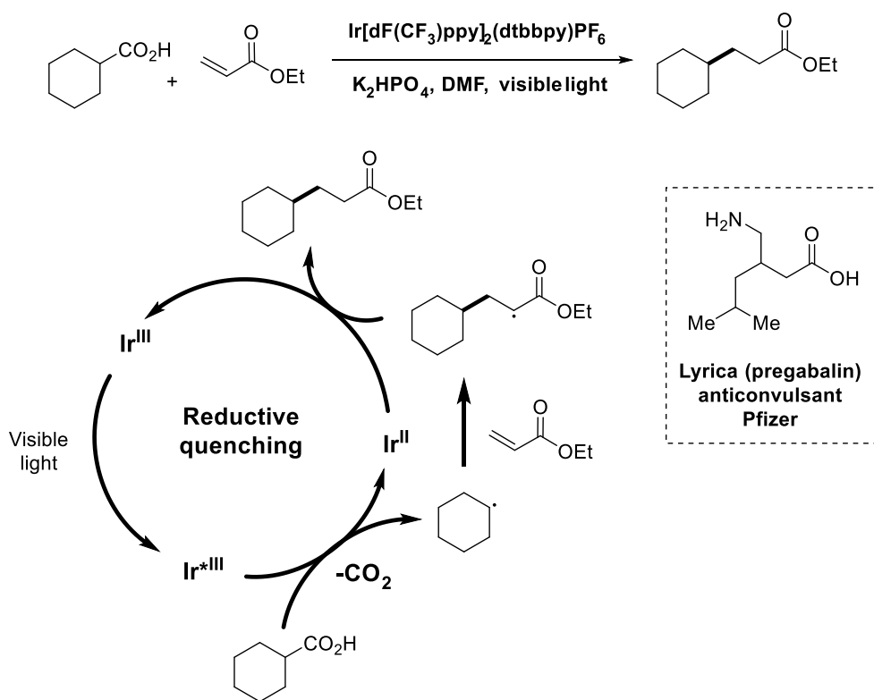
Scheme 1.6. Photoredox Catalyzed Radical Michael Addition Reaction.
