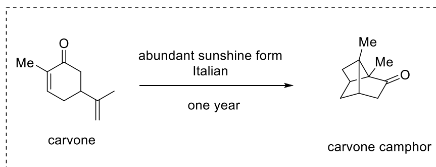
Figure 1.1. The Synthesis of Carvone Camphor under Sunlight.
