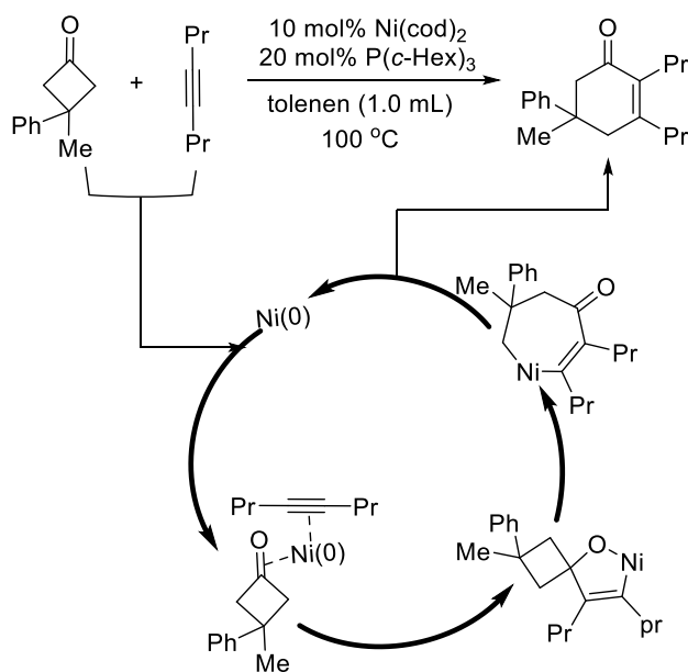
Scheme 1.16. Nickel Catalyzed [4+2] Cycloaddition of Cyclobutanones and Alkynes.
