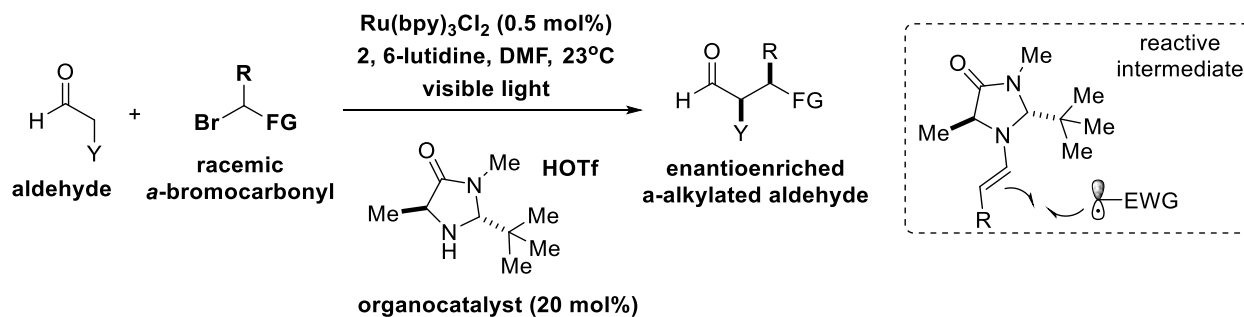
Scheme 1.1. Direct Asymmetric \alpha -Alkylation of Aldehydes under Photoredox Catalysis.
