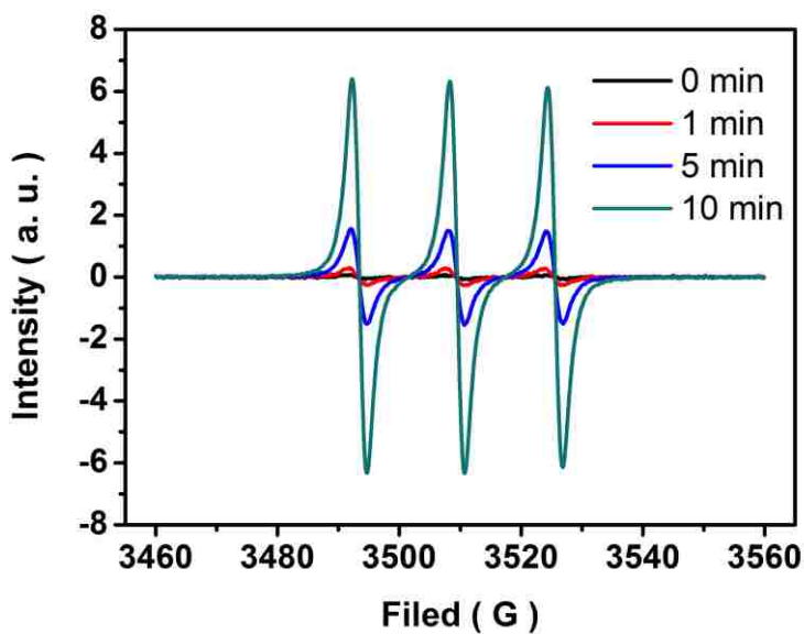
Figure 2.4.4. Trapping of ^1\text{O}_2 by TEMP without cyclobutylaniline 1a .
