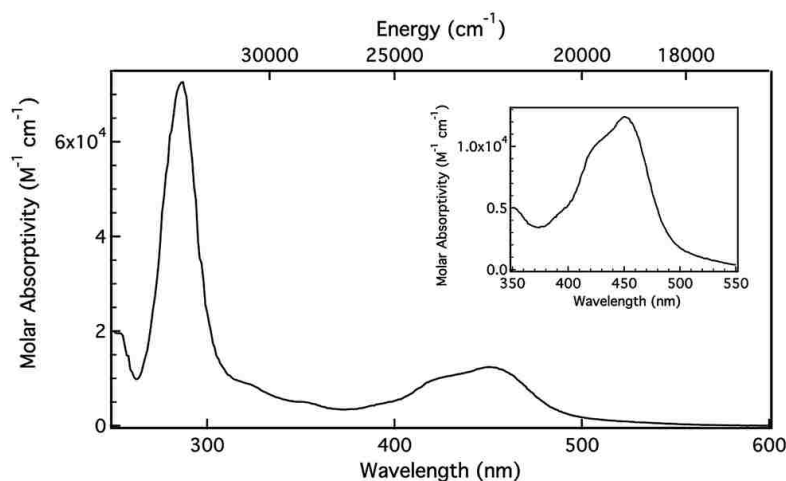
Figure 1.3. Absorption spectrum of Ru(bpy) 3 (PF 6 ) in CH 3 CN.
