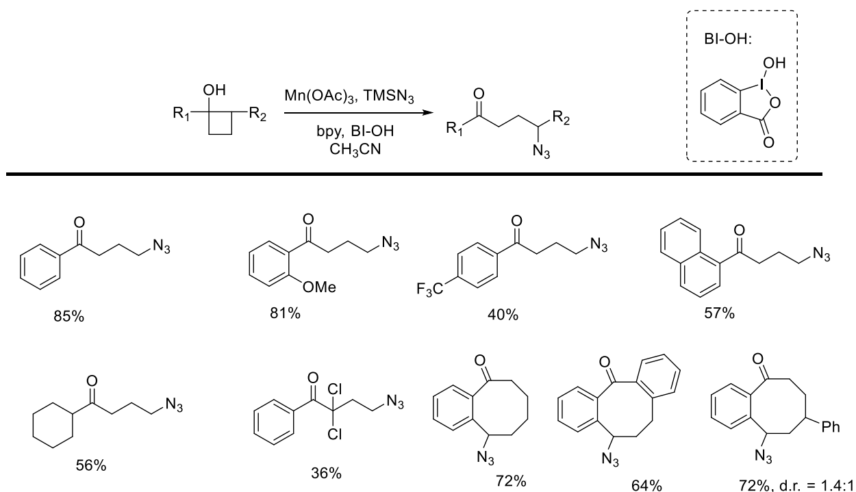
Scheme 1.20. Cyclobutanol Ring Opening for Azidations.
