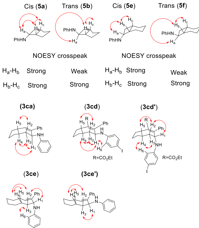
Chart 2.4 Diastereomer Identification.
