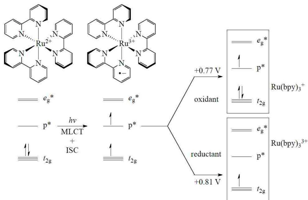
Figure 1.4. Depiction of working protocol of Ru(bpy) 3 (PF 6 ) 2 .
