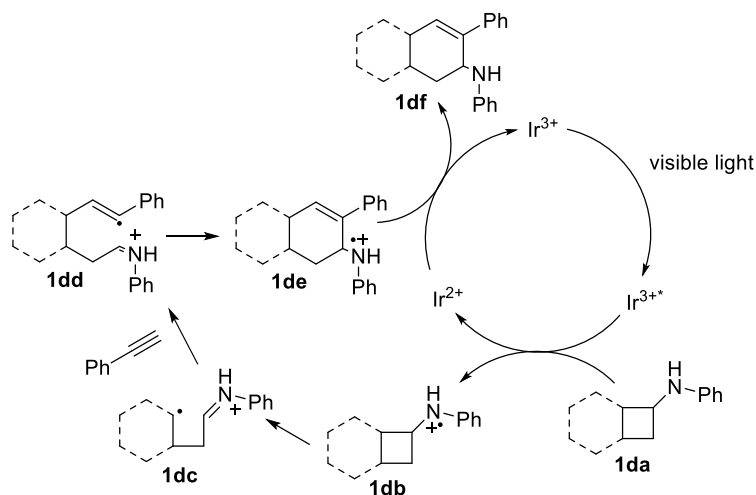
Scheme 2.2. Proposed Reaction Mechanism.
