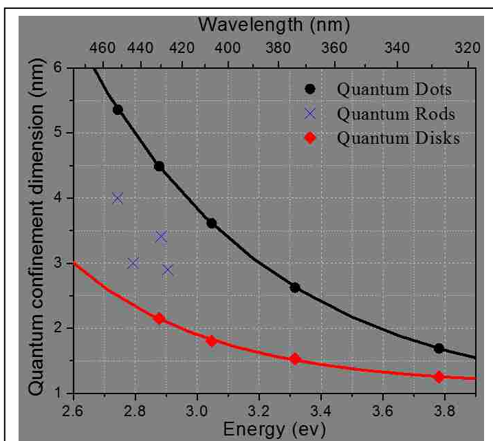
Figure 4-7. Quantum confinement dimension versus the first excitonic peak for CdS quantum dots, rods, and disks.
