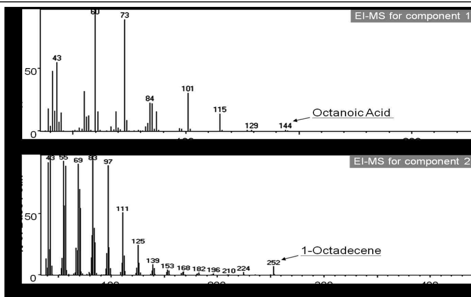
Figure 2-9. Electron ionization-mass spectra (EI-MS) of the 1 st and 2 nd component in the GC trace.
