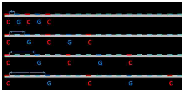
Figure 3.2 Schematic of electrode configurations for four different edge-to-edge gap conditions, 4, 12, 20 and 28 \mu\text{m} , in which two electrodes are shorted as the generator (G) and three alternating electrodes are shorted as the collector (C).
