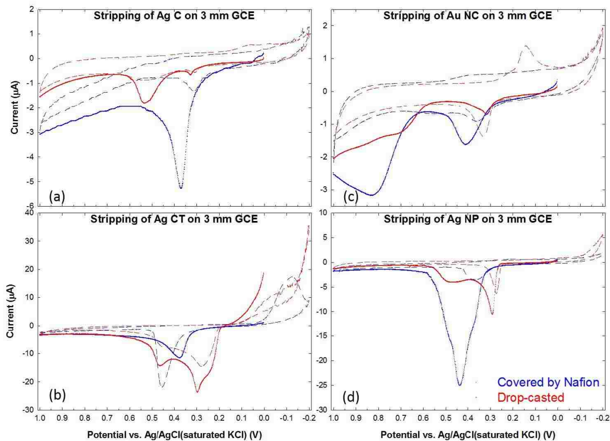
Figure 6.4 Anodic stripping voltammogram of nanoparticles drop casted on electrode surface with (blue) and without (red) Nafion coverage in surface in 0.1 M \text{NaNO}_3 . The modified electrodes were swept from 0 V \rightarrow 1.0 V \rightarrow -0.2 V \rightarrow 1.0 V at 0.05 V/s vs a Ag/AgCl (saturated KCl) reference electrode. The first sweep in each voltammogram is label as solid lines and the following segments are shown in dashed lines: (a) Ag Cs; (b) Ag CTs; (c) Au NCs; (d) Ag NP
