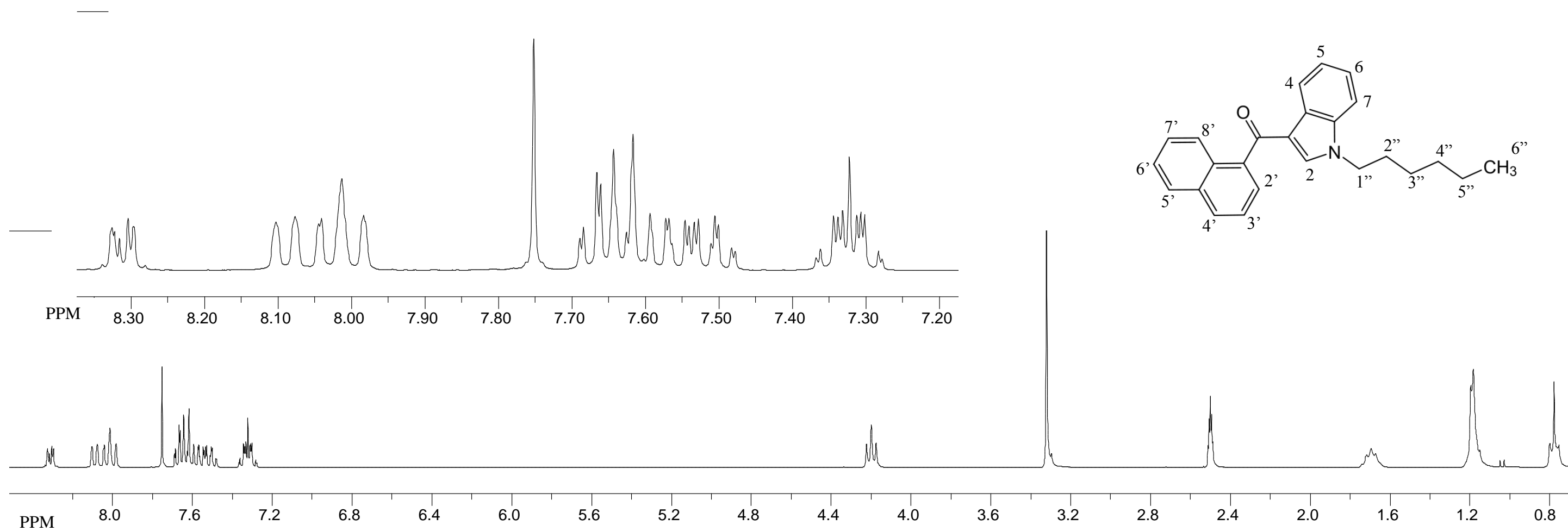
Figure14: The ^1\text{H} NMR for JWH-019. The peak assignments are as follows: H1'': 4.2 Hz, H2'': 1.7Hz; H3'', H4'', H5'': 1.18 Hz; H6'': 7.78 Hz; H-2: 7.75 Hz; H4: 8.3, 8.32 Hz; H5, 6, 7, 2', 7' 7.47-7.70 Hz; H3', 6':
