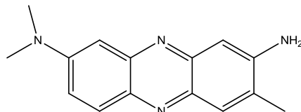
Figure 9: Neutral red contains an amine that could form a possible Schiff base with JWH-019.
