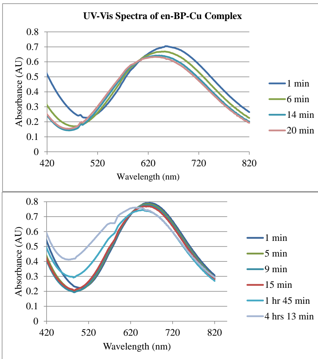
Figure 24: UV-Vis spectra of en-BP Cu complex when en-BP product was left in solution. In both experiments the \lambda_{\text{max}} decreased over time. For the top graph \lambda_{\text{max}} was 656 nm at 1 min, then decreased to 654 nm, then 642 nm and finally 634 nm at 20 min. A 2nd experiment was done and the results were similar. The \lambda_{\text{max}} es starting at 1 min and going up to 4 hrs are as follows: 666, 664, 660, 652, 650 and 638 nm.
