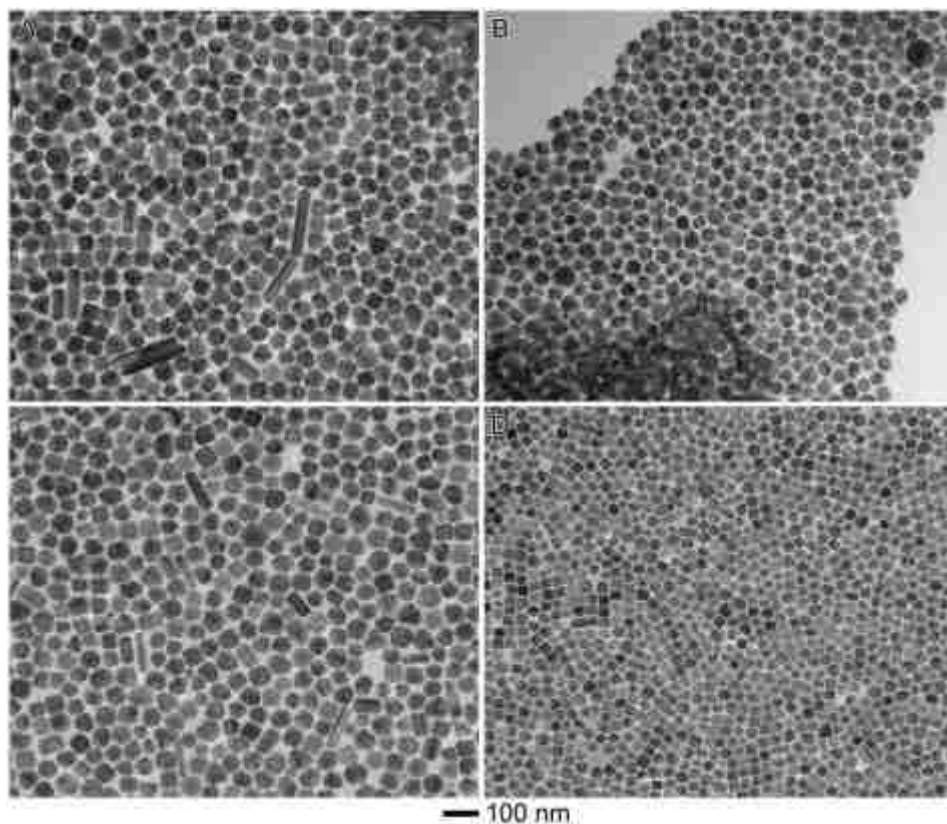
Figure S2. TEM characterization of the Cu nanoparticles synthesized by reducing \text{Cu}(\text{acac})_2 at 220\text{ }^\circ\text{C} at four different conditions: (A) no CO and formic acid; (B) CO alone (99.9% gas); (C) formic acid vapor alone (flown with Ar); (D) in the presence of both CO (99.9% gas) and formic acid vapor.
