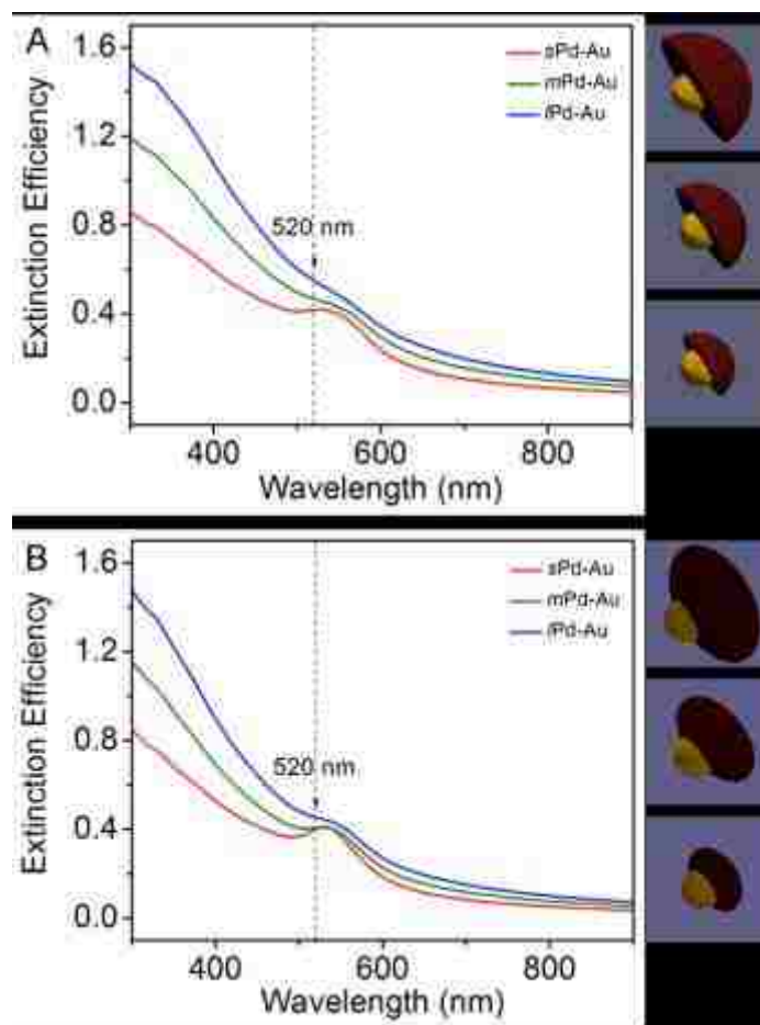
Figure S5. DDA simulation of the optical spectra of Pd-Au heterodimers with a Pd thick deposition of 4, 7, and 10 nm on a Au nanosphere with a diameter of 10 nm, denoted as sPd-Au , mPd-Au , lPd-Au , respectively, using two models: (A) a semispherical Pd shell interfacing with a spherical Au core; and (B) an ellipsoidal Pd shell carving on a spherical Au core. The right panel shows the corresponding geometries used for the simulation.
