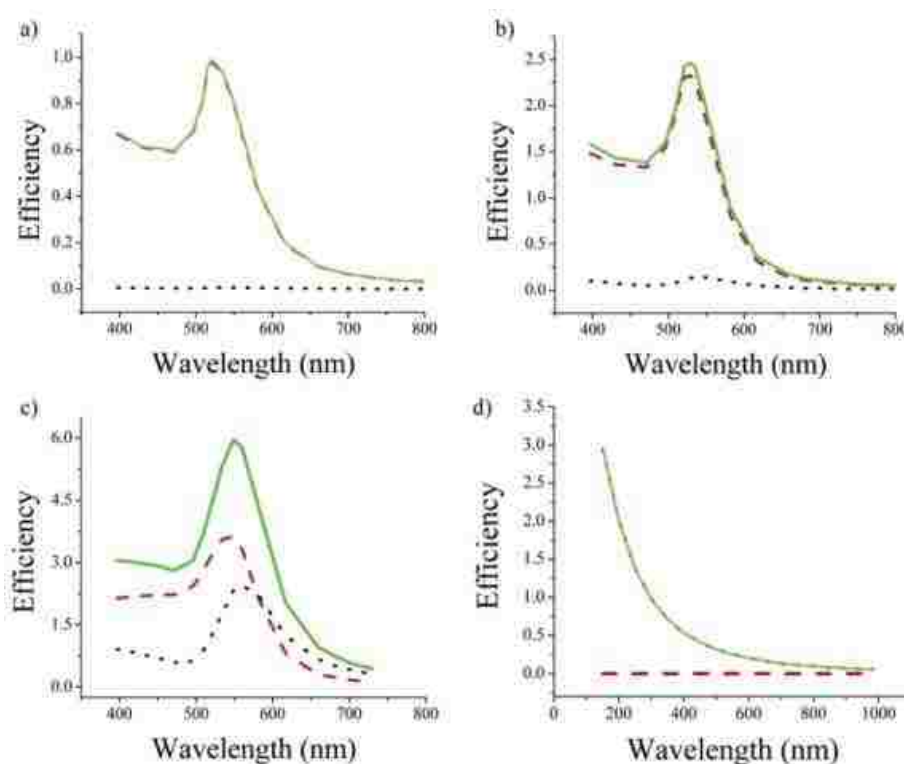
Figure 3: Calculated spectra of the efficiency of absorption Q_{abs} (red dashed), scattering Q_{sca} (black dotted), and extinction Q_{ext} (green solid) for gold nanoparticles (a) D = 20 nm, (b) D = 40 nm, (c) D = 80 nm, and polystyrene nanoparticles (d) D = 300 nm. (Reproduced by permission from reference.24 Copyright © 2006 American Chemical Society.)
