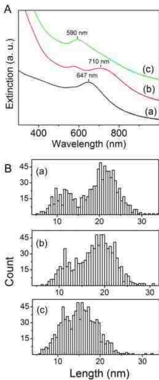
Figure 4. (A) UV-vis spectra of the AuCu 3 nanorods before (a) and after the coating of Fe 3 O 4 with a thin shell of ~2 nm (b), and a thick shell of ~5 nm (c). (B) Histograms of size distribution of the samples (a), (b), and (c).
