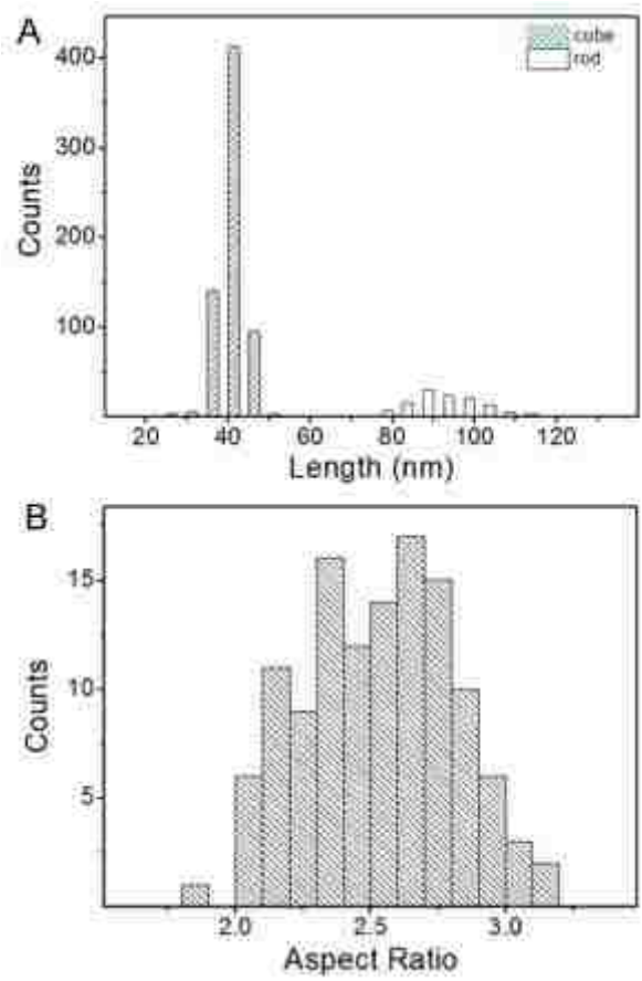
Figure S9. Size distribution analysis of the sample in Figure 6A: (A) histogram of the size distribution of Cu cubes and rods; and (B) histogram of the aspect ratios of the Cu rods.
