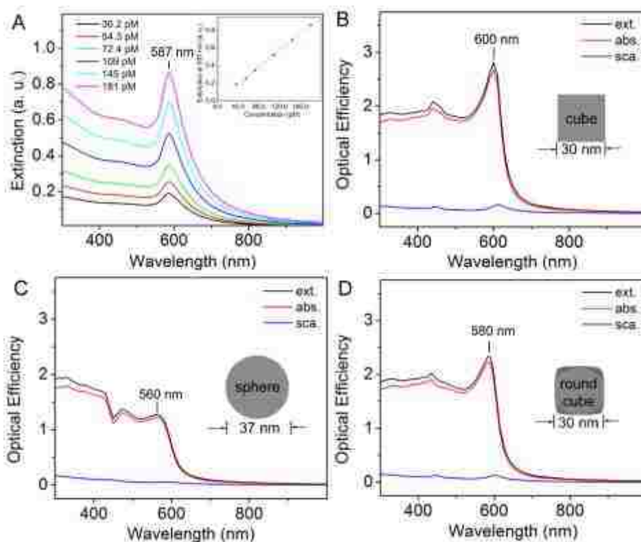
Figure 2. (A) UV-vis spectra of the Cu-SiO 2 core-shell nanoparticles at different concentrations. The inset is the plot of the extinction at LSPR maxima as a function of concentration. The red line is the linear fit of the data ( y = 4.77 \times 10^9 x , R^2 = 0.9998 ). (B) DDA simulated spectra of an isolated Cu nanocube with an edge length of 30 nm. The inset is the schematic drawing of the cross section of the nanocube. (C) DDA simulated spectra of an isolated Cu nanosphere with the same volume as the nanocube in (B). The inset is the schematic drawing of the cross section of the nanosphere. (D) DDA simulated spectra of a rounded Cu nanocube with ~2% of the total mass of the nanocube in (B) removed from the corners. The inset shows the schematic drawing of the rounded nanocube viewed from the front. All simulated spectra were calculated using water as the medium.
