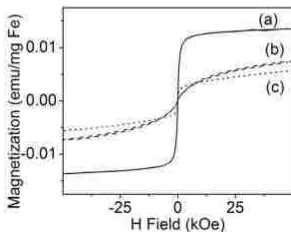
Figure 5. Magnetic measurements of (a) Fe_3O_4 nanoparticles with the size of 5 nm, (b) \text{AuCu}_3@Fe_3O_4 with a thin shell of ~2 nm, and (c) \text{AuCu}_3@Fe_3O_4 with a thick shell of ~5 nm.
