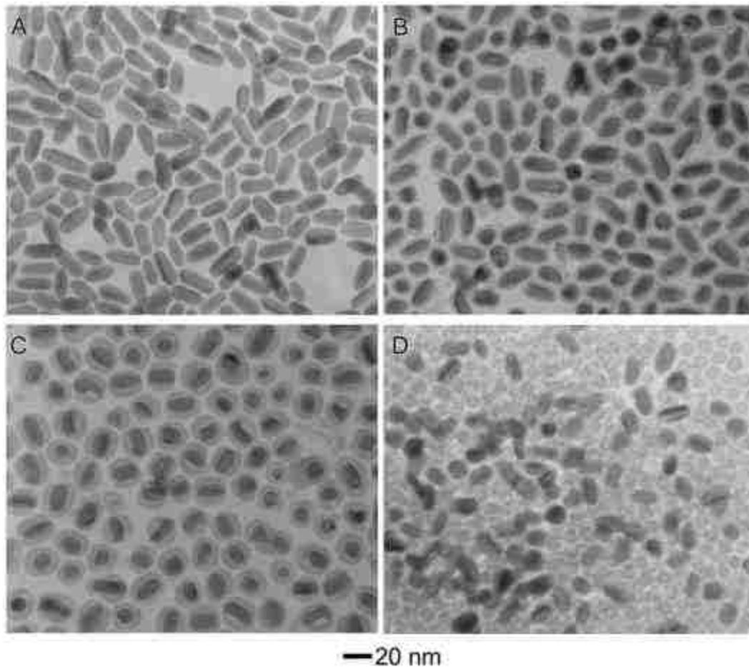
Figure 1. TEM images of controlled deposition of \text{Fe}_3\text{O}_4 shells on the \text{AuCu}_3 nanorods: (A) \text{AuCu}_3 nanorod seeds; (B) \text{AuCu}_3@Fe_3O_4 core-shell structures with a thin shell of 1-2 nm prepared at 200 °C; (C) \text{AuCu}_3@Fe_3O_4 core-shell structures with a thin shell of 6 nm prepared at 280 °C; and (D) a mixture of \text{AuCu}_3@Fe_3O_4 core-shell structures and free iron oxide particles prepared at 315 °C.
