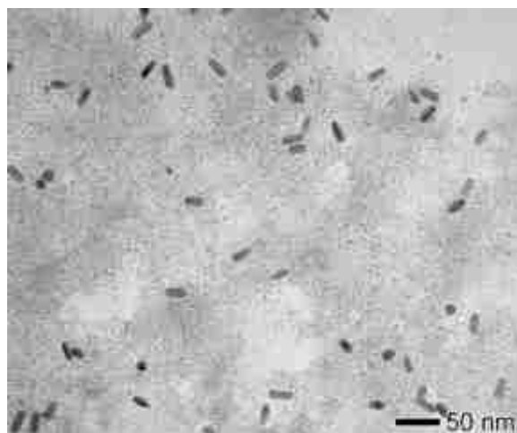
Figure S3. TEM image of the product of the AuCu 3 @NiO synthesis performed at a reaction temperature of 250°C.
