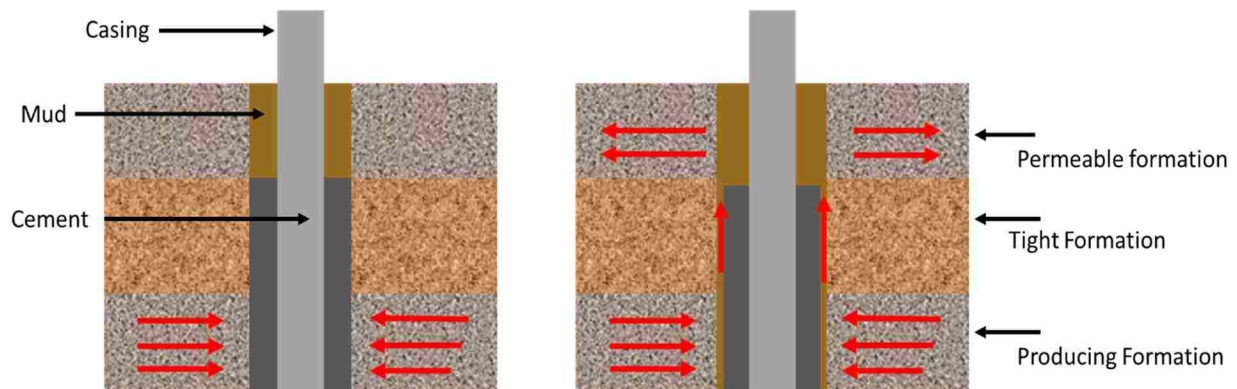
Figure 5.4: Shows how on the left as the cement shrinks a microannulus is formed around the cement allowing for fluids to flow up the wellbore, but by preventing this shrinkage as seen on the right flow up the wellbore is cut off because there is no microannulus.
