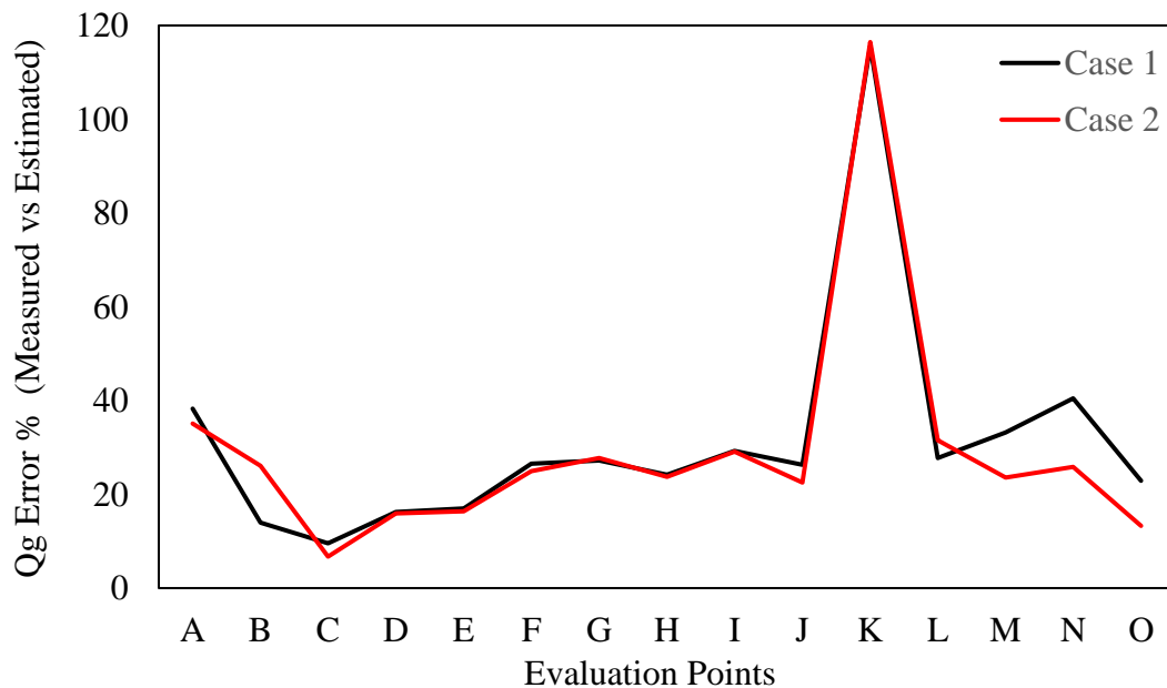
Figure 4.11 Error percentage for predicted gas flow rates for evaluation points A through O for cases 1 & 2
