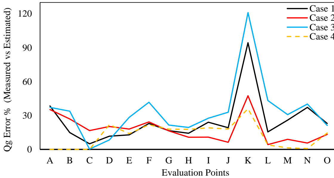
Figure 4.27 Error percentage for predicted oil flow rates for evaluation points A through O for cases 1~4
