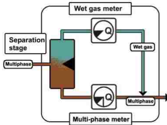
Figure 2.11 Partial separation with two measurement loop (Corneliusson 2005)
