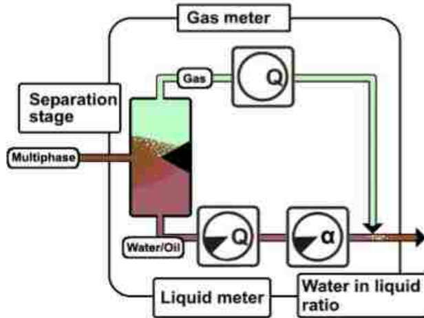
Figure 2.10 Separation type meters (Corneliusson 2005)
