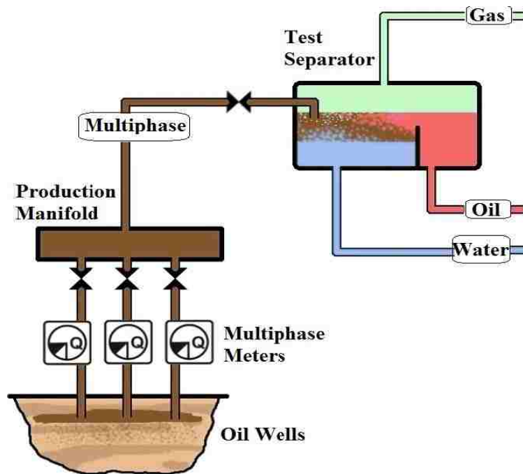
Figure 2.2 MPFMs on the flow line of each well (Corneliusson 2005)
