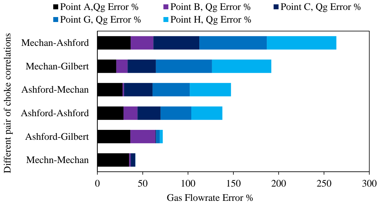
Figure 4.32 Gas flow rates error percentage vs different choke correlations for five points (A+B+C+G+H)
