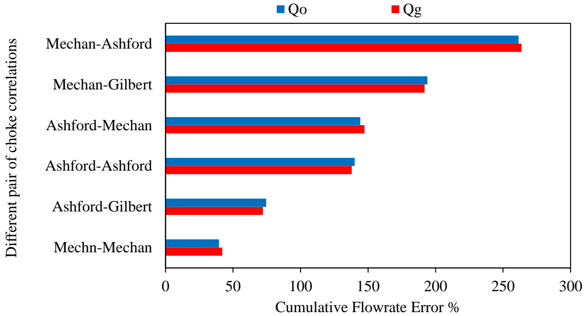
Figure 4.34 Cumulative error percentage for gas and oil flow rates vs different choke correlations for five points (A+B+C+G+H)
