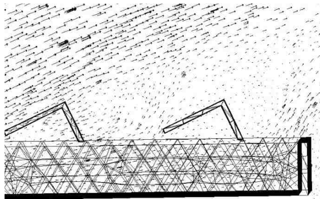
Fig. 5-5 Velocity vectors at wind attack angle of 210^\circ for vertical spacing at the same height as the parapet
