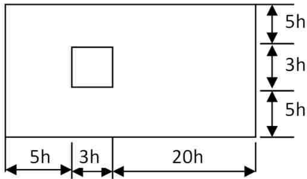
Fig. 3-4 Computational domain (horizontal layout, not to scale)
