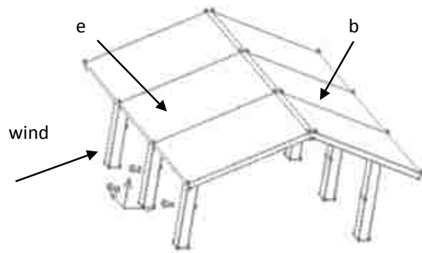
Fig. 3-1 Geometry of canopy with 0° wind attack angle
