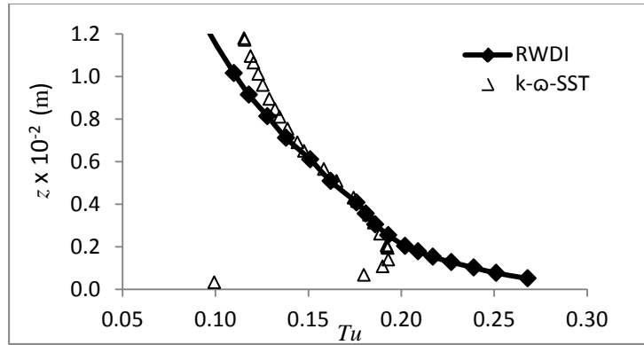
Fig. 4-3 Turbulence intensity in streamwise direction at building location, without presence of the building
