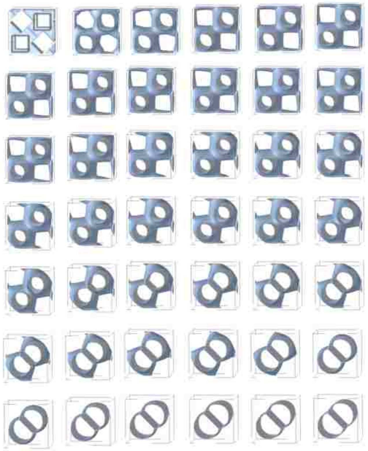
Figure 7.13: Double Hydrant evolution to a Double Cylinder.
