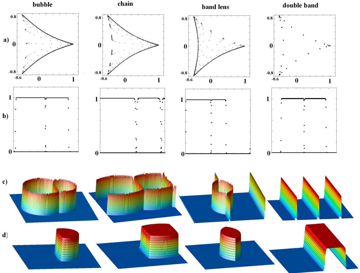
Figure 3.8: A range of plots for the standard double bubble V_1 = 0.2, V_2 = 0.1, P = 2.14 , standard chain V_1 = 0.3, V_2 = 0.2, P = 2.88 , band lens V_1 = 0.45, V_2 = 0.1, P = 2.70 and the double band V_1 = 0.33, V_2 = 0.33, P = 2.99 , where P is the perimeter. a) The plot of the field values in the complex plane. b) Cross sectional plots of the volume densities. c) Plot of the energy density, showing the position and thickness of the domain walls, as well as their general behaviour. d) Plot of the volume density.
