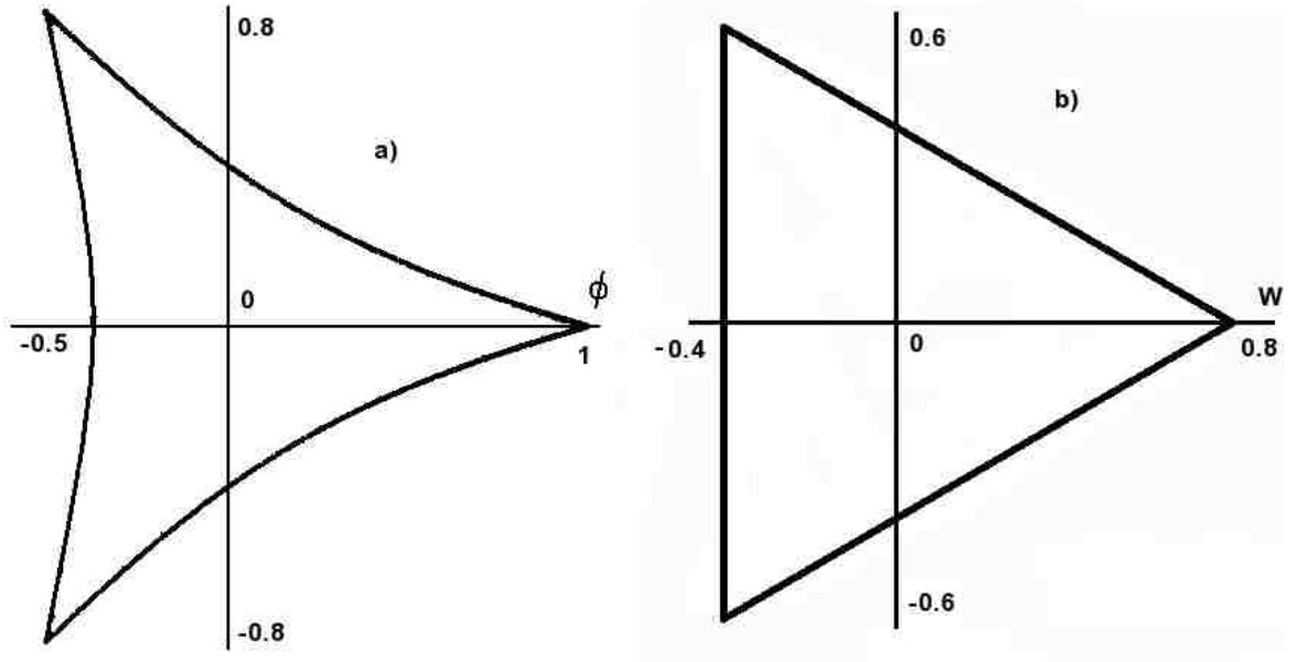
Figure 1.2: The kinks linking the three vacua in the \phi^6 model in \phi -space a) and W -space b) The three vacua are located at the corners, and the three kinks are the lines connecting the vacua. Note the scales on the two graphs are not the same
