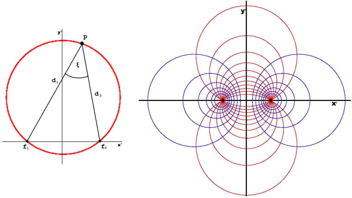
Figure 6.1: Bipolar Coordinates. (left) The red circle is a curve of constant \xi , a point is connected to the two foci, \mathcal{F}_1 and \mathcal{F}_2 . The natural logarithm of these two distances gives the \eta coordinate and the angle between them gives \xi . (right) The Apollonian circles, which characterises the constant coordinate curves here. The red circles are curves of constant \xi while the blue circles are curves of constant \eta .
