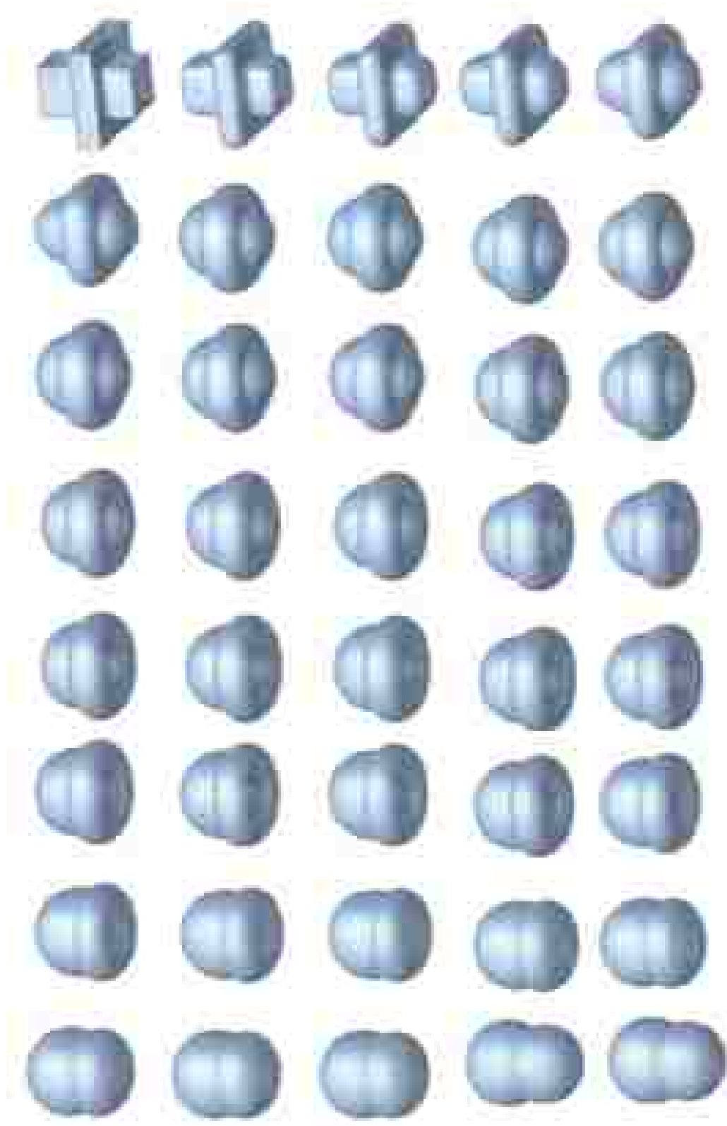
Figure 7.10: Torus Bubble evolution to a Double Bubble.
