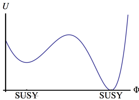
Figure 1.7: Metastable SUSY breaking. Although a locally stable SUSY breaking vacuum exists, one allows the existence of other, supersymmetric vacua elsewhere in field space.
