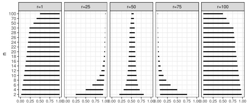
Figure 3.6: [\underline{P}, \overline{P}](X_{(r)} < Y_{(r)}) for m = 100
