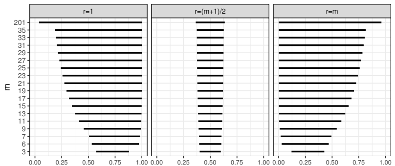
Figure 3.7: [\underline{P}, \overline{P}](X_{(r)} < Y_{(r)}) for n = 8
