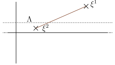
(b) The case that one of the points approaches the boundary. The second point in the bulk holds \Psi at order \ln \epsilon .
