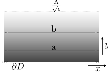
Figure 3.2: The regions of interest for the integral into the bulk. The lower line represents the boundary \partial D . a , b and \Lambda are chosen to allow the application of the approximate forms of \Psi . From the boundary up to a the lower approximation holds and from b to \frac{\Lambda}{\sqrt{\epsilon}} the upper approximation holds. In between there is no explicit form of \Psi but integrals in this region are independent of \epsilon .
