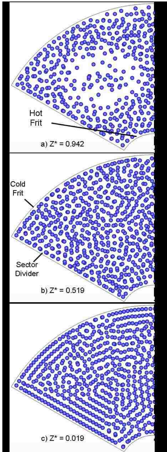
Fig. 4.26. - Plane-view images of the loaded fuel pellets at selected axial locations in the PeBR core sector (see Fig. 4.24) (pellets not to scale) [Schriener and El-Genk 2012c].
