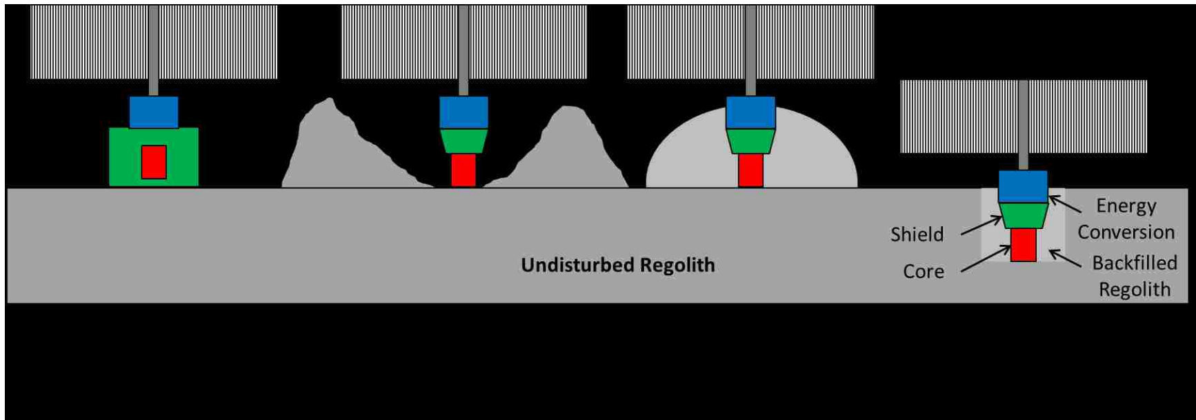
Fig. 2.3. - Placement options for lunar power reactors.
