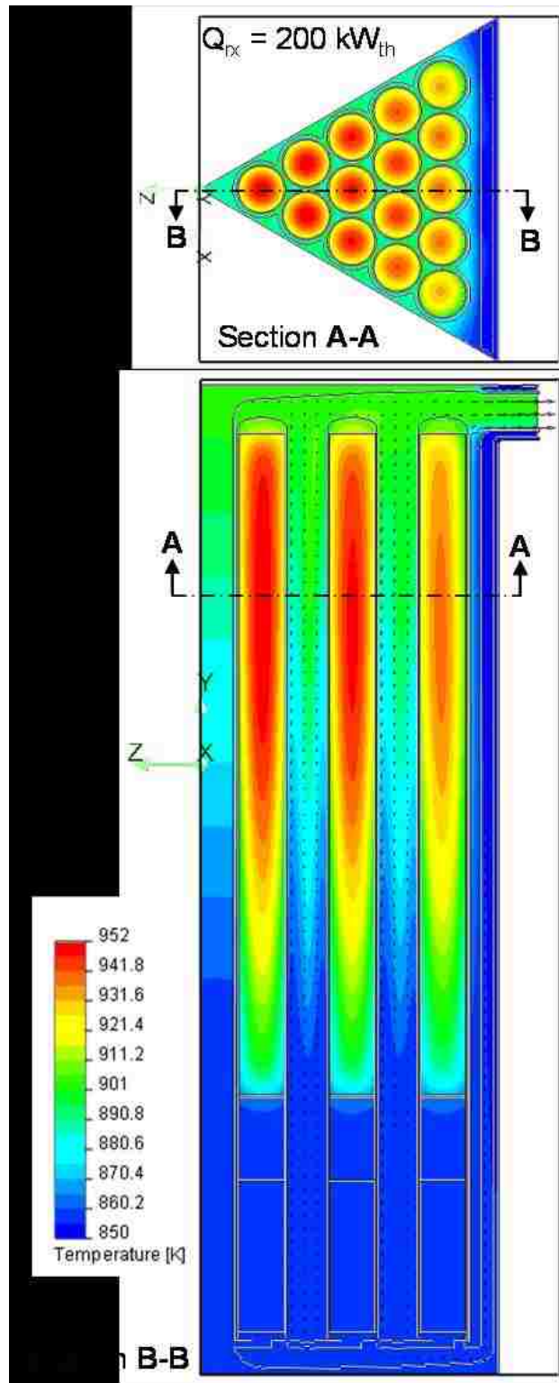
Fig. 3.31. - Calculated temperatures in a hydraulic sector of the SCoRe-N 5 reference design at 200 kW th [Schriener and El-Genk 2012a].
