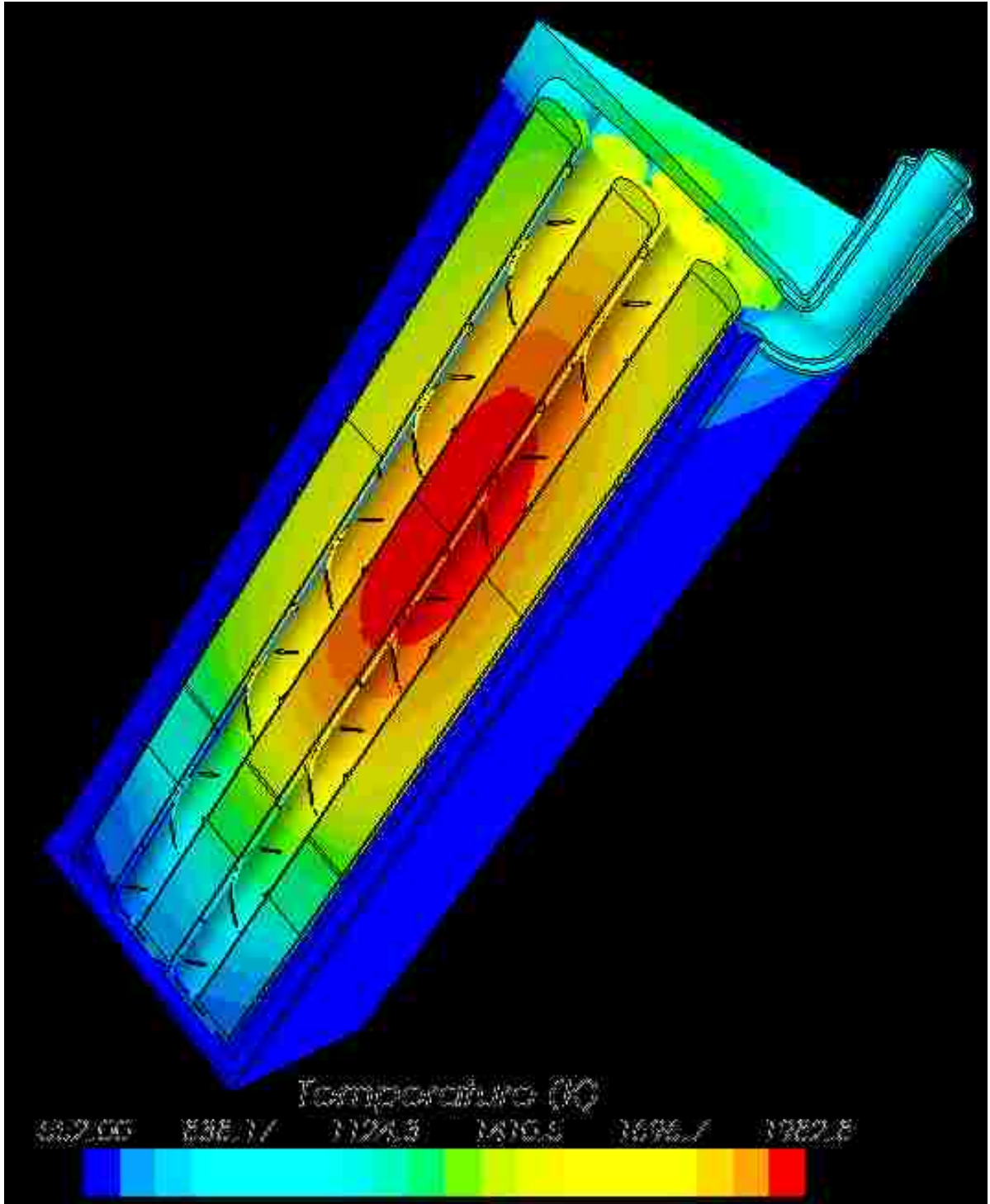
Fig. 3.41. - Perspective view of the core sector experiencing a LOC, with wire wrapped UN fuel rods a reactor power of 166.67 kW th [Schriener and El-Genk 2012b].
