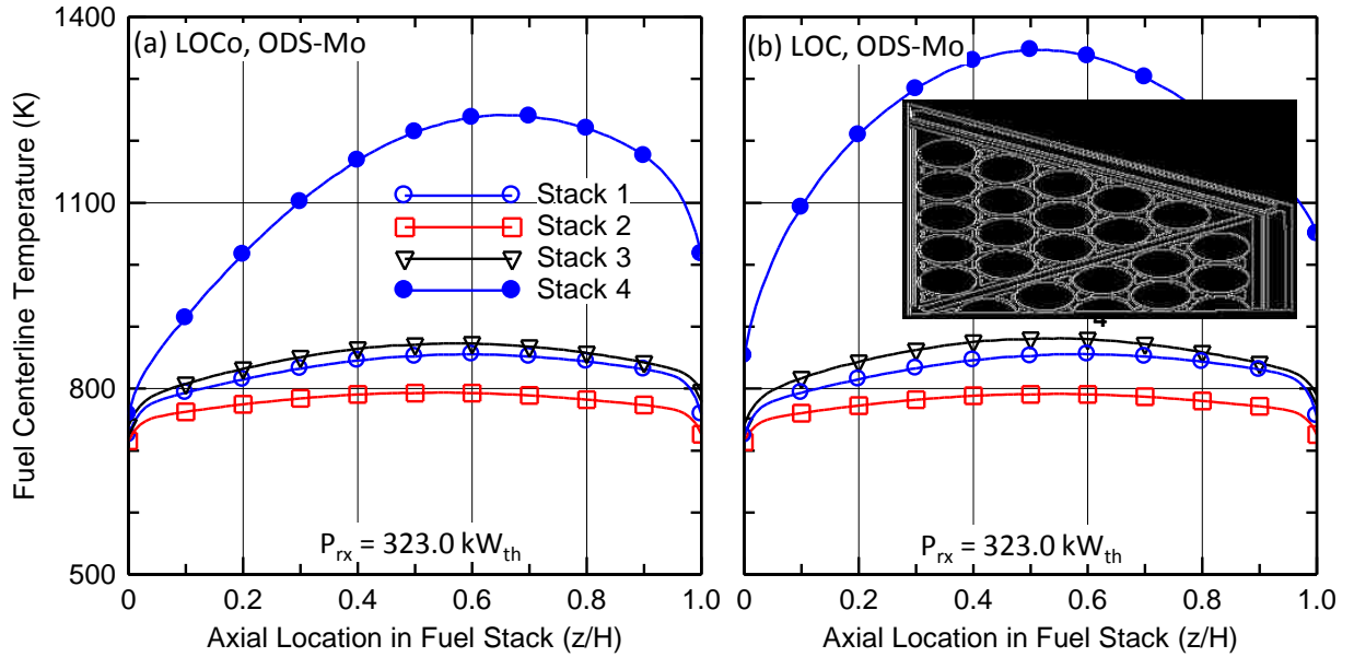
Fig. 3.56. - Calculated centerline temperatures of selected UN fuel stacks in SC-SCoRe operating at 323.0 \text{ kW}_{th} with a core sector experiencing: (a) a LOfCo and (b) a LOC [Schriener and El-Genk 2014b].
