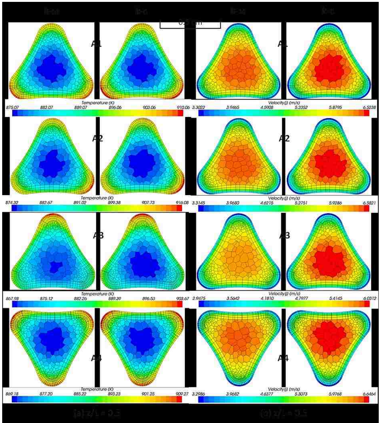
Fig. D.8. - Comparisons of the calculated temperature and velocity fields in selected liquid NaK-56 flow channels at core mid-plane using the k- \epsilon and k- \omega turbulence models with the finest numerical mesh 'a' (Table D.1) [Schriener and El-Genk 2014a].
