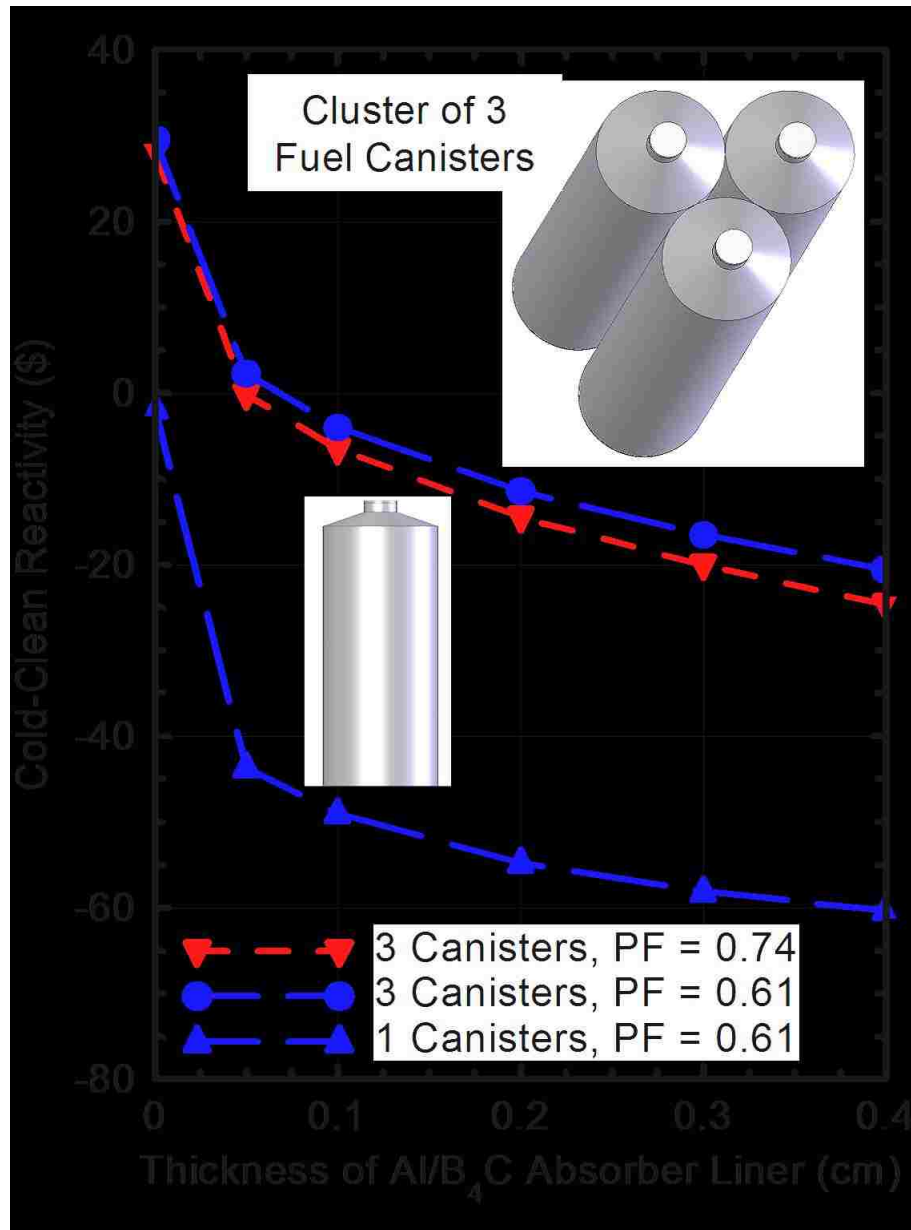
Fig. 4.18 - Criticality estimates of the canisters loaded fresh fuel pellets in the unlikely event of a launch abort accident [El-Genk and Schriener 2011].
