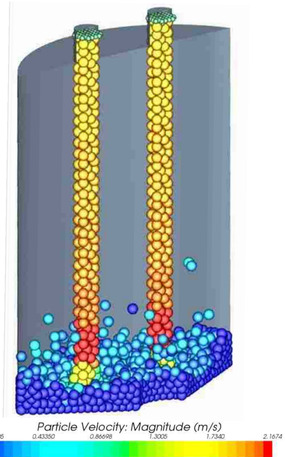
Fig. 4.19. - A PeBR core sector while being loaded with fuel, containing ~2,000 fuel pellets [Schriener and El-Genk 2012c].
