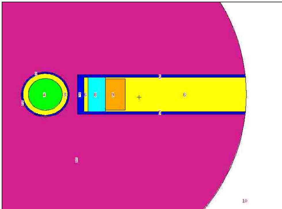
Figure 4.2.2: XY-plane view of the MCNP geometries for the NH-3 Neutron Howitzer with 15 mm \text{CaF}_2 sample inserted (as region 9).
