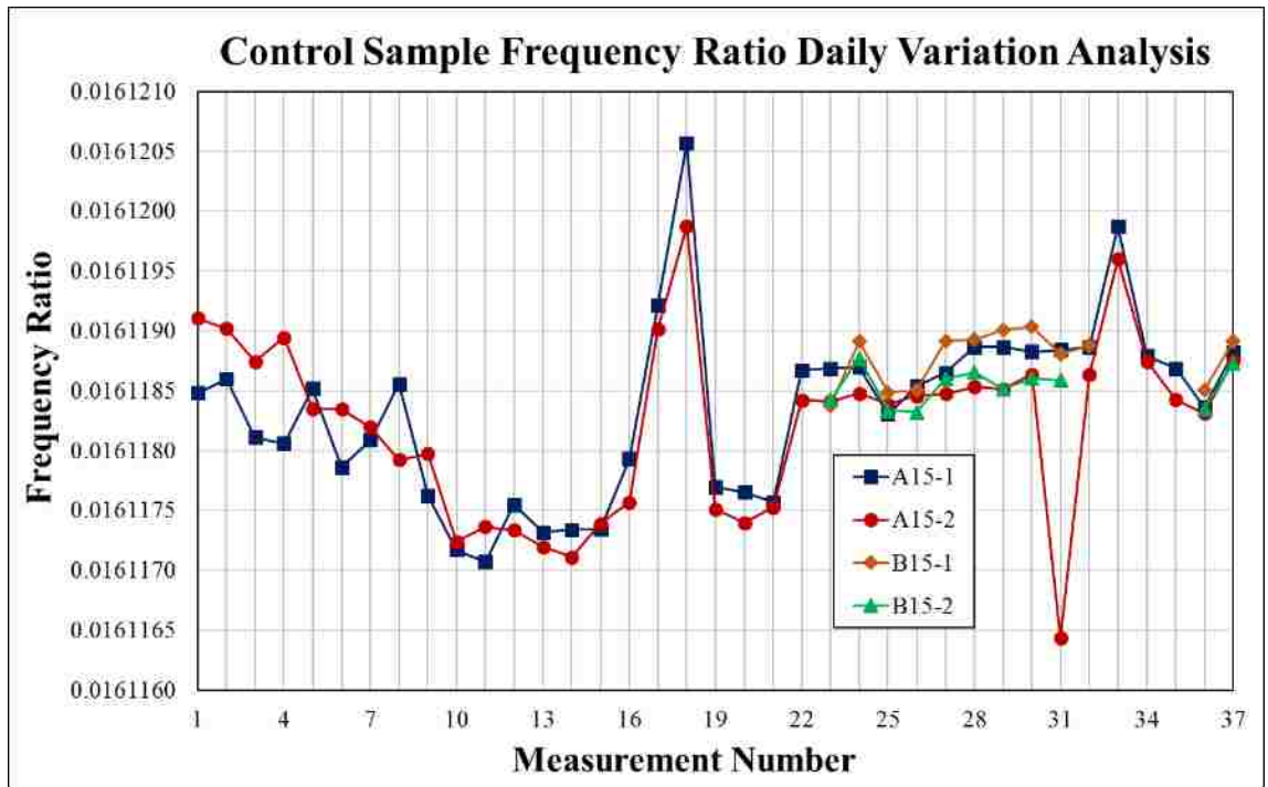
Figure 5.3.1: Variation in frequency ratio of unirradiated control samples A15-1 and A15-2, as well as the later included control samples B15-1 and B15-2. The total time period of measurements occurred between June 29, 2016 and May 5, 2017.
