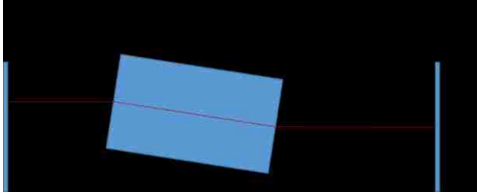
Figure 3.3.7: A simplified depiction of a laser cavity emphasizing the constant FPE angle requirement for a cavity length scan to determine the refractive index change of an FPE.
