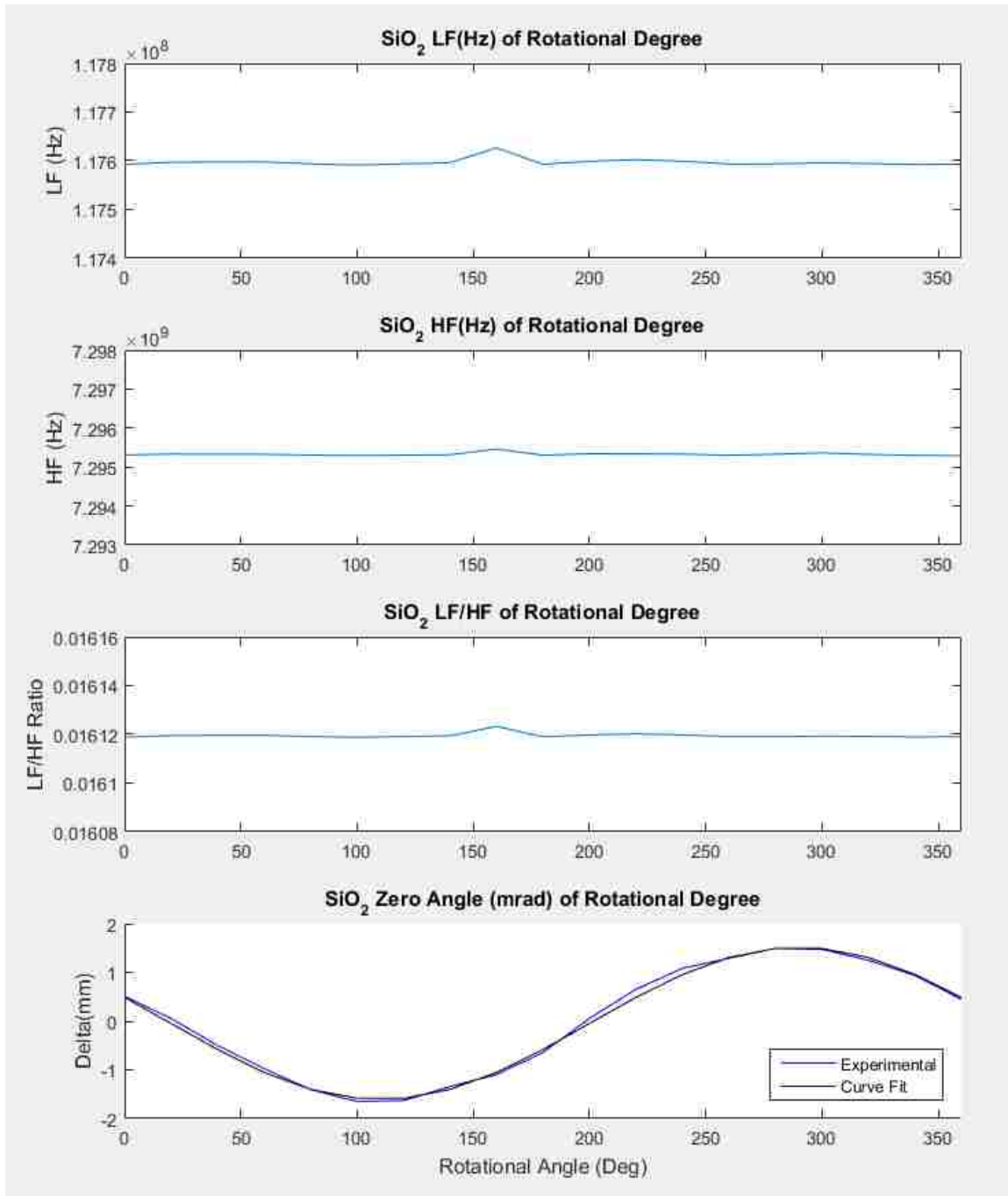
Figure 3.5.17: Plot demonstrating LF, HF, ratio, and zero angle data for the rotational experiment with SiO 2 .
