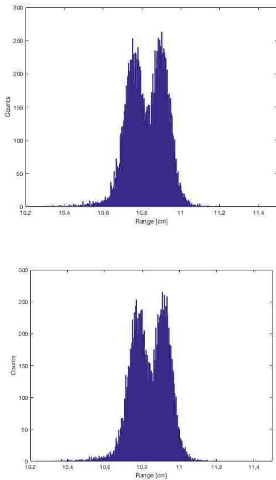
Figure 53 – ^{252}\text{Cf} fission fragment range distributions found with extracted drift velocities of 4.4 \times 10^6 cm/s (top) and 4.3 \times 10^6 cm/s (bottom)
