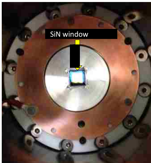
Figure 24 – SiN window
