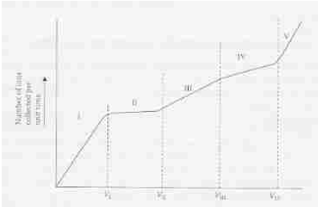
Figure 11 – Gas detector operation regions for applied voltage (x-axis) and number of ions collected per unit time (y-axis) [Tsoulfanidis 2015]
