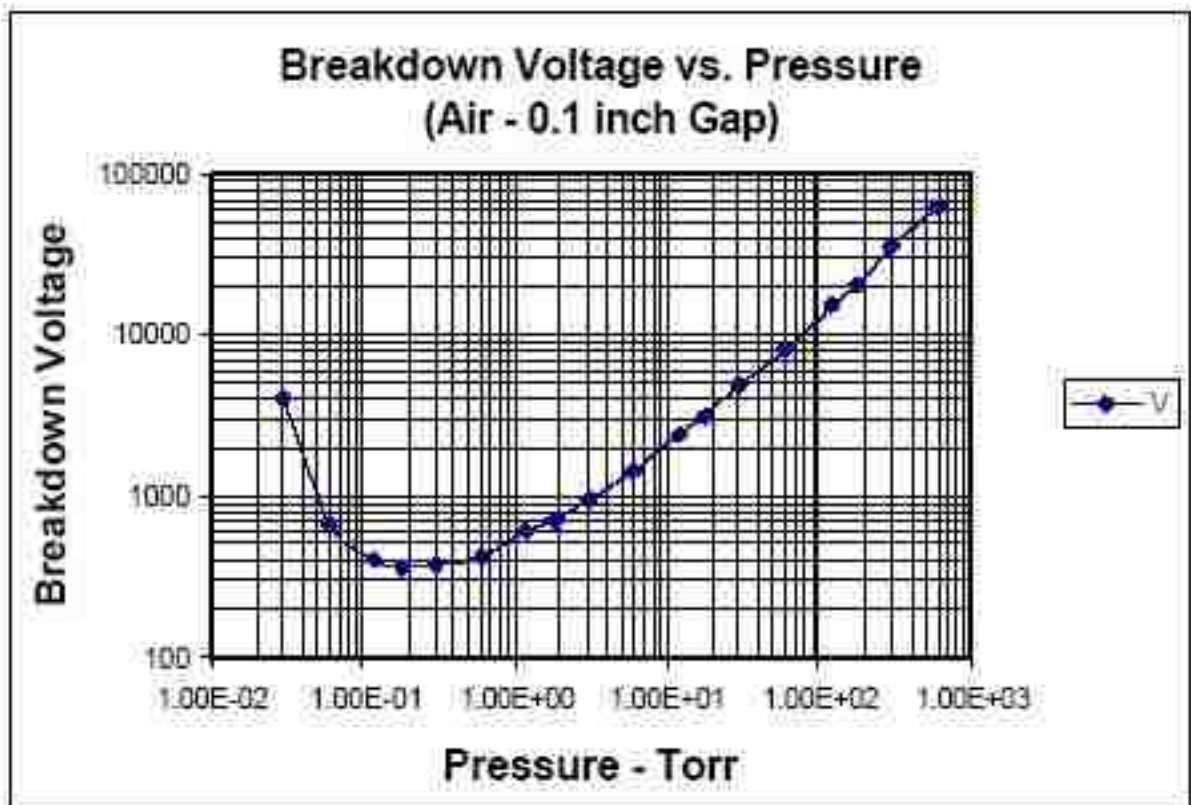
Figure 59 – Breakdown voltage vs. pressure [High Voltage Connection 2016]
