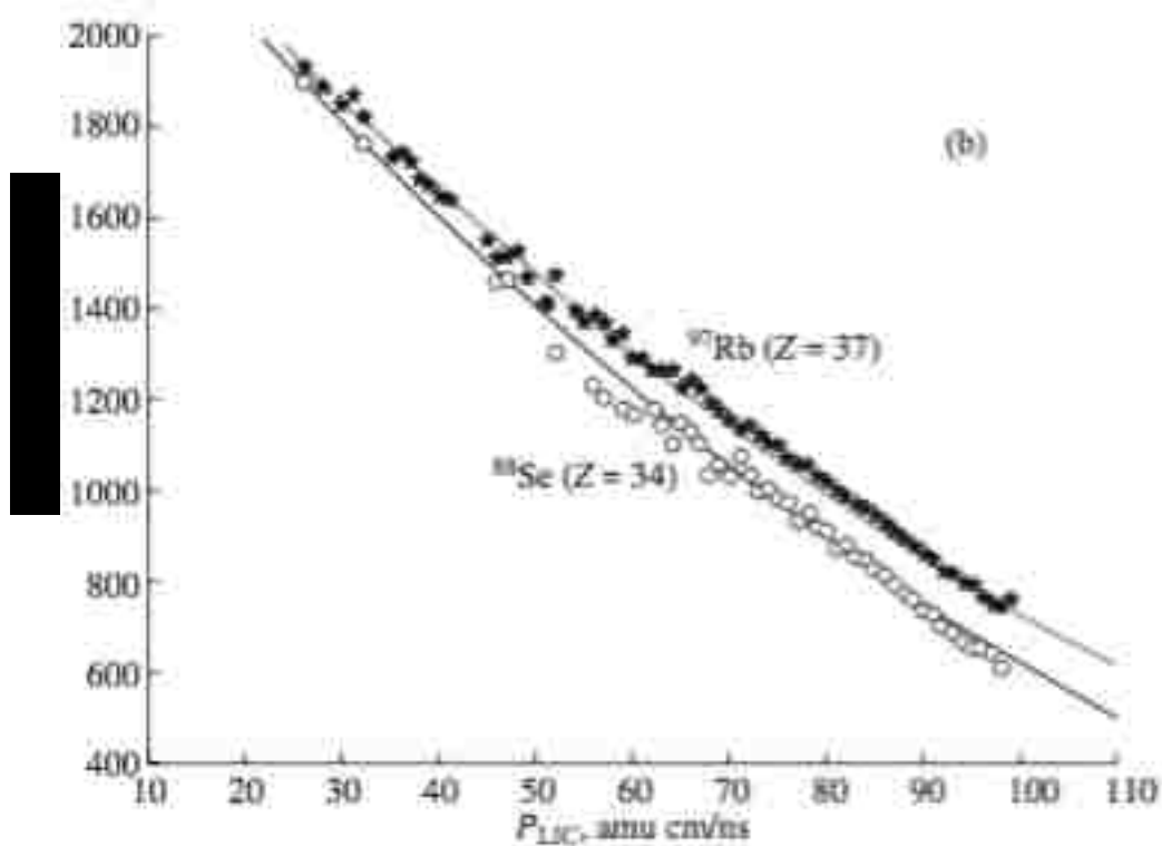
Figure 19 – Atomic charge based on Tyukavkin method for theoretical model and experimental data for ^{97}\text{Rb} and ^{88}\text{Se} [Tyukavkin 2008]
