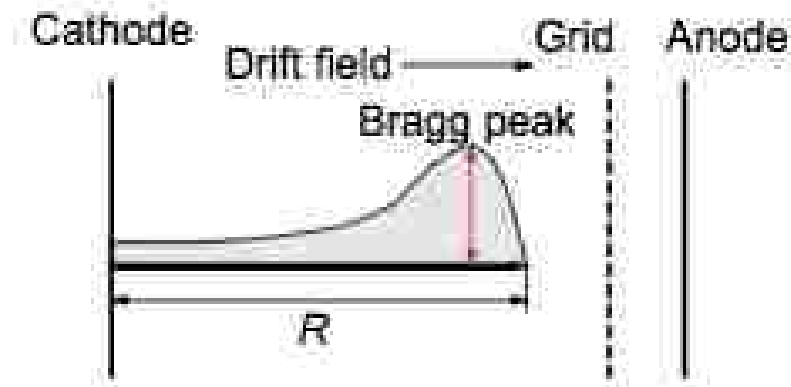
Figure 16 – Model of a Bragg curve within a gridded ionization chamber [Sanami 2009]
