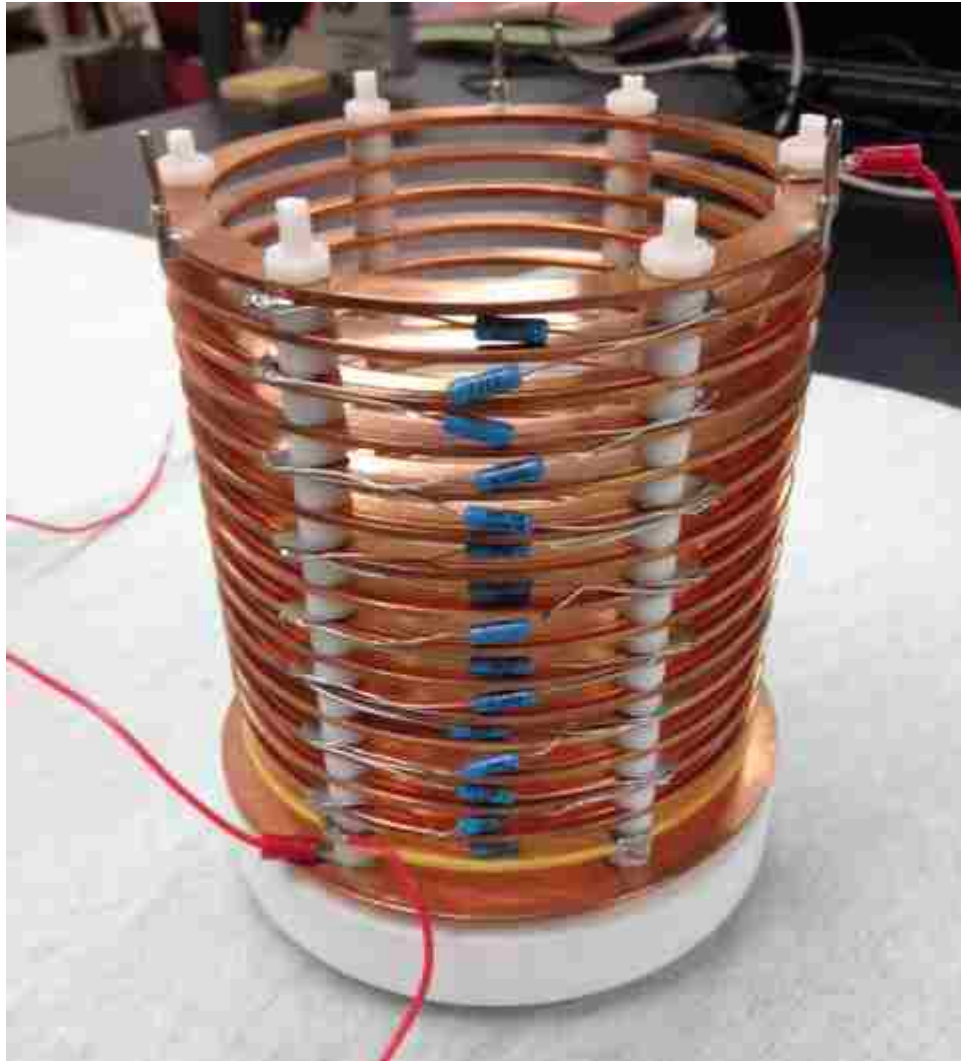
Figure 21 – Ionization chamber
