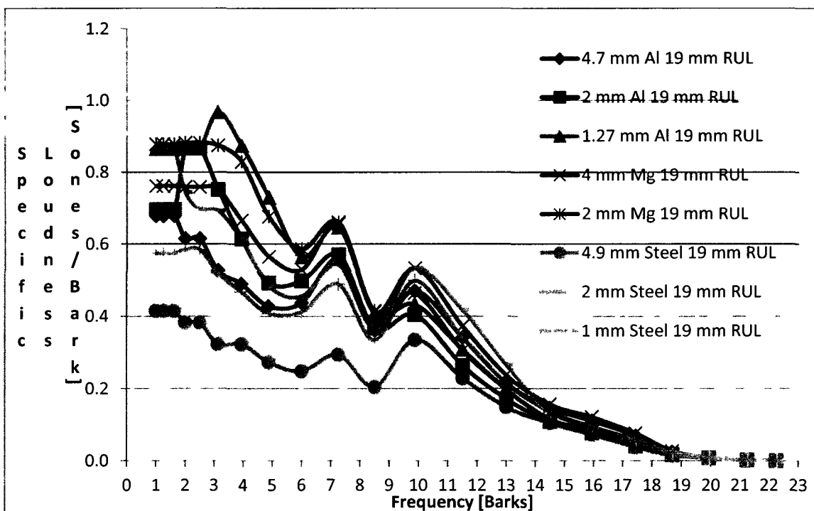
Figure 41: Averaged Specific Loudness for a Free Field Sound Field Condition from Microphones 6 and 10 for the Eight Different Metal Thicknesses of AZ31B Magnesium, 6061-T6 Aluminum and 1018 Cold-Rolled Steel with the 19 mm Thick, 60cmX60cm Sample of RUL Automotive Underpad with Diesel Generator Noise 10 Seconds Signal Duration
