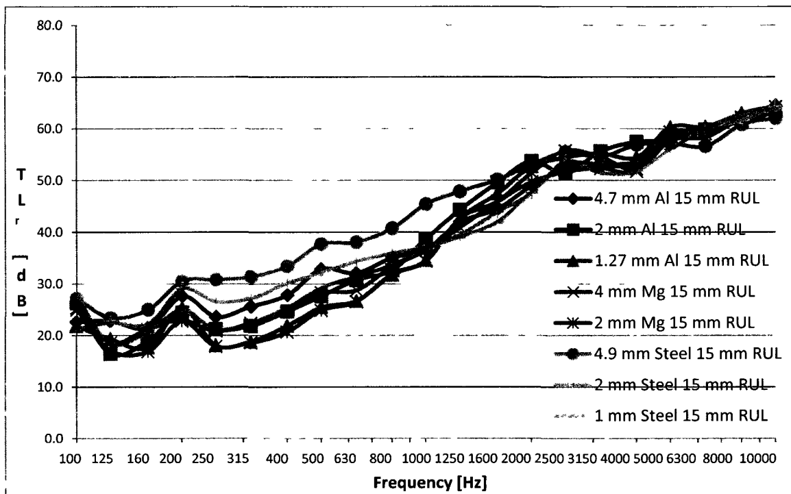
Figure 30: Electric Motor Noise TL r Results of All Material 60cmX60cm Samples with the 15 mm Thick, 60cmX60cm Sample of RUL Automotive Underpad from the Tests in Canton, Michigan
