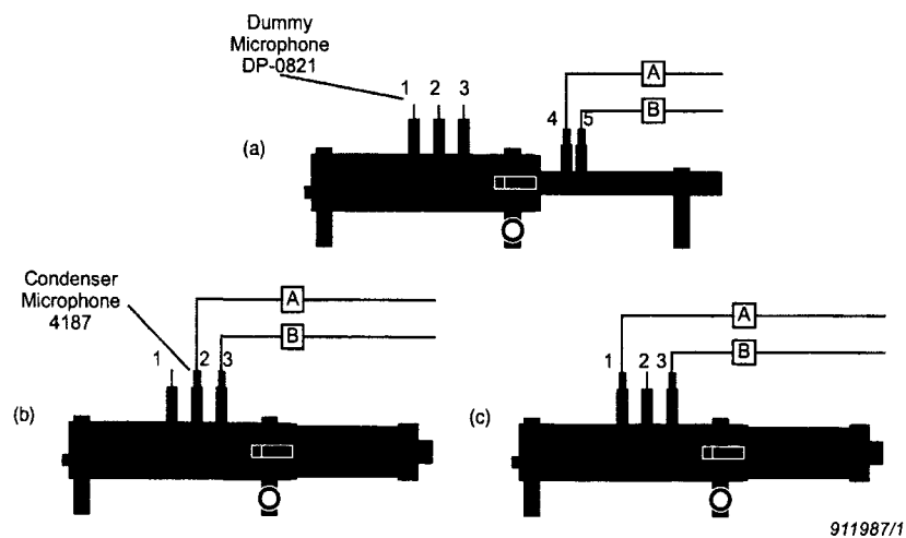
Figure 9: The Tube Setups for Type 4206: a) Standard High Frequency Tube; b) Standard Low Frequency Tube; c) Wide Spacing Low Frequency Tube (Bruel & Kjaer Impedance/Transmission Loss Measurement Tubes Type 4206 Technical Committee, 2007)
