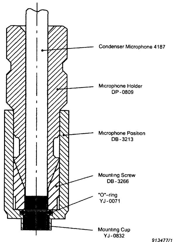
Figure 7: The Internal Structure of a Microphone's Position and Holder (Bruel & Kjaer Impedance/Transmission Loss Measurement Tubes Type 4206 Technical Committee, 2007)
