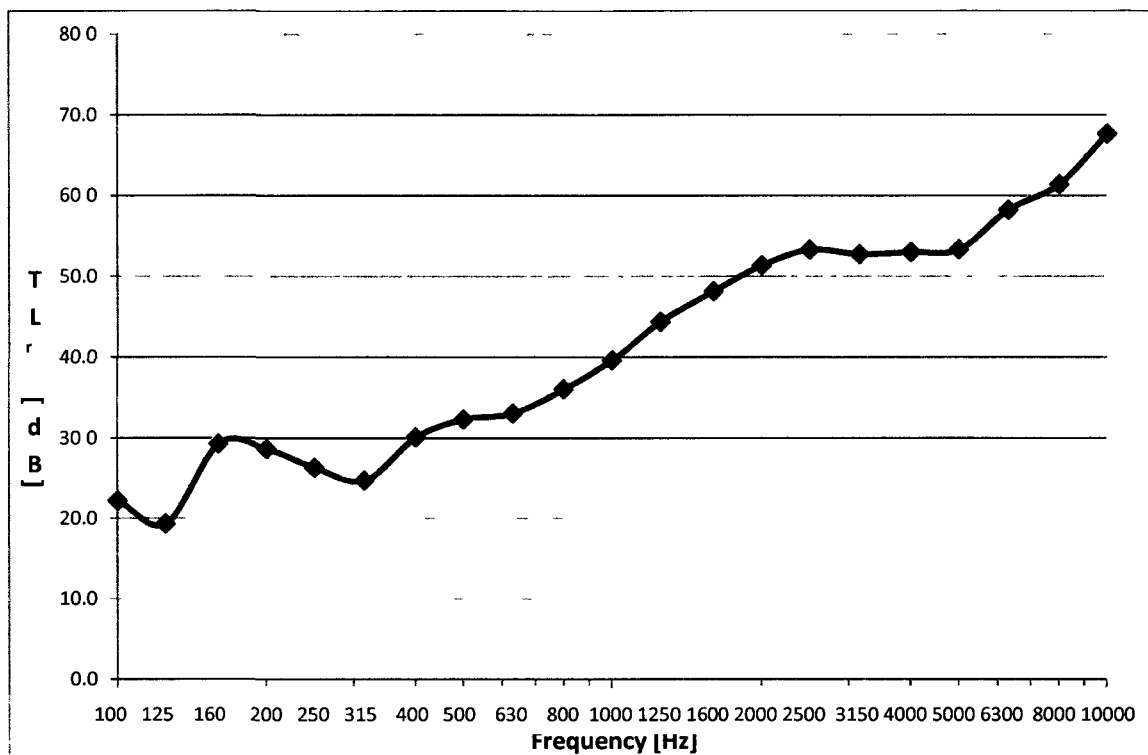
Figure 69: The 2 mm Thick, 60cmX60cm 1018 Cold-Rolled Steel Sample with the 19 mm Thick, 60cmX60cm Sample of RUL Automotive Underpad TL Random Incidence from the J1400 Test in Canton, Michigan
