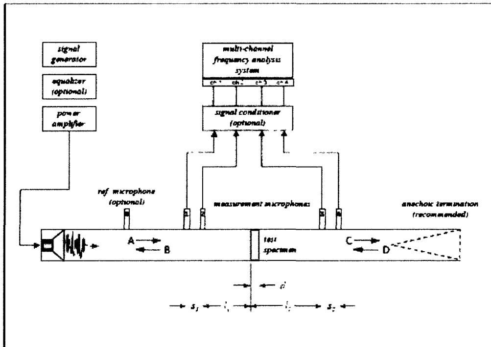
Figure 3: Schematic Drawing of the Measurement Setup (ASTM E2611 Technical Committee, 2009)
