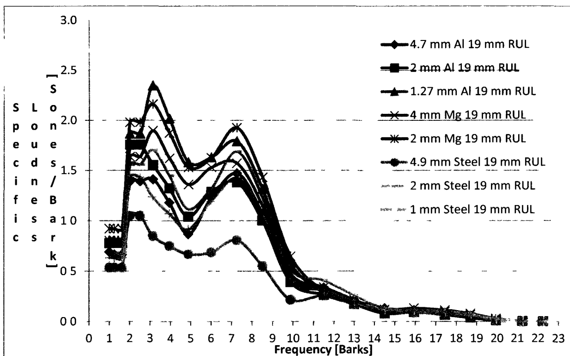
Figure 44: Averaged Specific Loudness for a Free Field Sound Field Condition from Microphones 6 and 10 for the Eight Different Metal Thicknesses of AZ31B Magnesium, 6061-T6 Aluminum and 1018 Cold-Rolled Steel with the 19 mm Thick, 60cmX60cm Sample of RUL Automotive Underpad with Electric Motor Noise 10 Seconds Signal Duration
