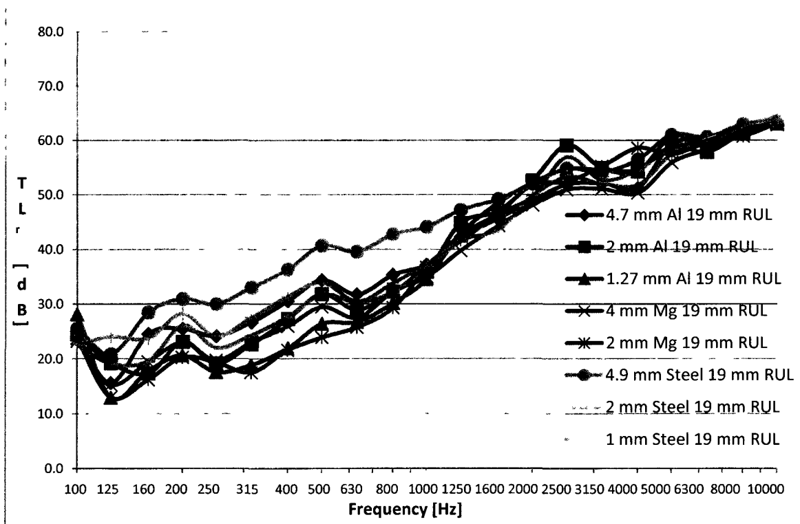
Figure 31: Electric Motor Noise TL r Results of All Material 60cmX60cm Samples with the 19 mm Thick, 60cmX60cm Sample of RUL Automotive Underpad from the Tests in Canton, Michigan
