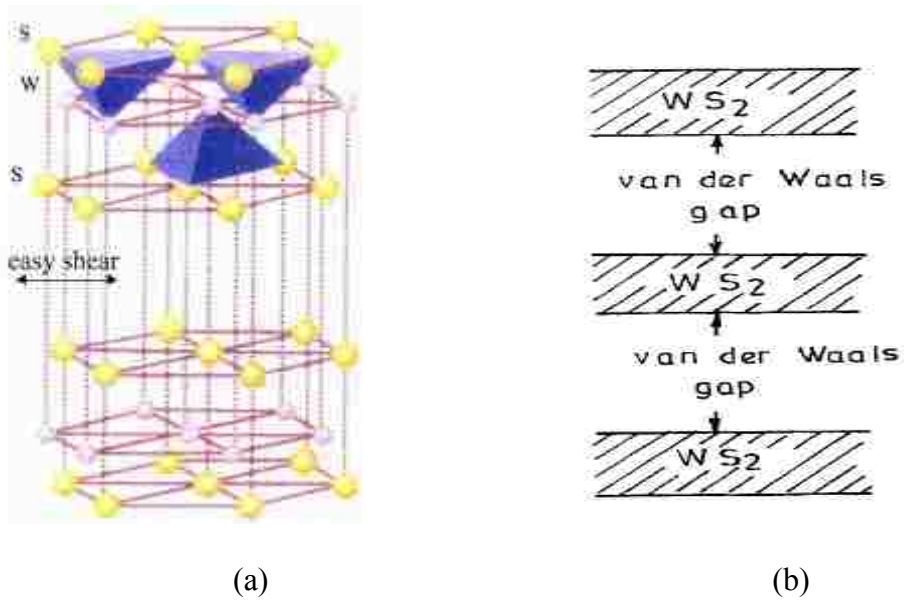
Figure 7 (a) Crystal structure of hexagonal 2H- \text{WS}_2 with easy shear direction [82], (b) structure showing stacking of layers [84]
