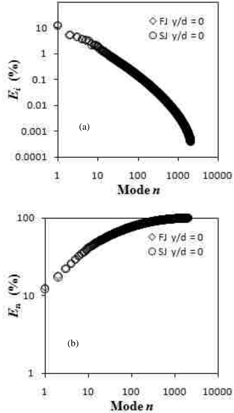
Figure 4.18 POD energy distributions in the horizontal central planes at 42 \leq x/d \leq 62 (a) Fractional contribution of each POD mode to the total energy, E_i . (b) Cumulative energy distribution, E_n .
