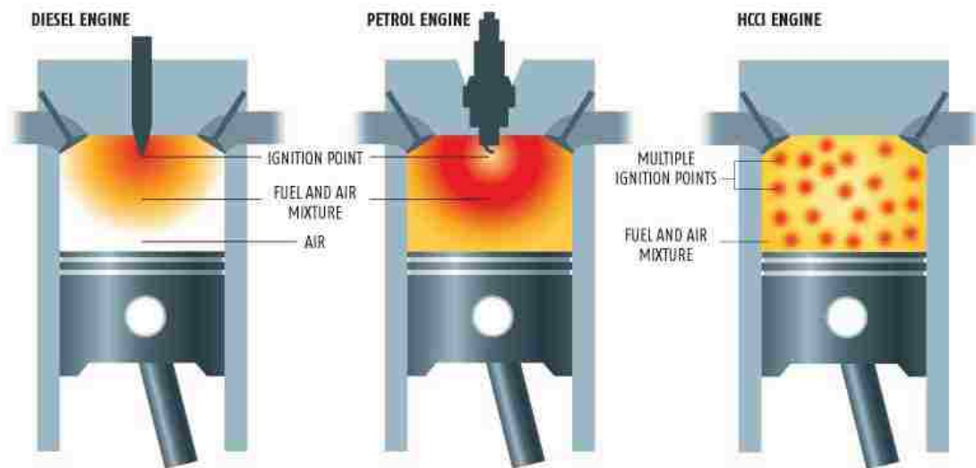
Figure 1.1: CI, SI & HCCI Pictorial Comparison [4]
