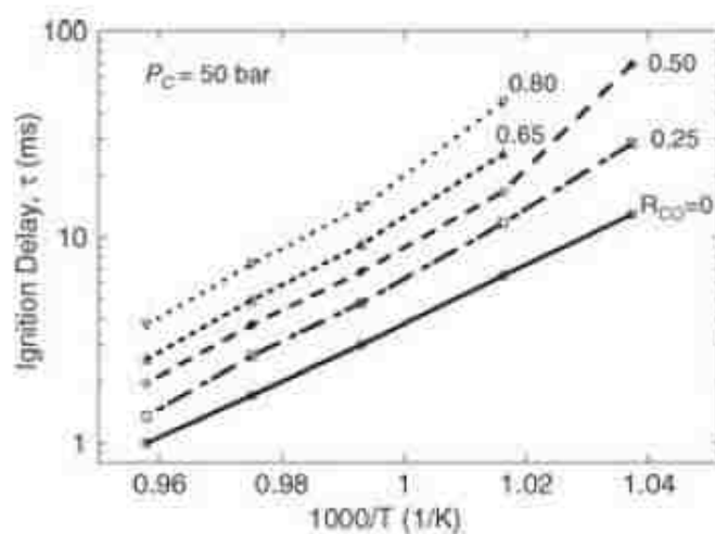
Figure 2.14: Measured ignition delays for H 2 /CO auto-ignition. Molar composition: (H 2 +CO)/O 2 /N 2 /Ar=12.5/6.25/18.125/63.125. Pressure at TDC, P c =50bar [51]
