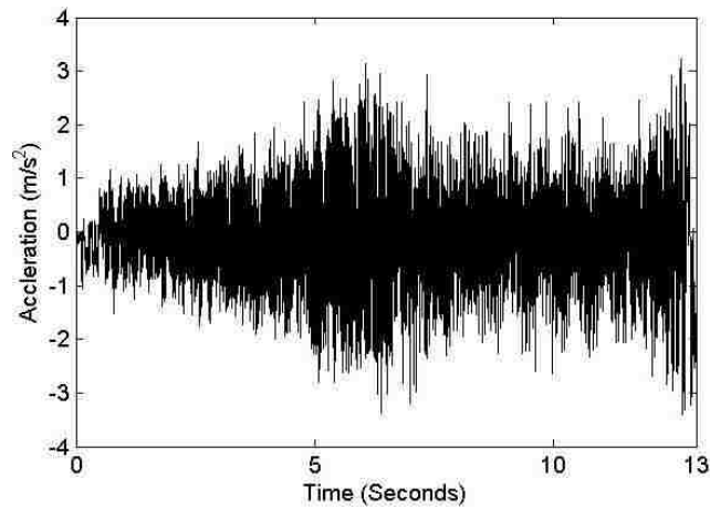
Figure 4-5: Turbine response to yaw motion. Obtained from accelerometer mounted at 50m. Acceleration ( \text{m/s}^2 ) vs. Time (seconds).
