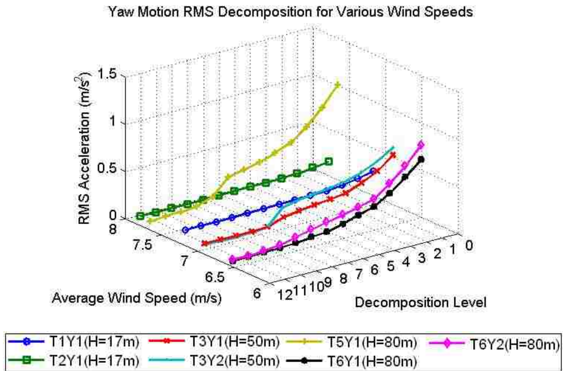
Figure 3-9. Mean Wind Speed (m/s), RMS (m/s 2 ), Decomposition Level Relationship.
