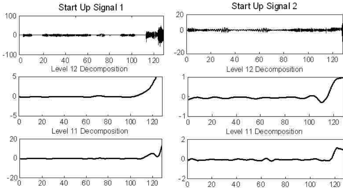
Figure 2-5: Start up raw vibration signals with level 12 and Level 11 decompositions. Signal Amplitude ( \text{m/s}^2 ) vs. Time (seconds).
