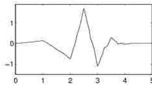
Figure 2-1: Daubachies 6 wavelet. Amplitude vs. Length (dimensionless).
