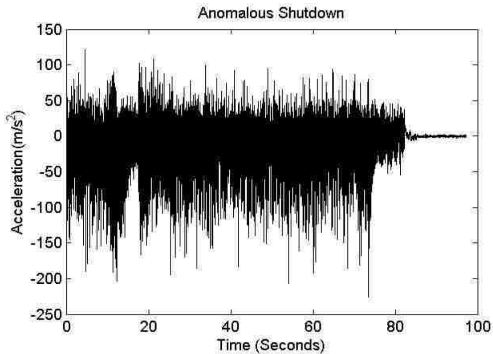
Figure 4-9: Anomalous Shut down signal. Acceleration ( \text{m/s}^2 ) vs. Time (seconds).
