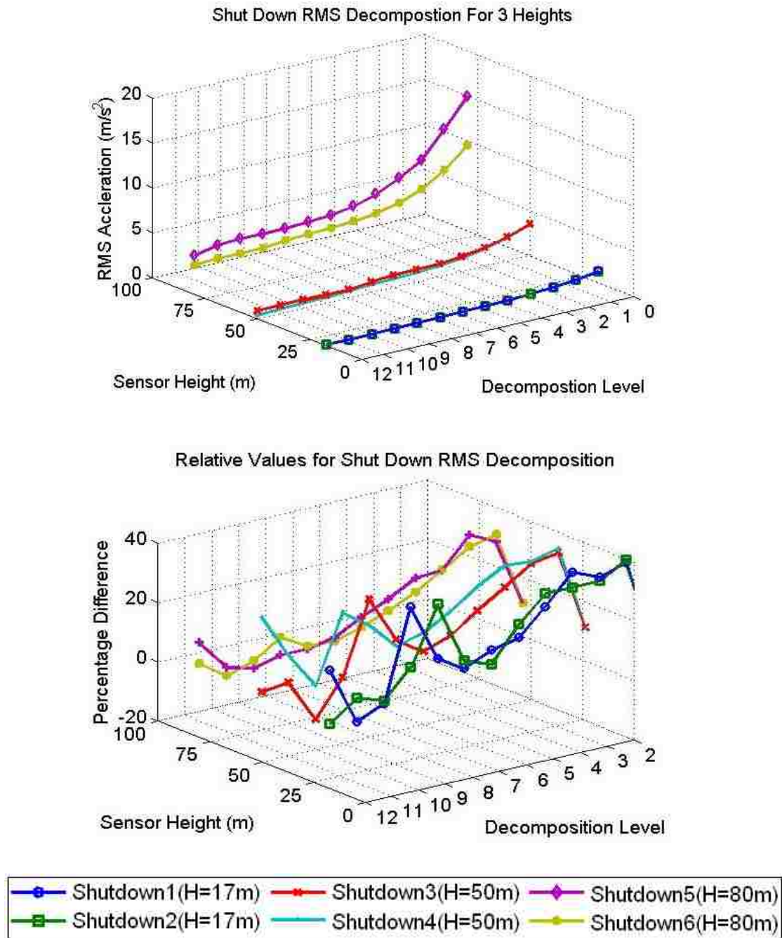
Figure 3-14. Height (m), RMS ( \text{m/s}^2 ), Decomposition Level Relationship for Shutdown. Absolute Values (Top frame), Relative Values (bottom frame).
