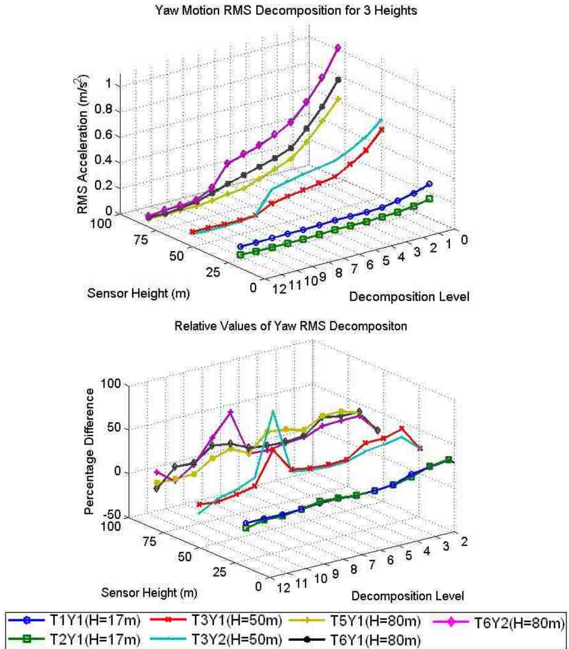
Figure 3-8. Yaw Motion RMS Decomposition for 3 Heights. Height (m), RMS ( \text{m/s}^2 ), Absolute and Relative values.
