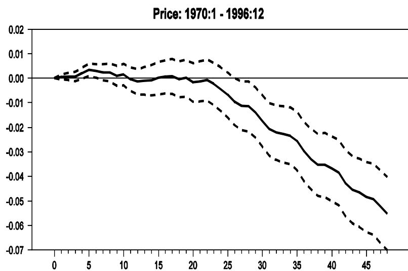
Figure 3.12 – Impulse Response Functions: Carter Credit Controls Specification
