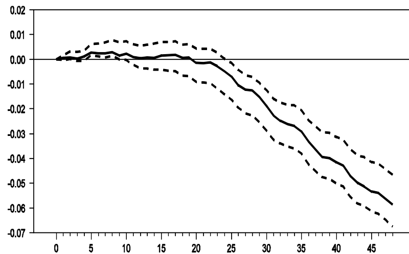
Price - 1996 IRF in 2003 S.C. Corrected CI
