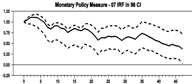
Figure 4.44 – Comparison of ALFRED / BCI / SPF VAR IRF's
