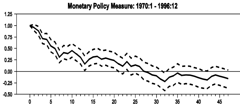
Figure 3.9 – VAR Impulse Response Functions: Chairmen Specification
