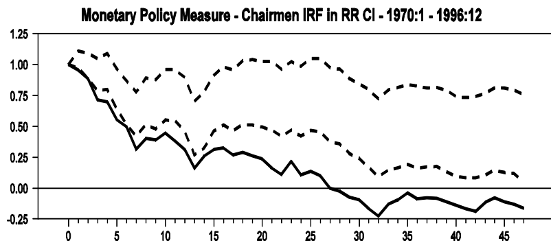
Figure 3.10 – Comparison of Romer-Romer and Chairmen Specification VAR IRF's
