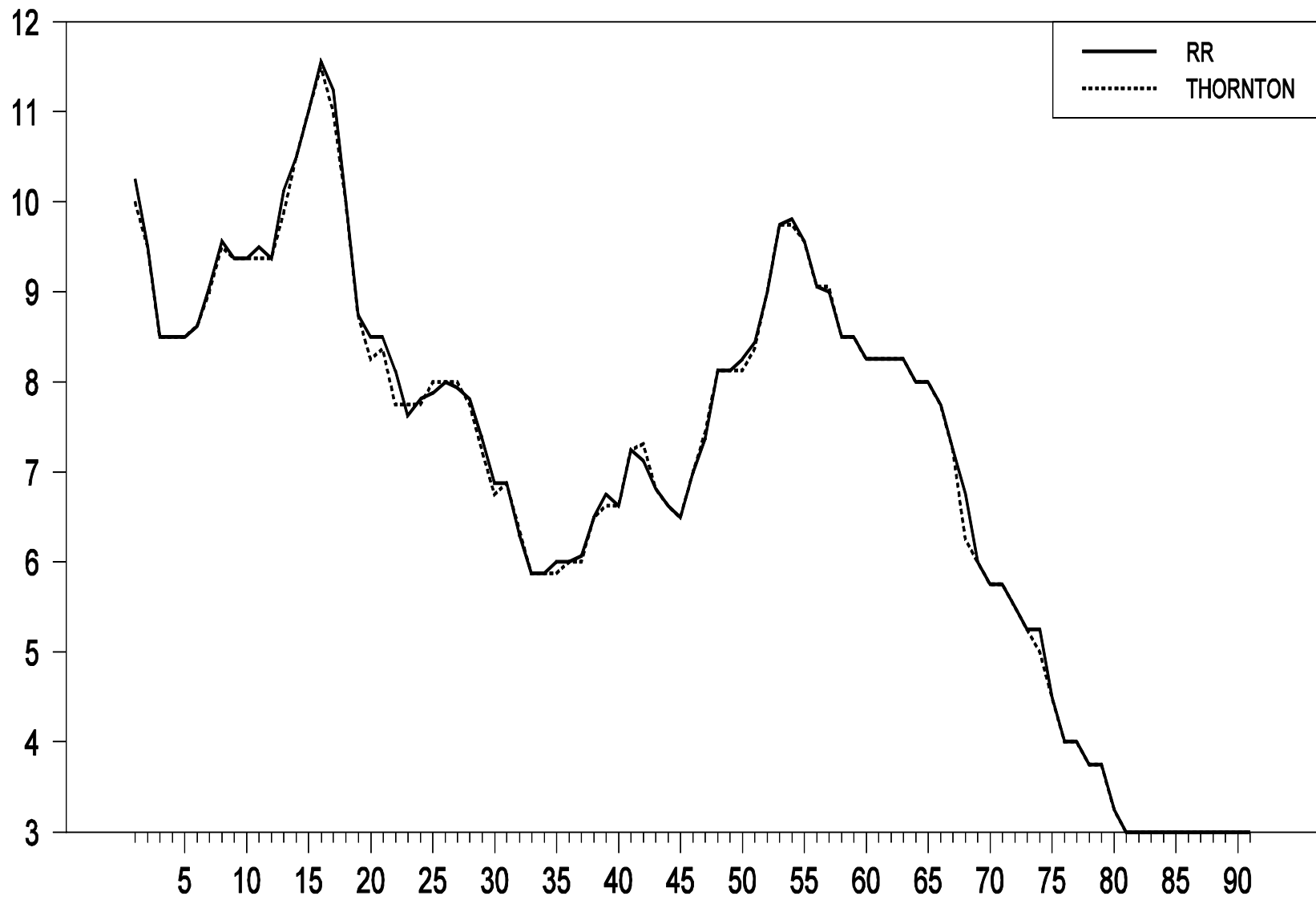
Figure 2.8 – Comparison of RR and Thornton Level of the Intended Funds Rate Prior to Meeting
