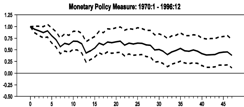
Figure 4.8 – VAR Impulse Response Functions: RR / BCI Specification
