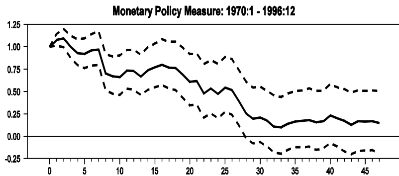
Figure 3.4 - VAR Impulse Response Functions: Regimes Specification
