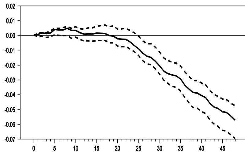
Price - 2003 S.C. Corrected IRF in 1996 CI
