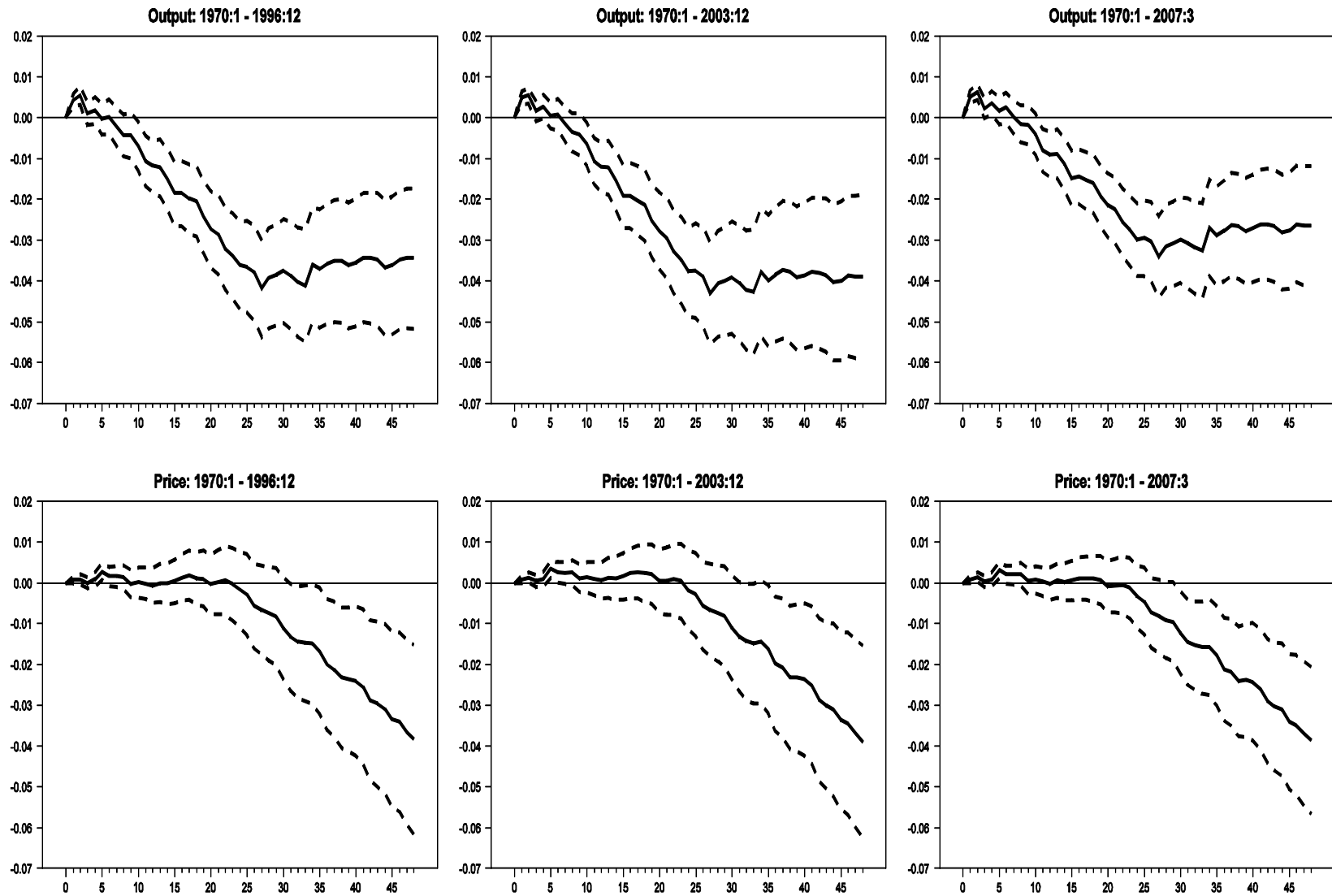
Figure 4.15 – Single Equation Impulse Response Functions: SPF Specification
