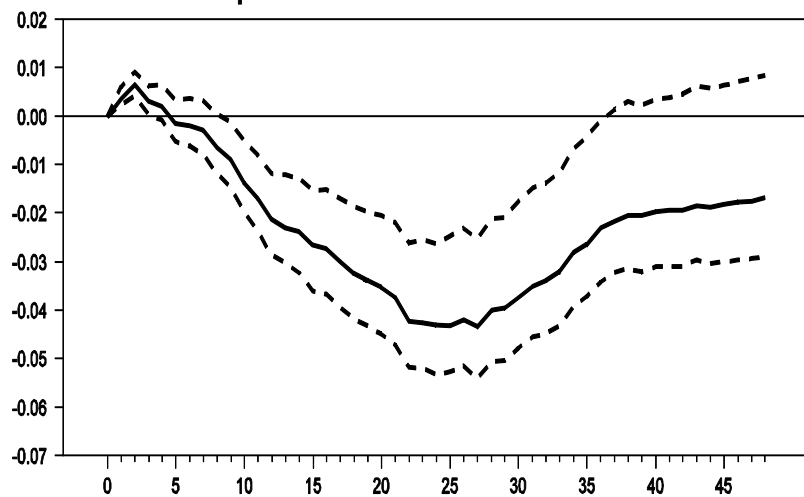
Output - 1996 IRF in 2003 S.C. Corrected CI
