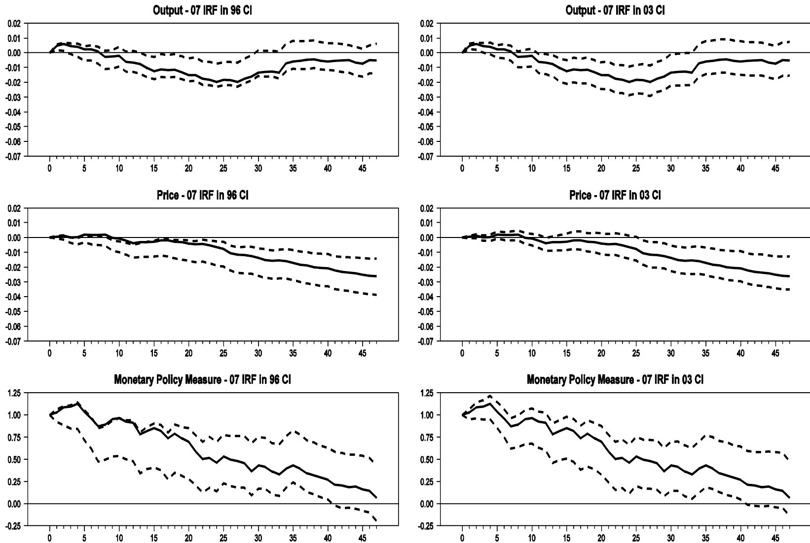
Figure 4.32 – Comparison of BCI Specification VAR IRF's
