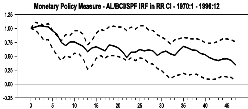
Figure 4.43 – Comparison of Romer-Romer and ALFRED / BCI / SPF VAR IRF's
