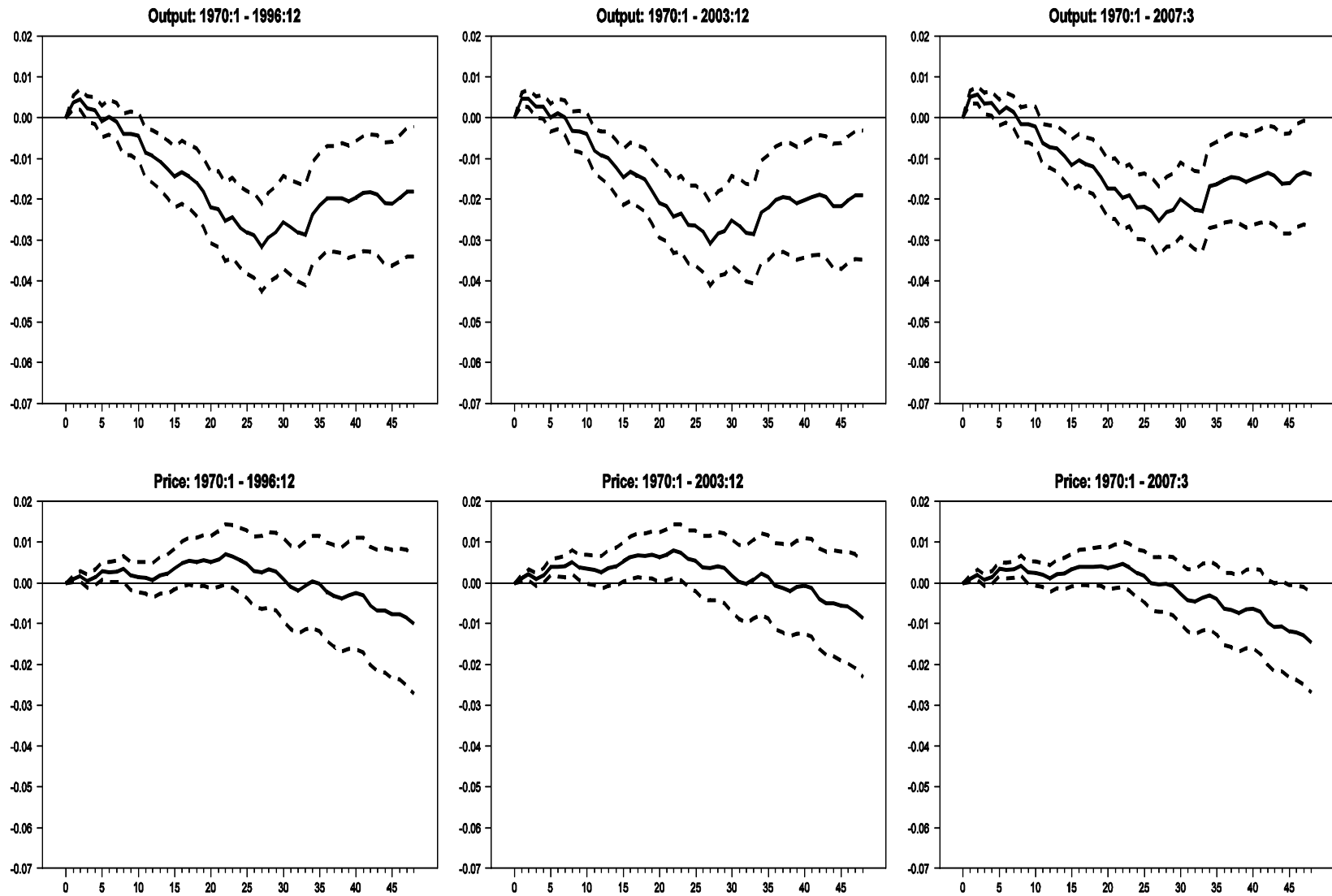
Figure 4.27 – Single Equation Impulse Response Functions: BCI Specification
