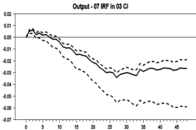
Figure 4.17 – Comparison of SPF Specification Single Equation IRF's
