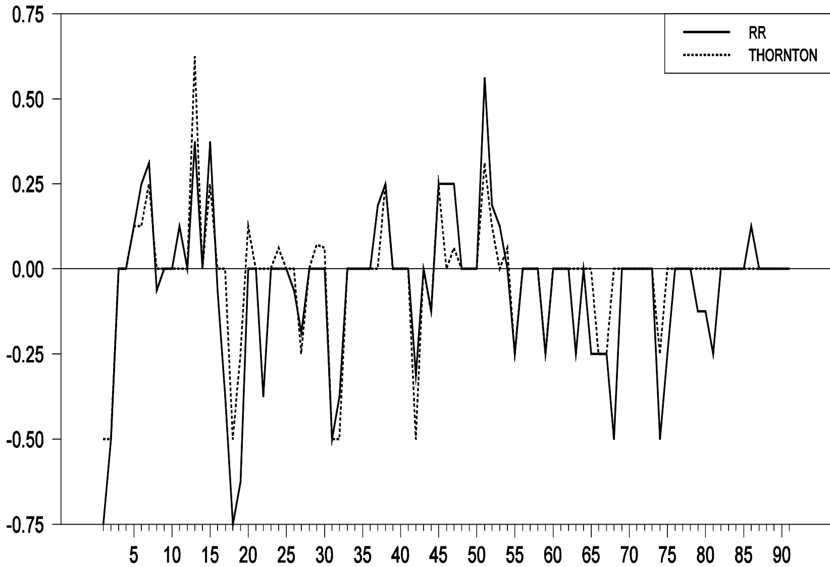
Figure 2.6 – Comparison of RR and Thornton Change in Intended Funds Rate
