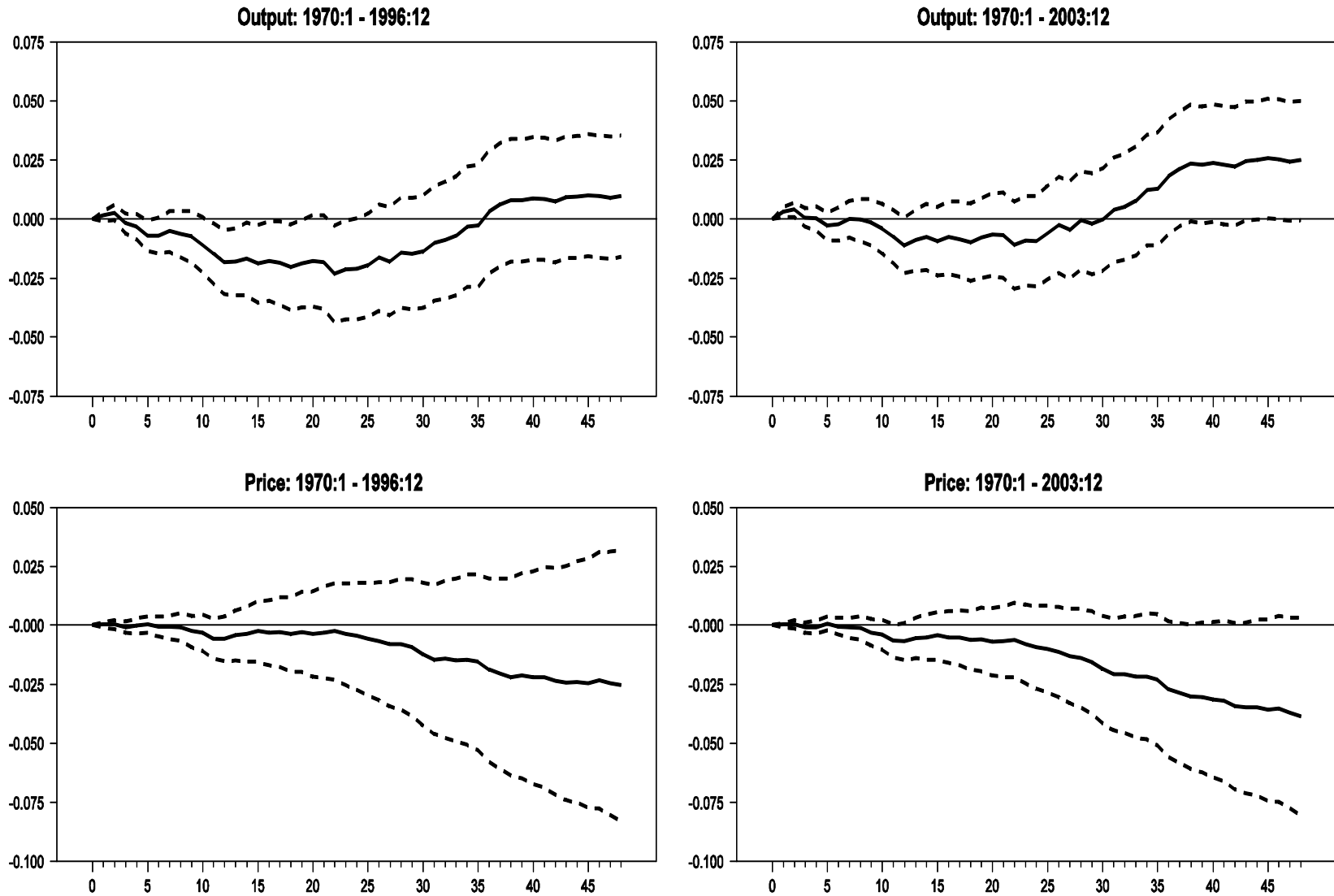
Figure 3.7 – Single Equation Impulse Response Functions: Chairmen Specification
