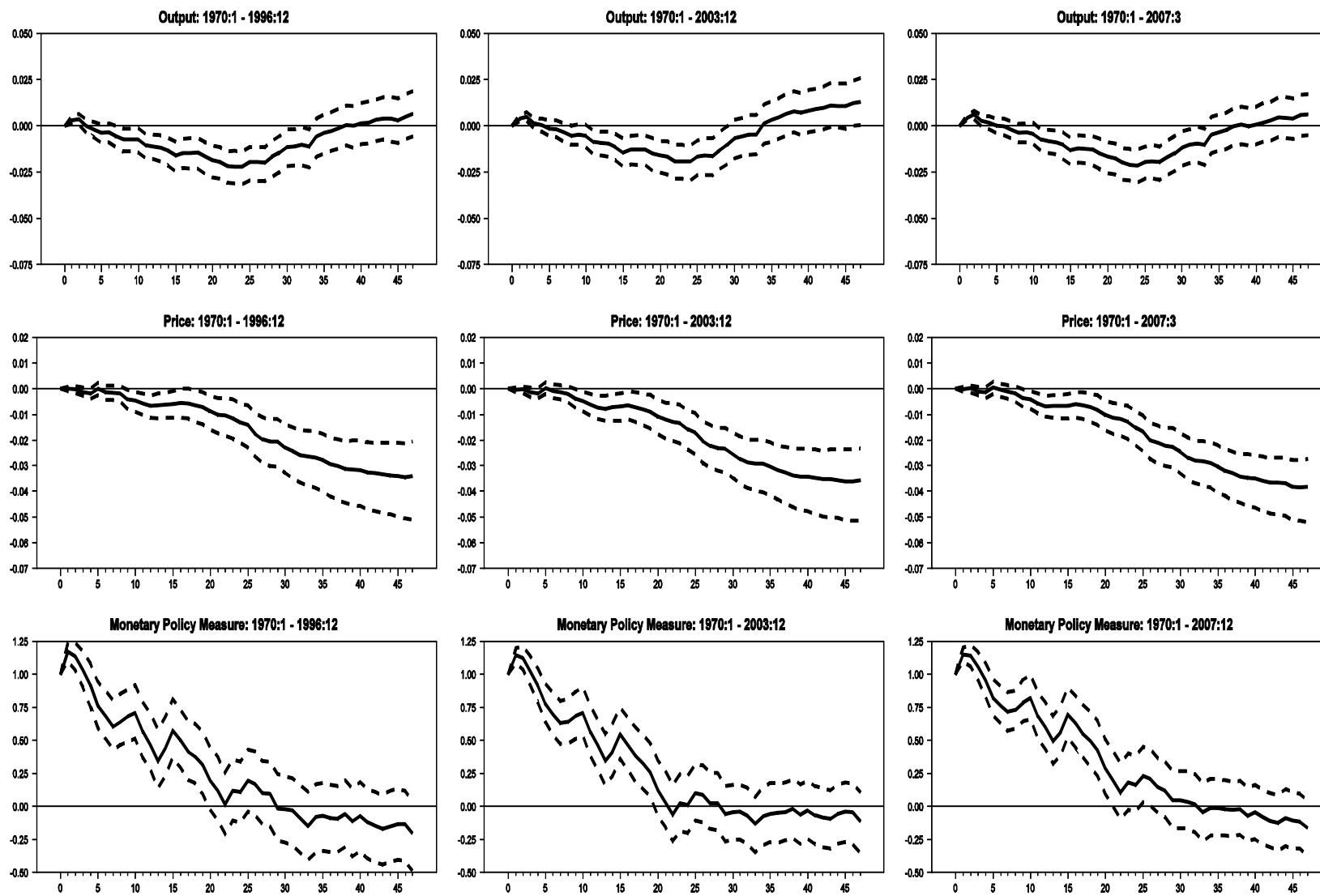
Figure 4.24 – VAR Impulse Response Functions: ALFRED / SPF Specification
