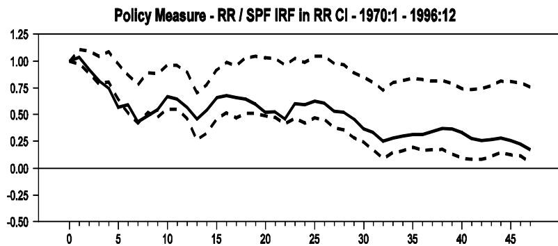
Figure 4.5 – Comparison of Romer-Romer and RR / SPF VAR IRF's
