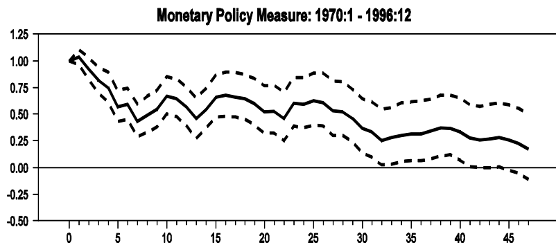
Figure 4.4 – VAR Impulse Response Functions: RR / SPF Specifications
