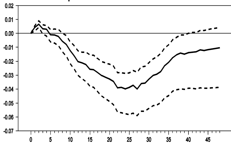
Output - 2003 S.C. Corrected IRF in 1996 CI
