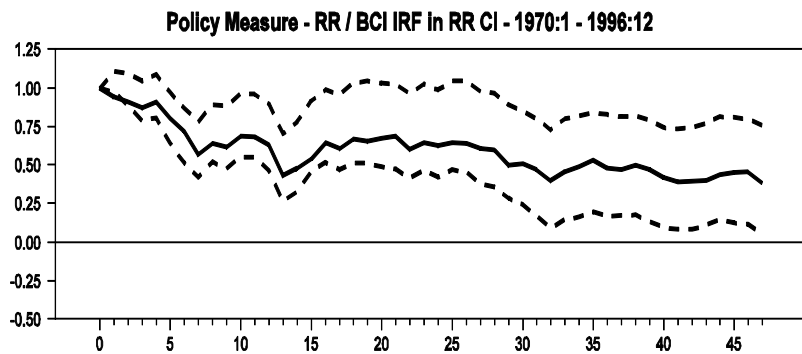
Figure 4.9 – Comparison of Romer-Romer and RR / BCI VAR IRF's
