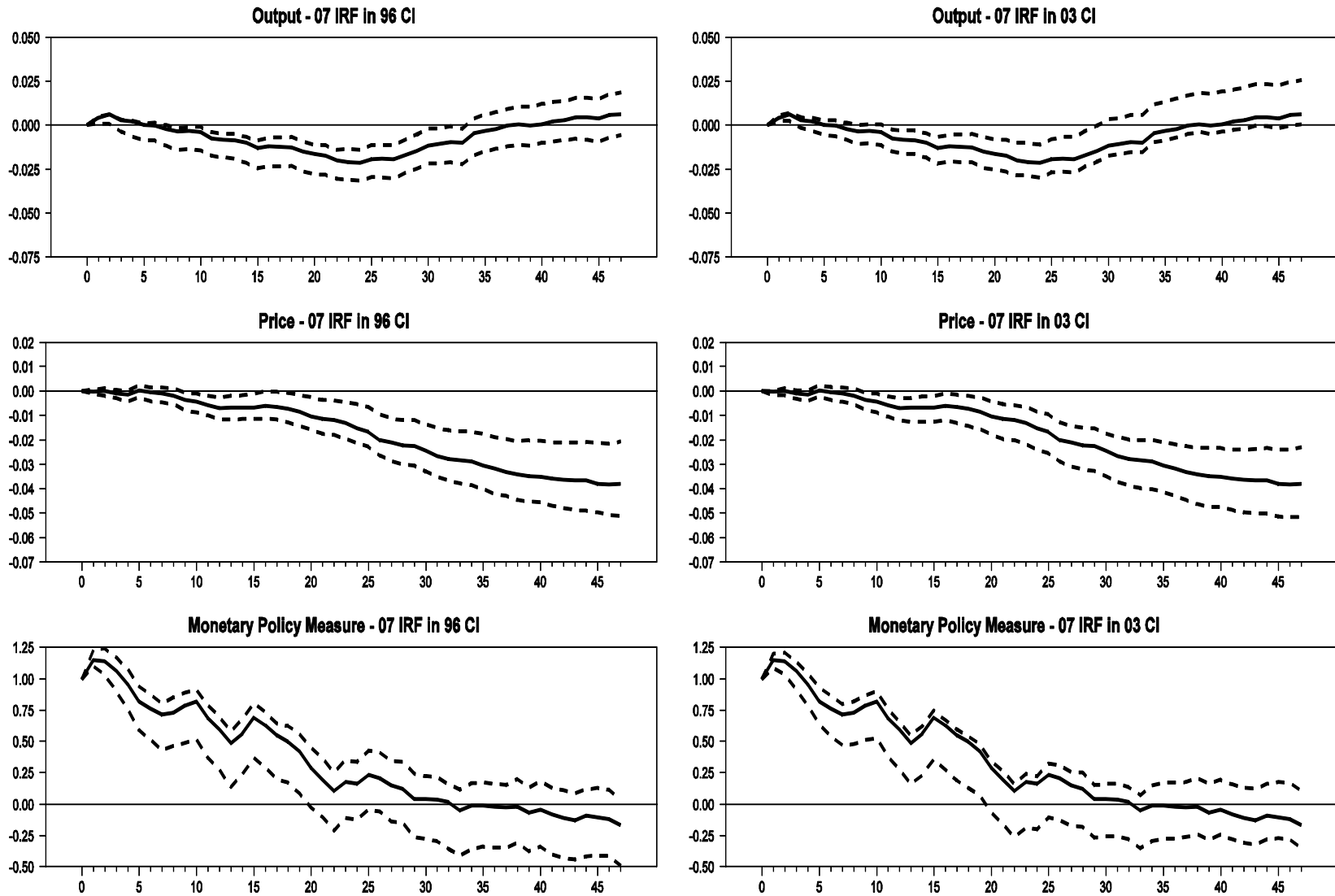
Figure 2.26 – Comparison of ALFRED / SPF Specification VAR IRF's
