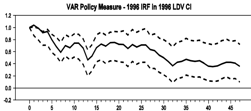
Figure 2.5 – Comparisons of VAR Impulse Response Functions – a
