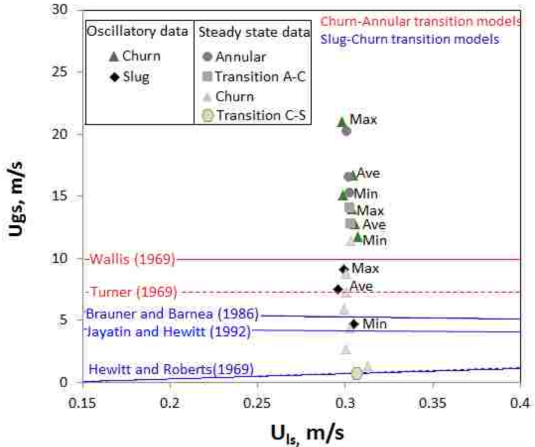
Figure 4.2 Flow regime comparison for steady-state, oscillatory data and transition models at 220 Kpa.
