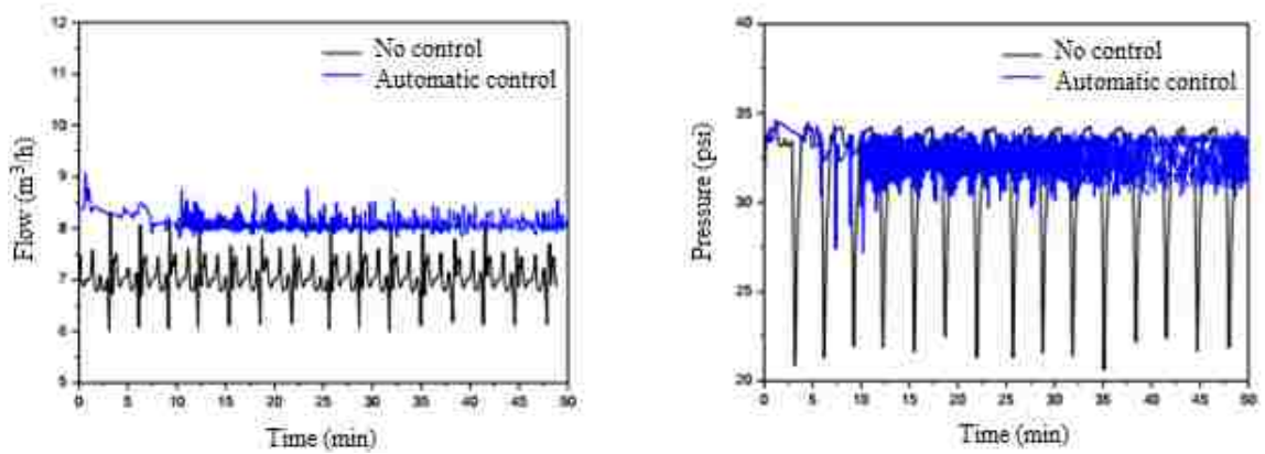
Figure 2.9 The graphs represent the natural and controlled oscillations. The left graph shows the flow rate variation and the right indicates the pressure variation both with respect to time (Silva et al. 2013).
