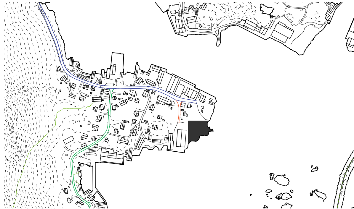
Figure 15: Aerial photograph of Ballstad and accompanying map with 5m contour
