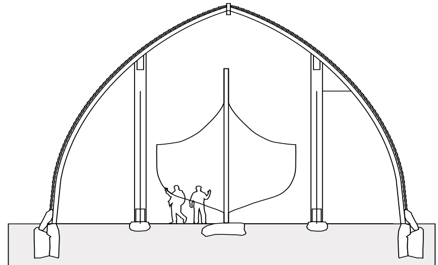
Figure 36: The sectional and structural evolution of the naust
