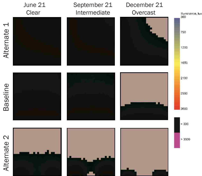
Figure 3.6 Point-in-time Illuminance results.
