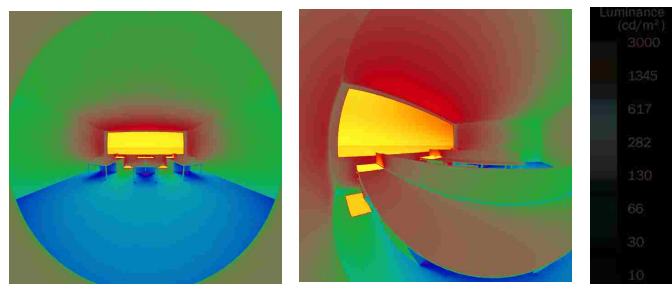
Figure 3.14 Luminance falsecolors from back of space (left) and at desk facing southwest (right) with scale 0-3,000 cd/m 2 .
