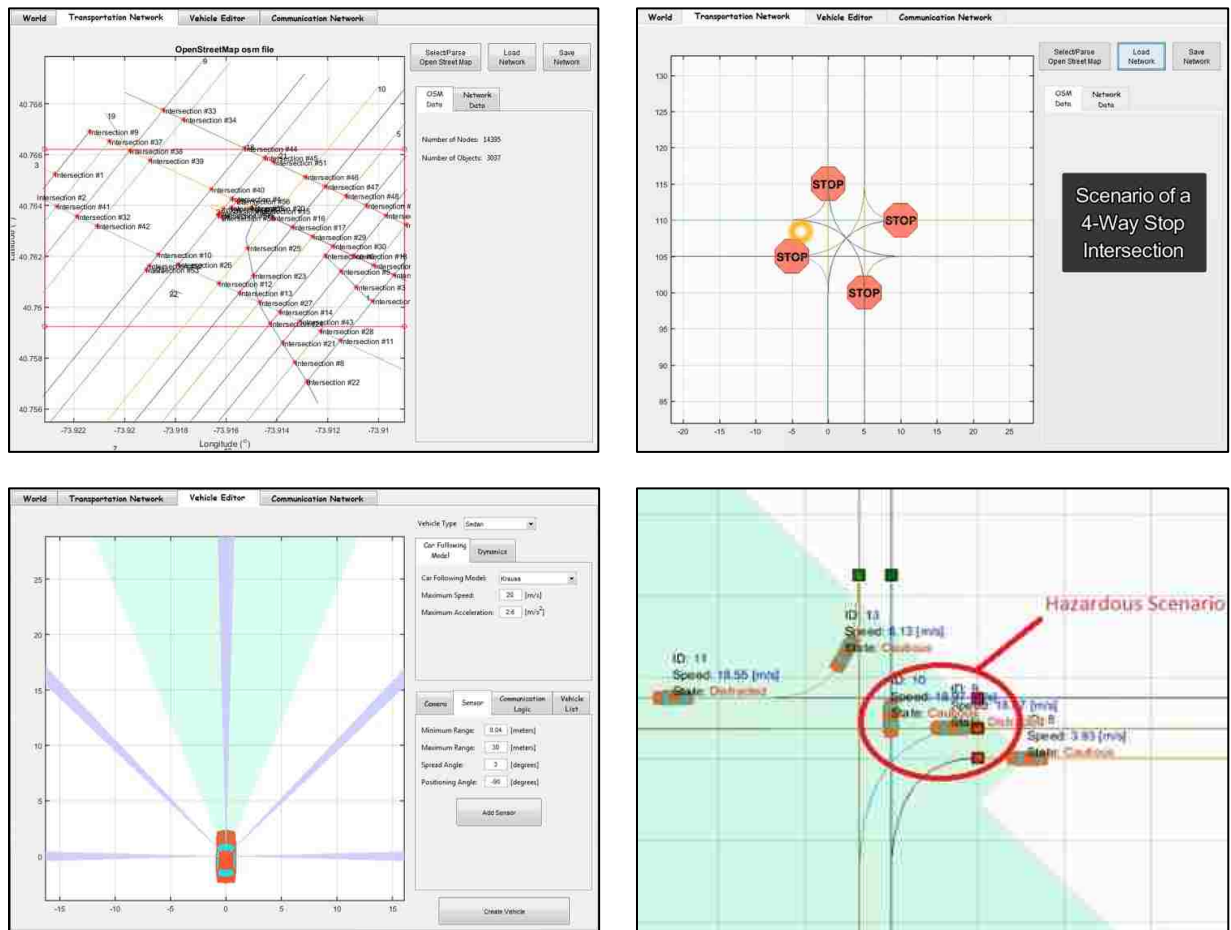
Figure 3: Snapshot of the early prototype of the co-simulator
