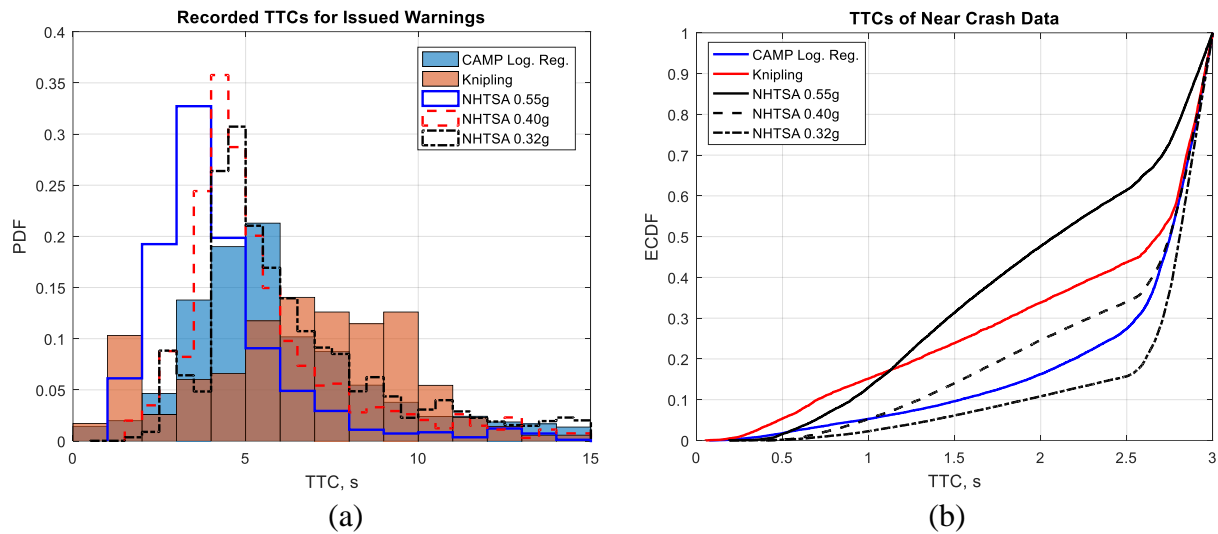
Figure 29: (a) Distribution of TTCs that were recorded when a positive warning was generated (b) ECDF of near-crash data for all recorded TTCs
