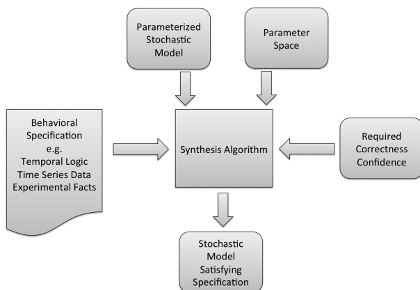
Figure 3.1: Problem description: Given behavioral specifications about the computational model of a system, the parametric stochastic model itself, and a correctness confidence, find the values of the parameters that enable the model to satisfy the specification.
