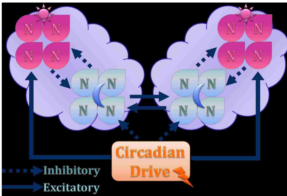
Figure 3.1 – Two-Hemisphere Model
